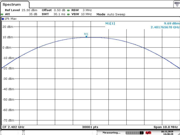
Channel 0 (2402MHz)
