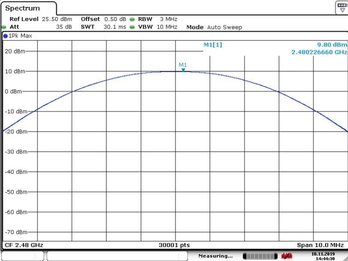
Channel 39 (2480MHz)
