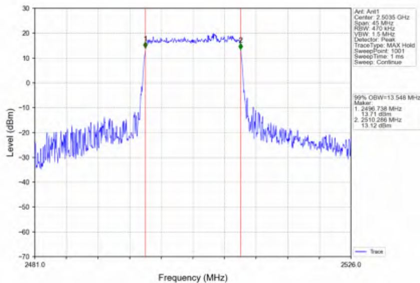
Band41_15MHz_16QAM_LCH_2503.5MHz_RB_75_0_NTNV
