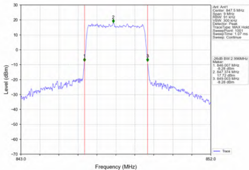
Band26b_3MHz_16QAM_HCH_847.5MHz_RB_15_0_NTNV
