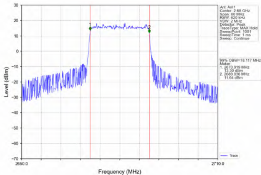
Band41 20MHz 256QAM HCH 2680MHz RB 100 0 NTNV
