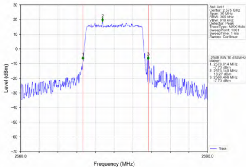
Band38_10MHz_16QAM_LCH_2575MHz_RB_50_0_NTNV
