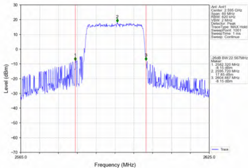
Band38_20MHz_64QAM_MCH_2595MHz_RB_100_0_NTNV
