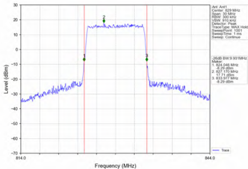
Band26b_10MHz_16QAM_LCH_829MHz_RB_50_0_NTNV
