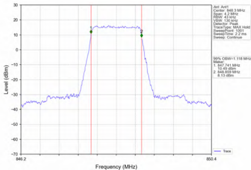
Band26b_1.4MHz_256QAM_HCH_848.3MHz_RB_6_0_NTNV
