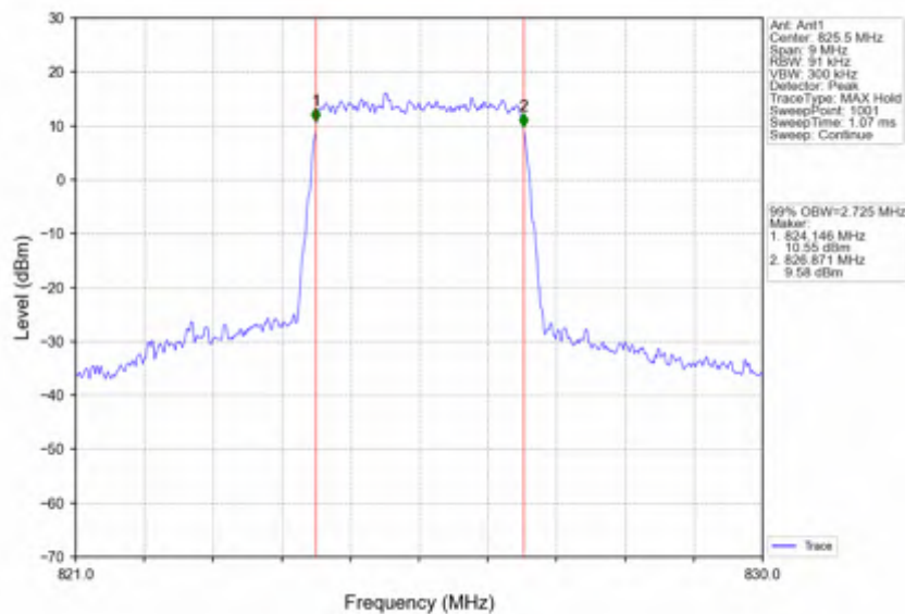
Band26b_3MHz_256QAM_LCH_825.5MHz_RB_15_0_NTNV
