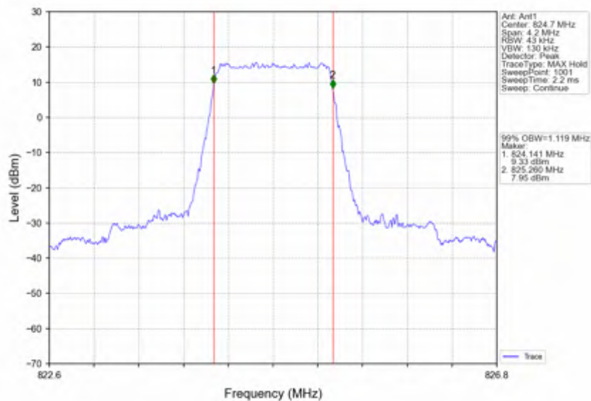
Band26b_1.4MHz_256QAM_LCH_824.7MHz_RB_6_0_NTNV
