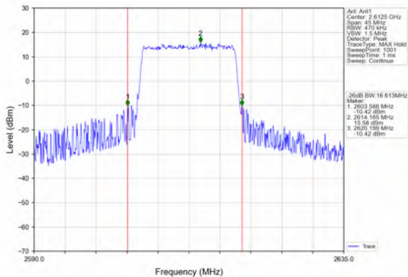
Band38 15MHz 256QAM HCH 2612.5MHz RB 75 0 NTNv
