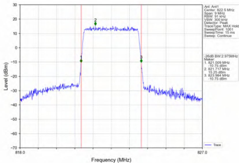
Band26a_3MHz_16QAM_HCH_822.5MHz_RB_15_0_NTNV
