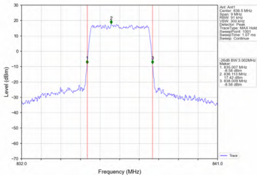
Band26b_3MHz_64QAM_MCH_836.5MHz_RB_15_0_NTNV
