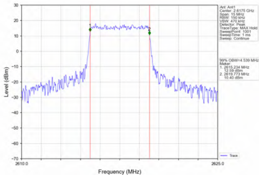
Band38_5MHz_16QAM_HCH_2617.5MHz_RB_25_0_NTNV
