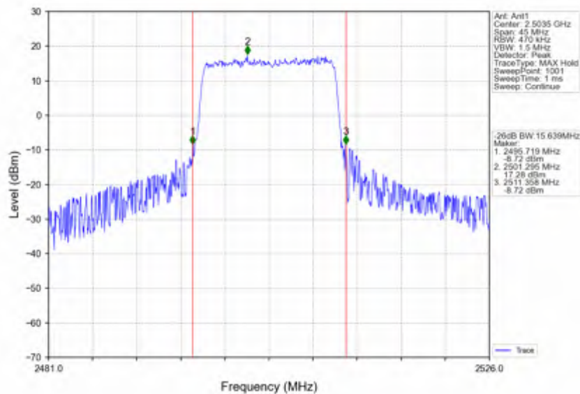
Band41_15MHz_256QAM_LCH_2503.5MHz_RB_75_0_NTNV
