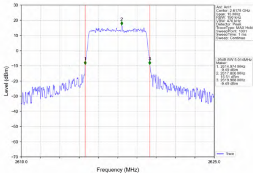
Band38_5MHz_256QAM_HCH_2617.5MHz_RB_25_0_NTNV
