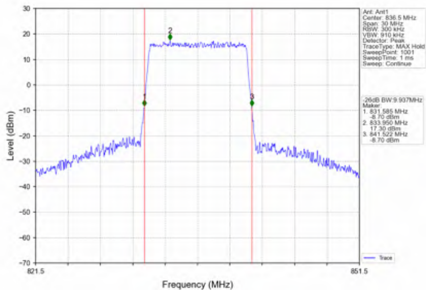
Band26b_10MHz_QPSK_MCH_836.5MHz_RB_50_0_NTNV
