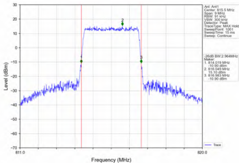
Band26a_3MHz_16QAM_LCH_815.5MHz_RB_15_0_NTNV
