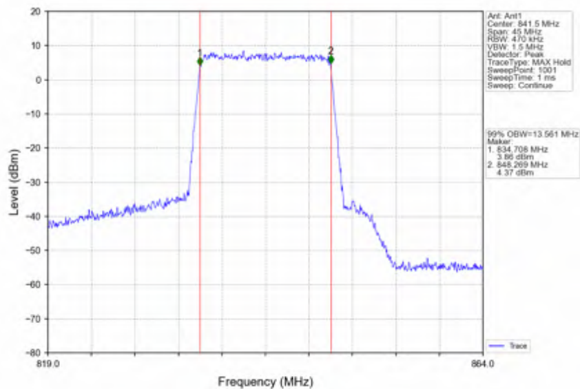
Band26c_15MHz_256QAM_HCH_841.5MHz_RB_75_0_NTNV
