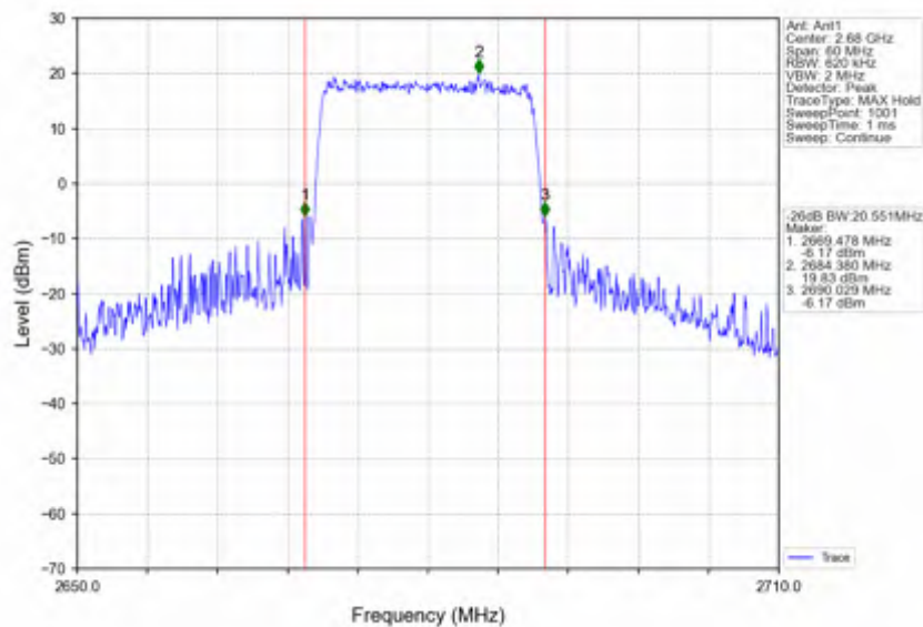
Band41_20MHz_16QAM_HCH_2680MHz_RB_100_0_NTNV
