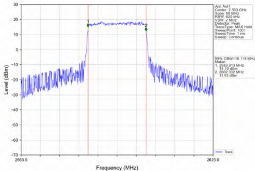
Band41_20MHz_64QAM_MCH_2593MHz_RB_100_0_NTNV
