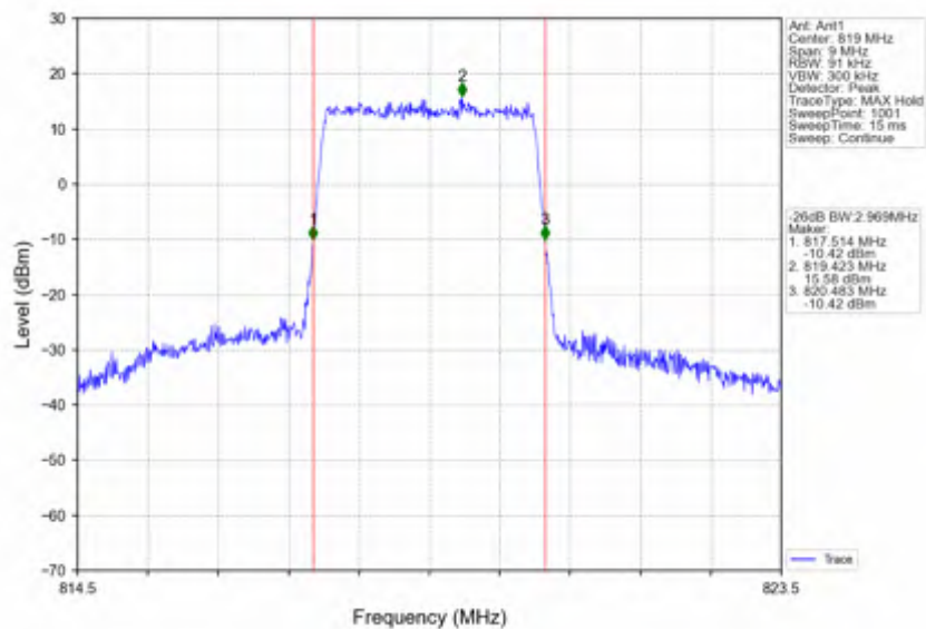
Band26a_3MHz_QPSK_MCH_819MHz_RB_15_0_NTNV
