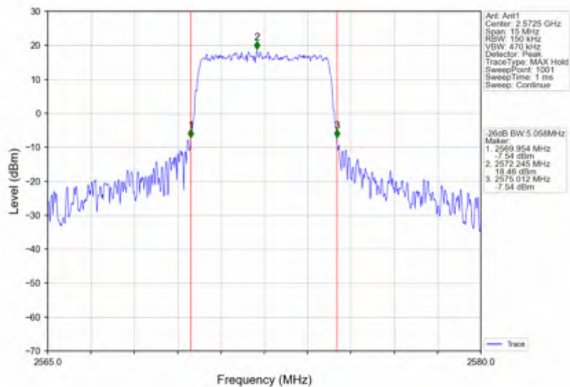
Band38 5MHz 16QAM LCH 2572.5MHz RB 25 0 NTNV
