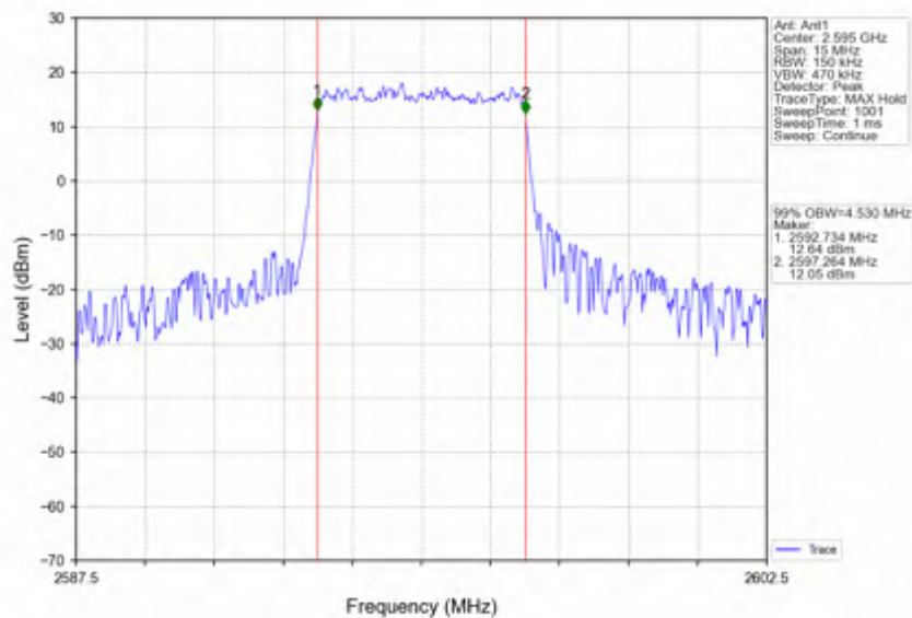
Band38_5MHz_64QAM_MCH_2595MHz_RB_25_0_NTNV
