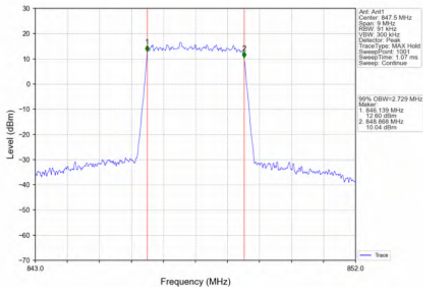
Band26b_3MHz_256QAM_HCH_847.5MHz_RB_15_0_NTNV
