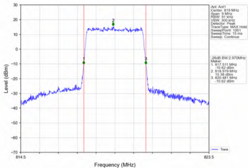
Band26a 3MHz 64QAM MCH 819MHz RB 15 0 NTNV
