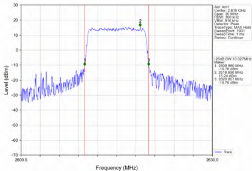
Band38_10MHz_256QAM_HCH_2615MHz_RB_50_0_NTNV
