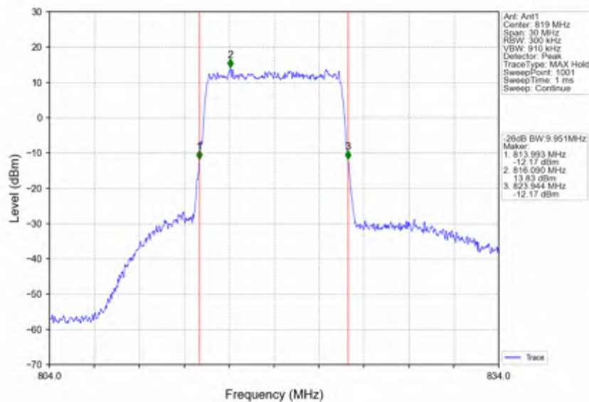
Band26a_10MHz_256QAM_LCH_819MHz_RB_50_0_NTNV
