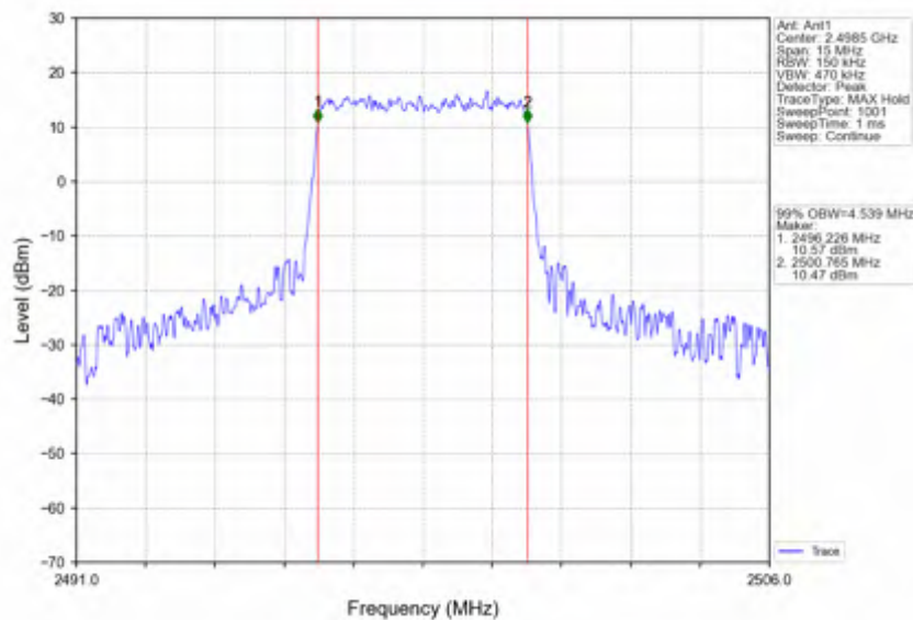
Band41_5MHz_256QAM_LCH_2498.5MHz_RB_25_0_NTNV
