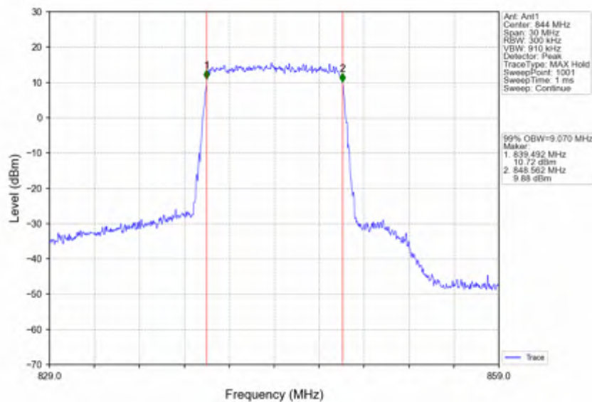
Band26b_10MHz_256QAM_HCH_844MHz_RB_50_0_NTNV
