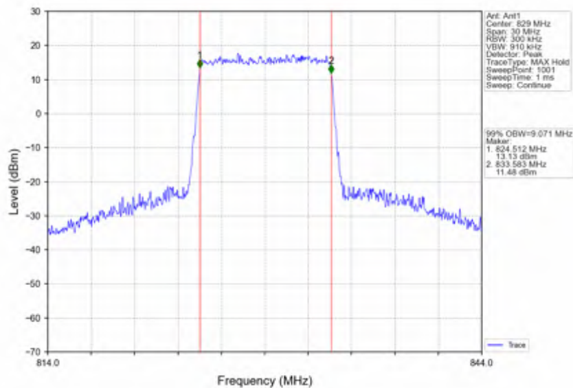
Band26b 10MHz 16QAM LCH 829MHz RB 50 0 NTNV
