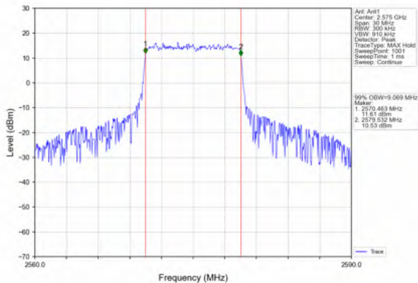
Band38_10MHz_256QAM_LCH_2575MHz_RB_50_0_NTNV
