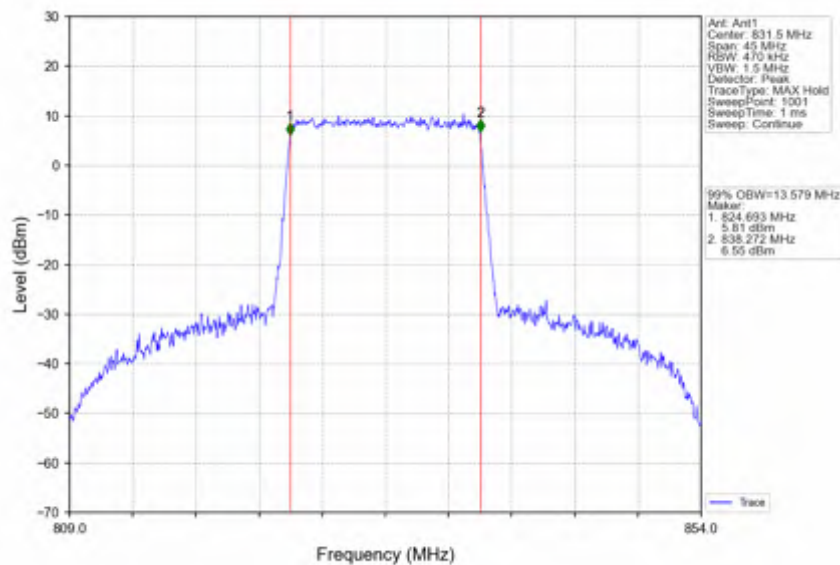
Band26c_15MHz_16QAM_LCH_831.5MHz_RB_75_0_NTNV
