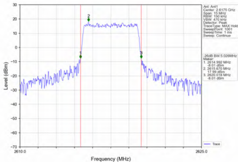
Band38_5MHz_16QAM_HCH_2617.5MHz_RB_25_0_NTNV
