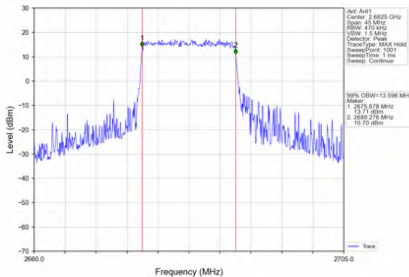
Band41_15MHz_256QAM_HCH_2682.5MHz_RB_75_0_NTNV
