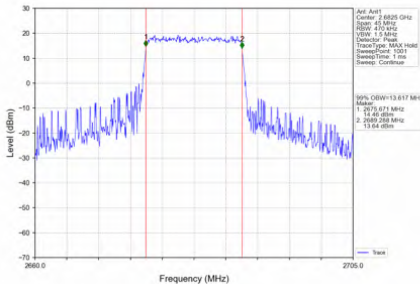
Band41_15MHz_16QAM_HCH_2682.5MHz_RB_75_0_NTNV
