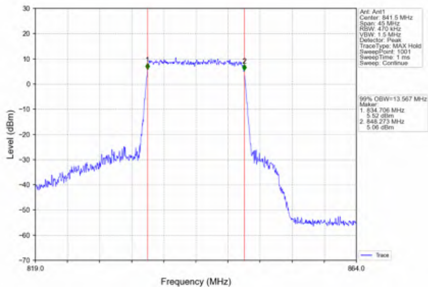
Band26c 15MHz 16QAM HCH 841.5MHz RB 75 0 NTNV
