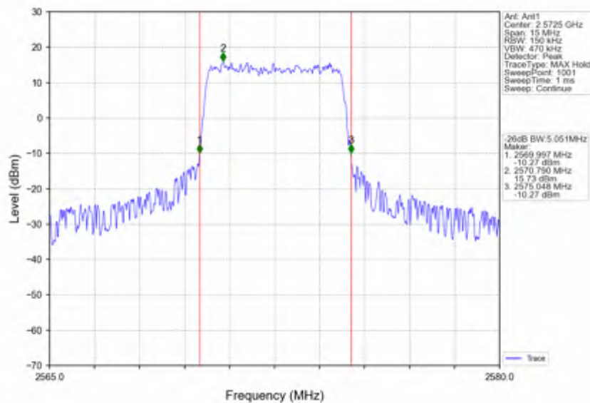
Band38_5MHz_256QAM_LCH_2572.5MHz_RB_25_0_NTNV
