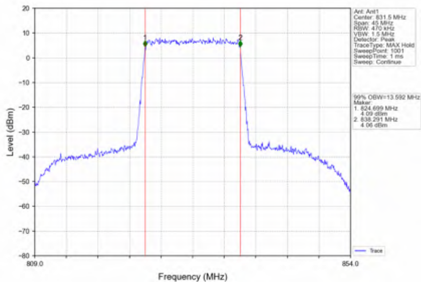
Band26c_15MHz_256QAM_LCH_831.5MHz_RB_75_0_NTNV
