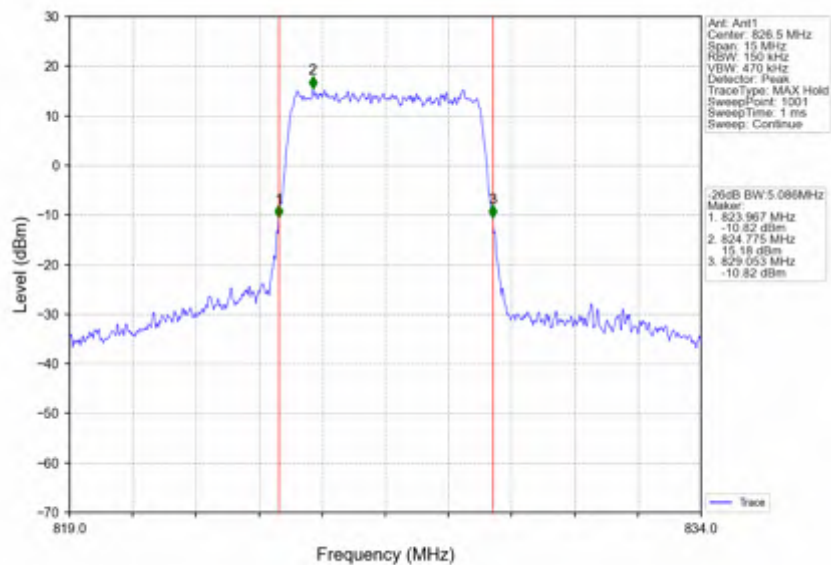
Band26b_5MHz_256QAM_LCH_826.5MHz_RB_25_0_NTNV
