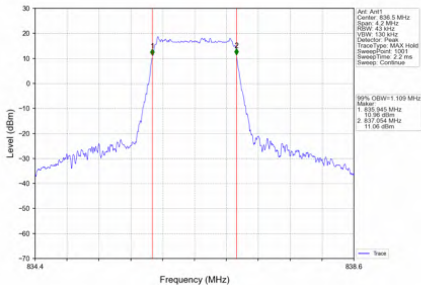
Band26b 1.4MHz 64QAM MCH 836.5MHz RB 6 0 NTNV
