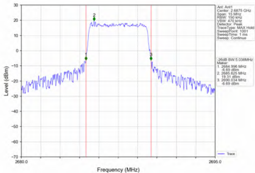
Band41_5MHz_16QAM_HCH_2687.5MHz_RB_25_0_NTNV
