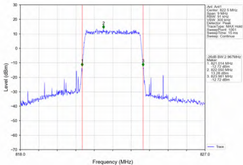
Band26a_3MHz_256QAM_HCH_822.5MHz_RB_15_0_NTNV
