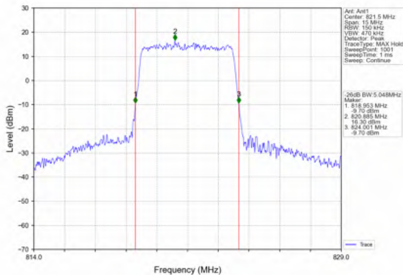
Band26a_5MHz_16QAM_HCH_821.5MHz_RB_25_0_NTNV
