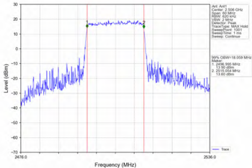
Band41_20MHz_16QAM_LCH_2506MHz_RB_100_0_NTNV
