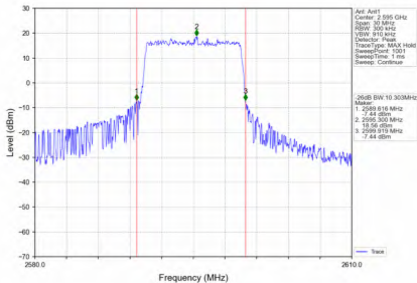
Band38_10MHz_64QAM_MCH_2595MHz_RB_50_0_NTNV
