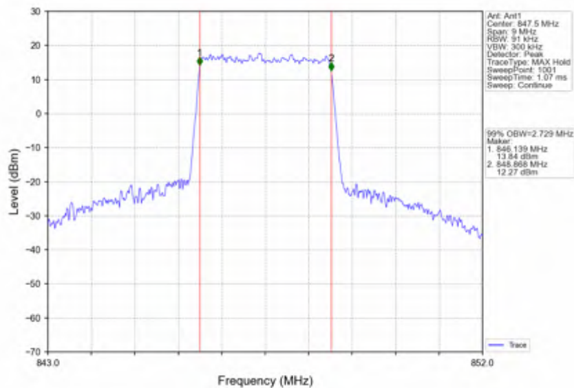
Band26b_3MHz_16QAM_HCH_847.5MHz_RB_15_0_NTNV
