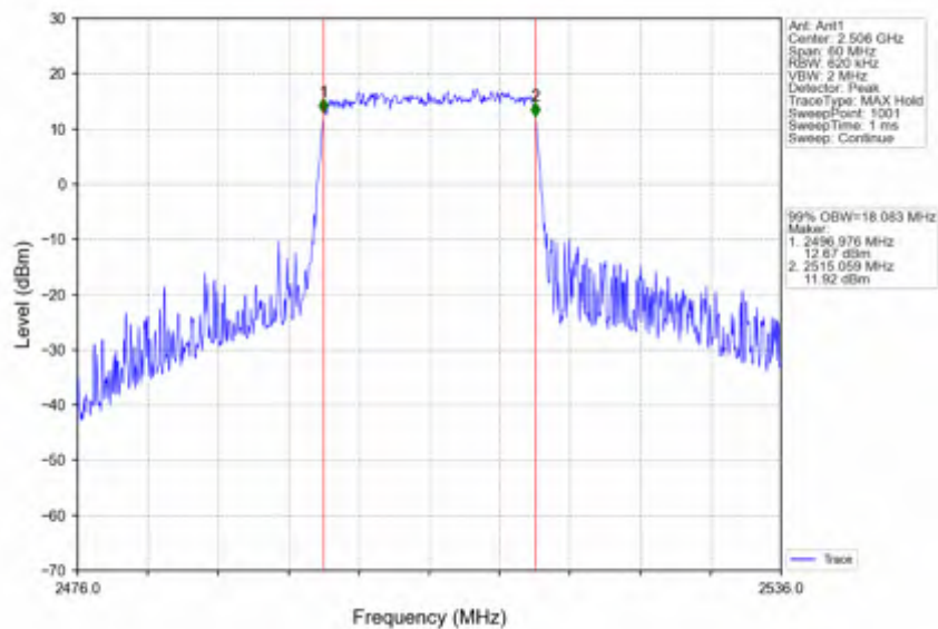
Band41_20MHz_256QAM_LCH_2506MHz_RB_100_0_NTNV
