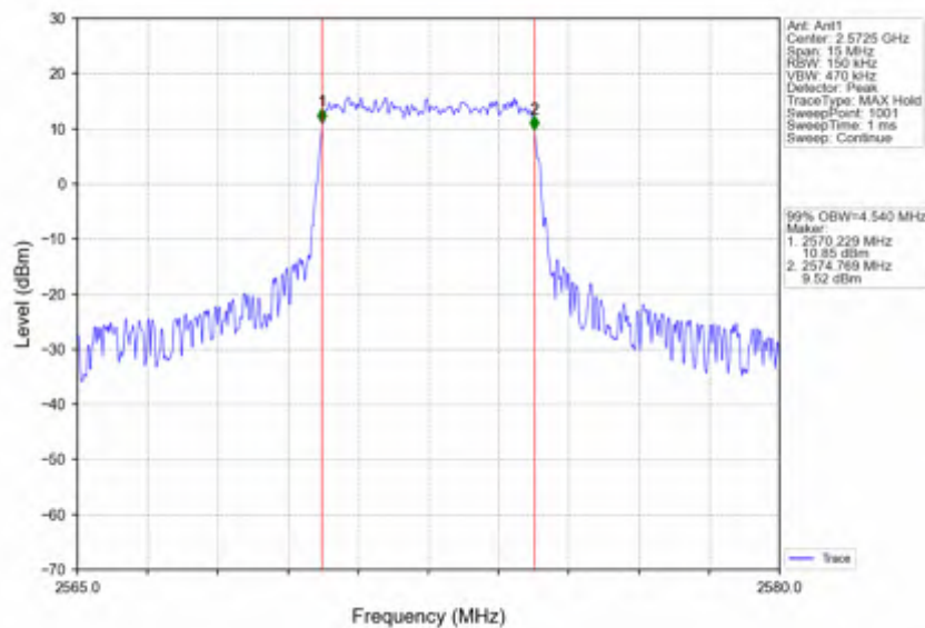
Band38_5MHz_256QAM_LCH_2572.5MHz_RB_25_0_NTNV
