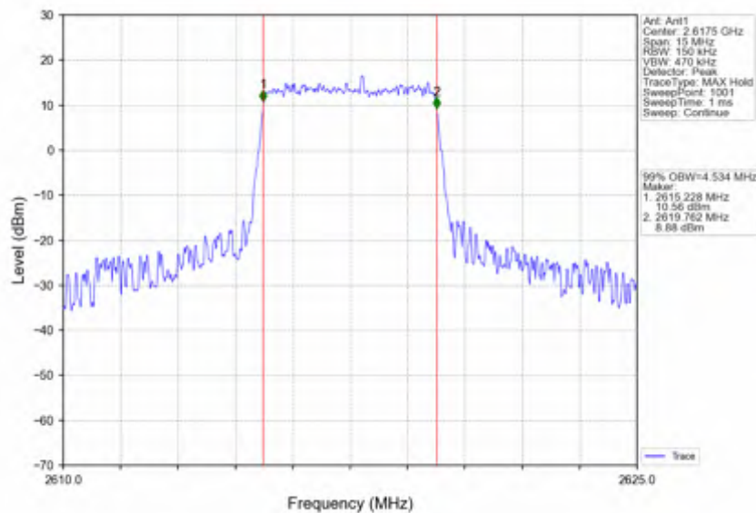
Band38 5MHz 256QAM HCH 2617.5MHz RB 25 0 NTNV
