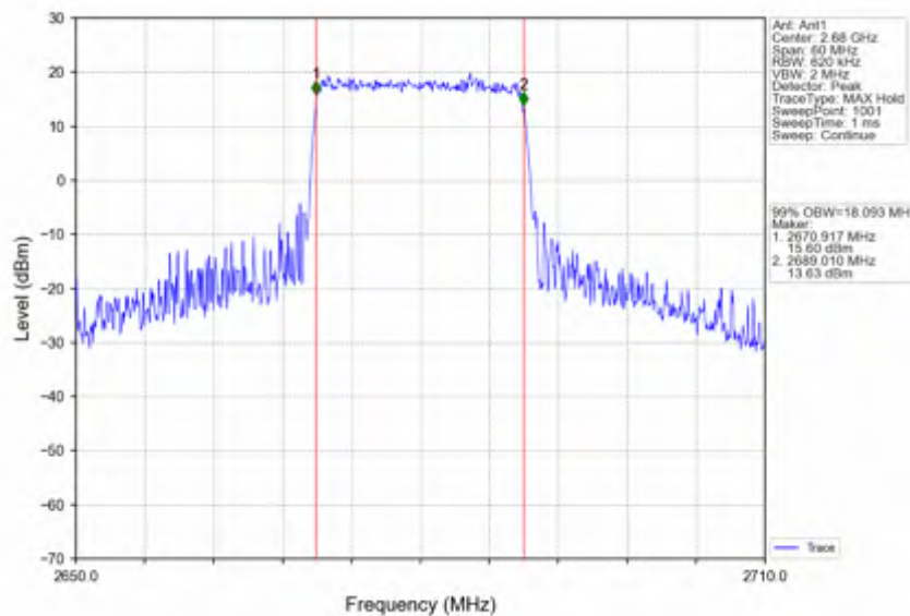
Band41_20MHz_16QAM_HCH_2680MHz_RB_100_0_NTNV
