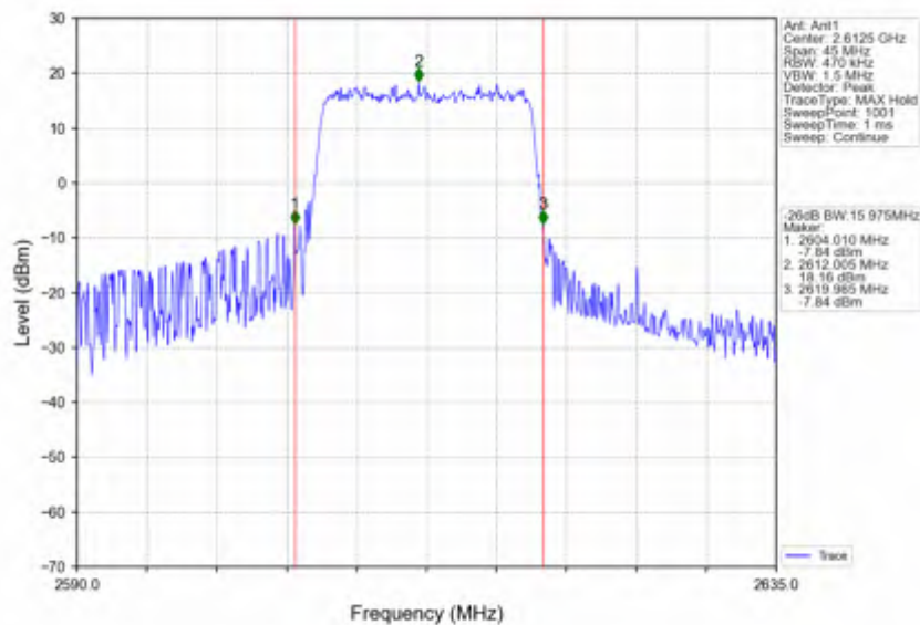
Band38_15MHz_16QAM_HCH_2612.5MHz_RB_75_0_NTNV
