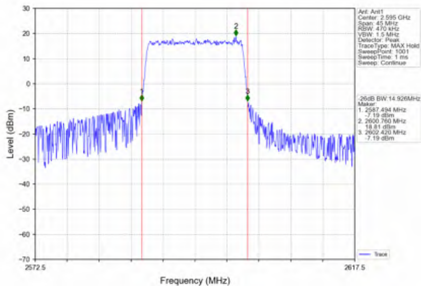
Band38_15MHz_64QAM_MCH_2595MHz_RB_75_0_NTNV
