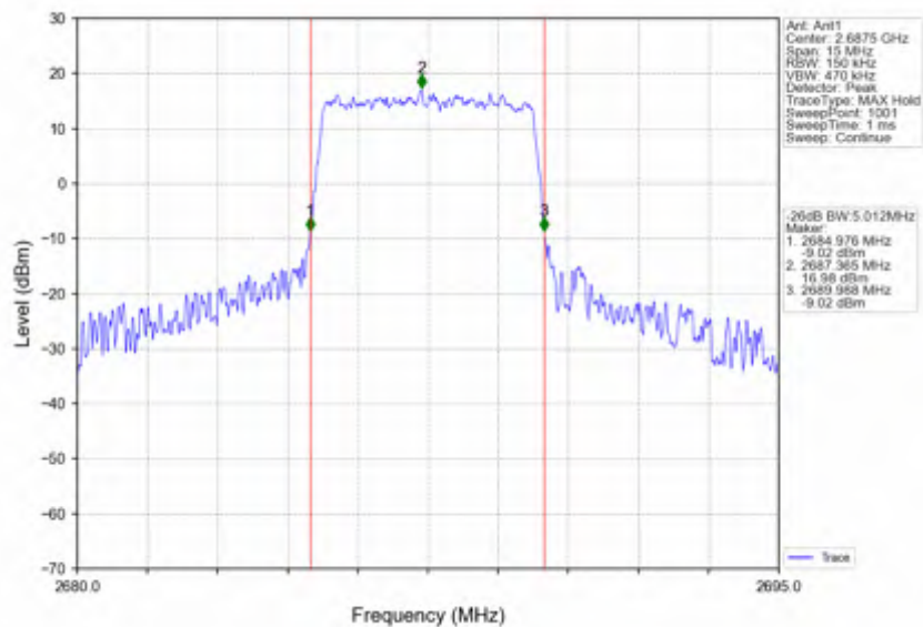
Band41_5MHz_256QAM_HCH_2687.5MHz_RB_25_0_NTNV
