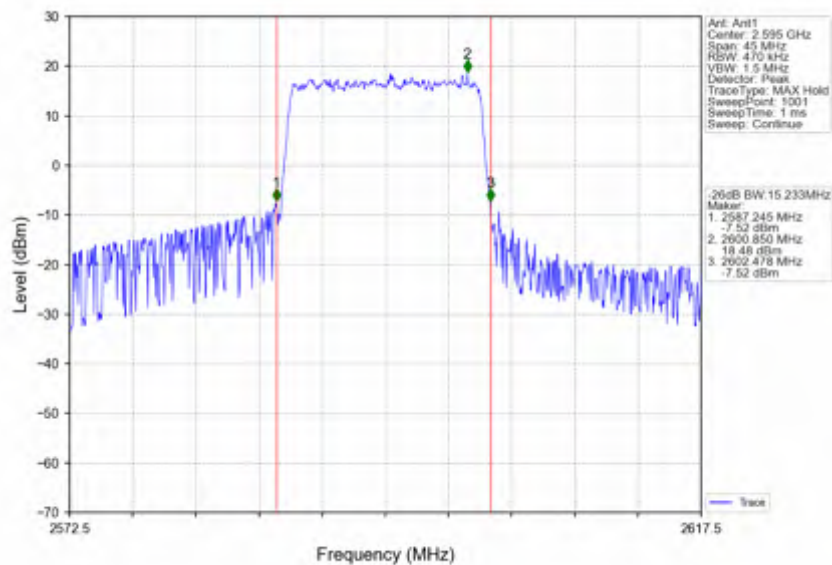
Band38_15MHz_QPSK_MCH_2595MHz_RB_75_0_NTNV
