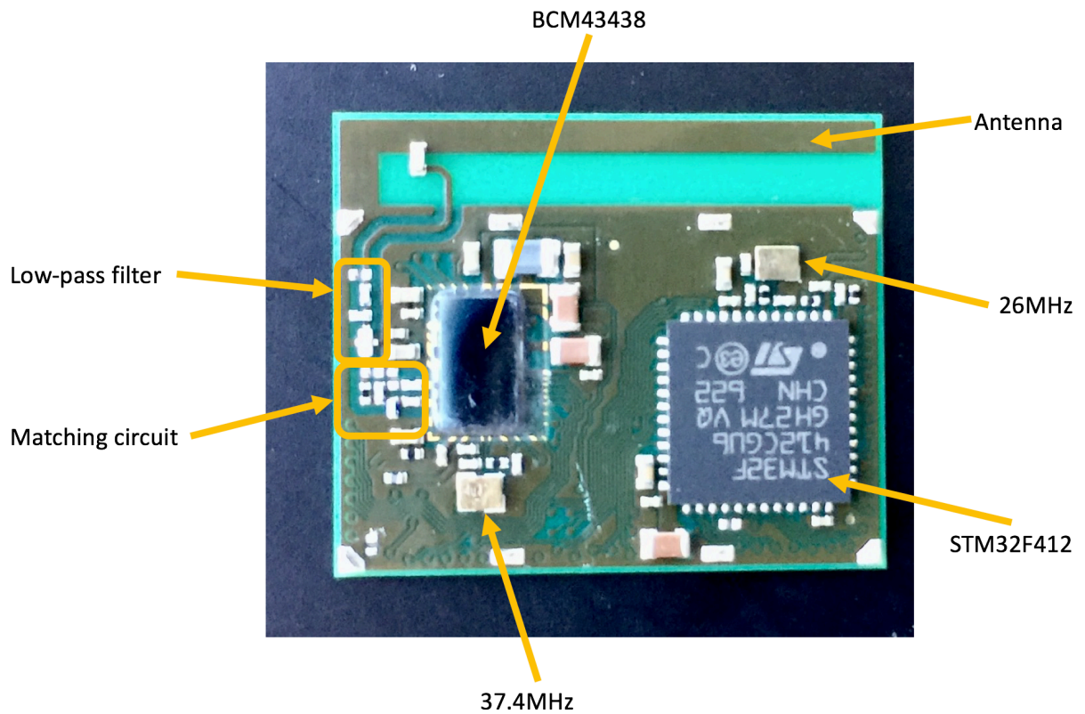
Image 2-1 internal photograph (Shielding removed)
