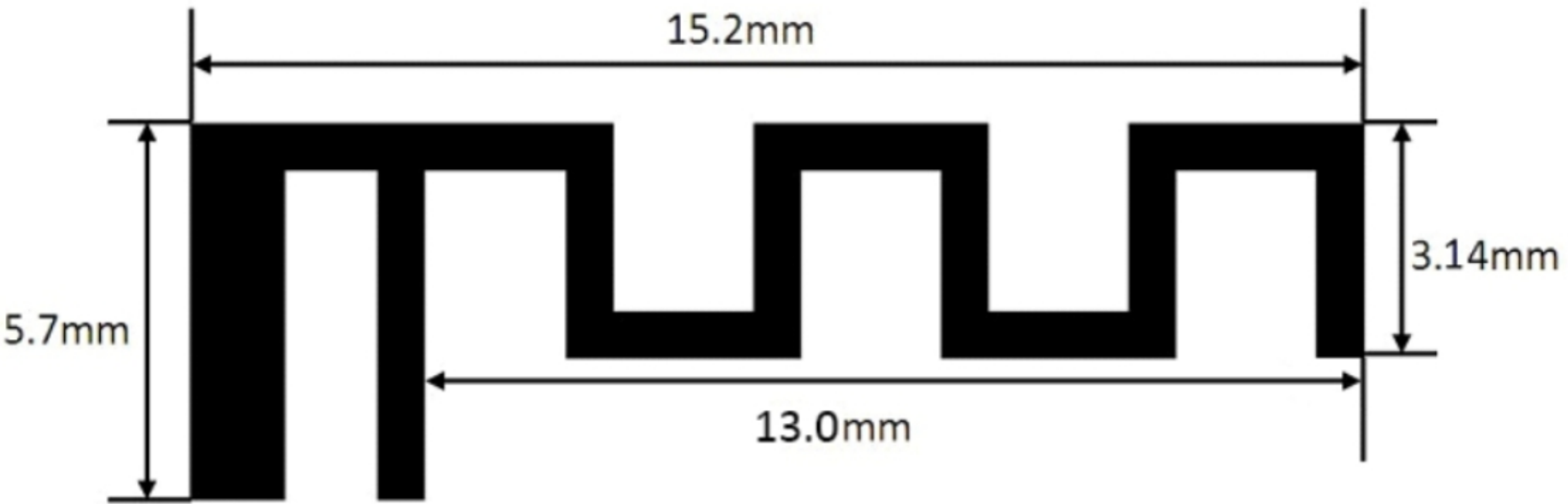
Antenna Photo & Length (mm)
