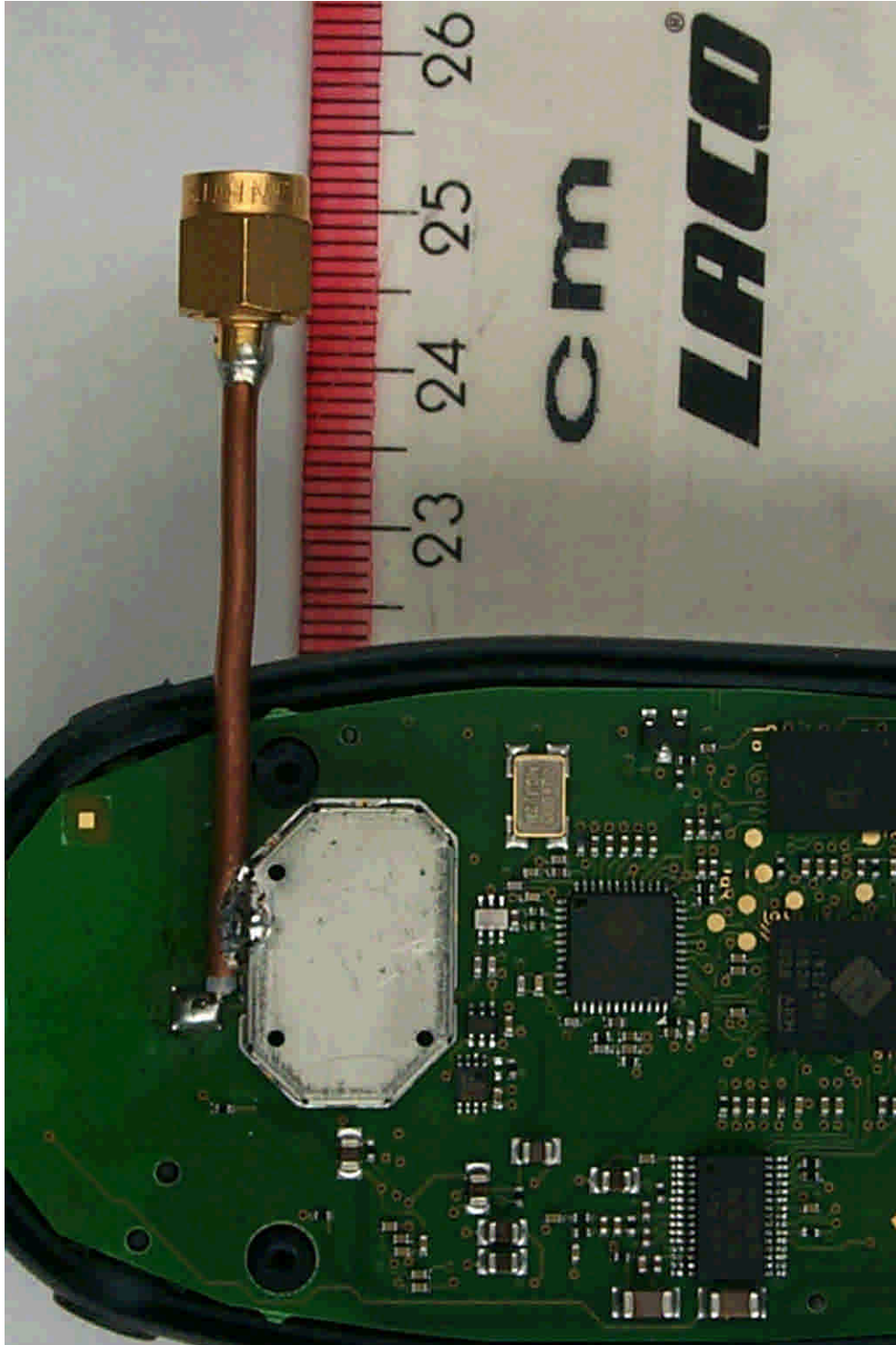
52105_13.jpg EXPLORER Bluetooth handset, sample with antenna connector, PCB, top view
