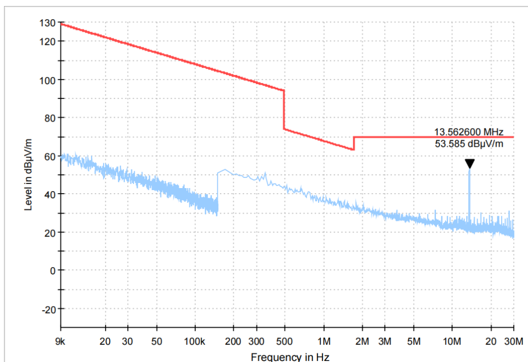
Figure 2 TX mode (9kHz-30MHz)
