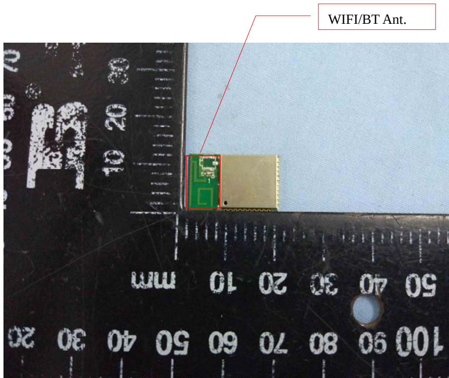
EUT View 1
