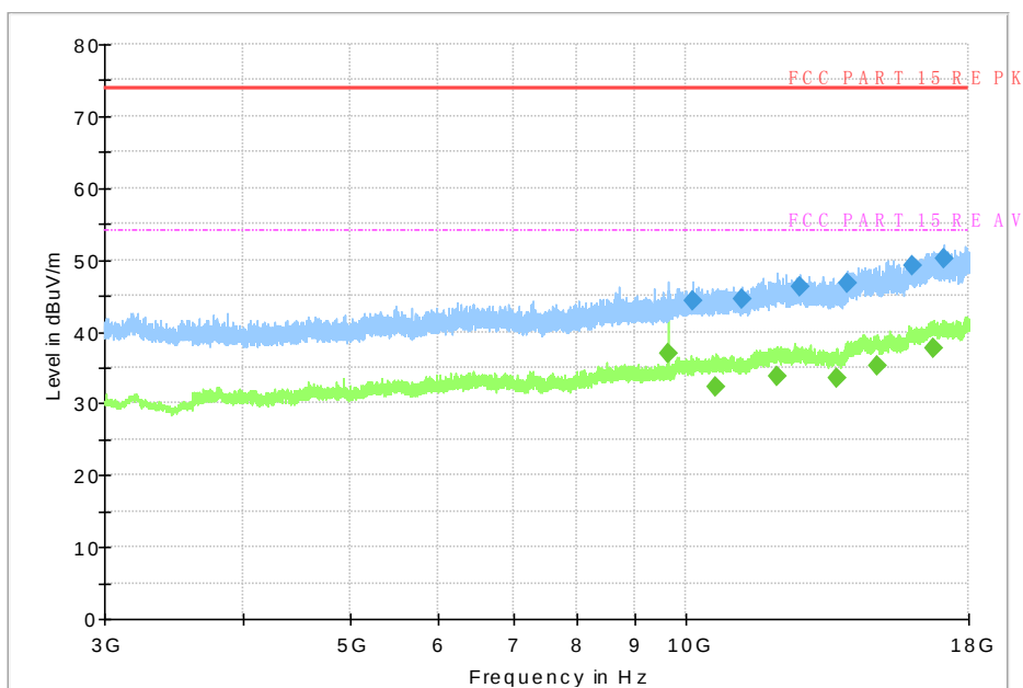
Fig.23 Radiated Spurious Emission (GFSK, Ch19, 3 GHz ~18 GHz)
