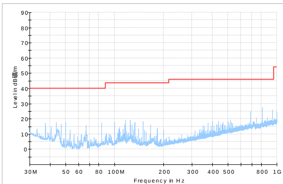
Fig.29 Radiated Spurious Emission (All Channels, 30 MHz-1 GHz)
