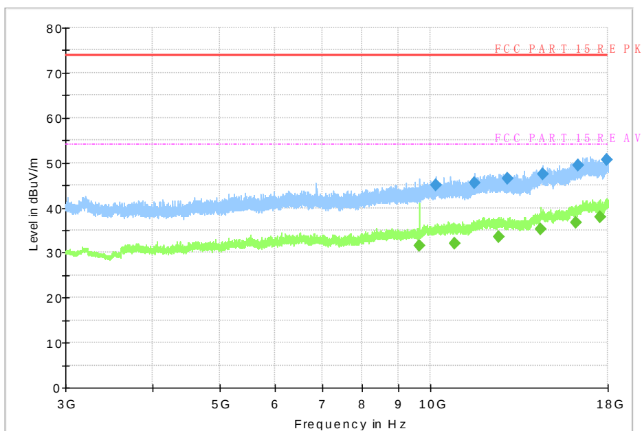
Fig.25 Radiated Spurious Emission (GFSK, Ch39, 3 GHz ~18 GHz)
