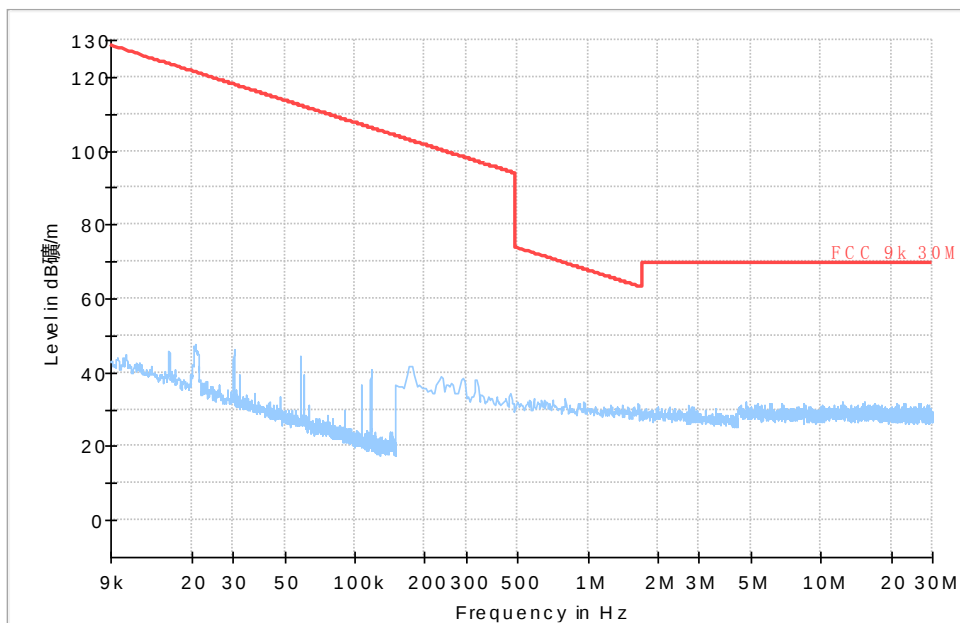
Fig.28 Radiated Spurious Emission (All Channels, 9 kHz-30 MHz)
