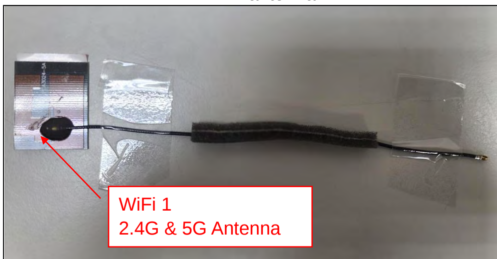
WiFi 1 antenna
