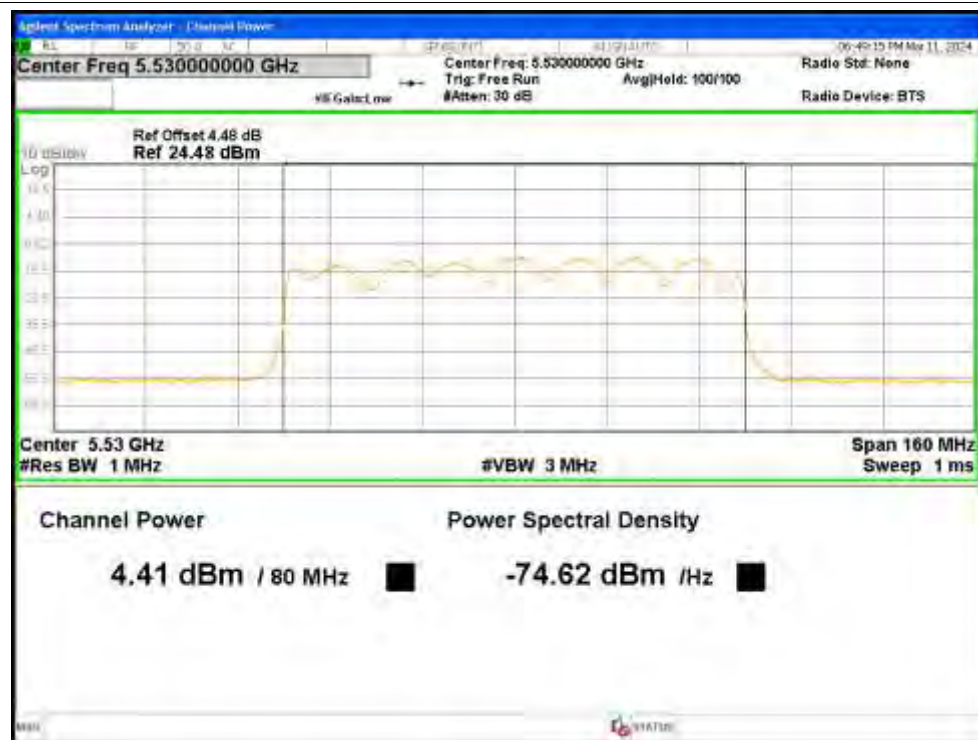
Power NVNT ax80 5530MHz Ant4
