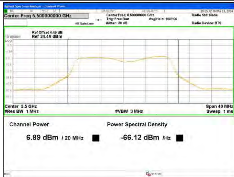
Power NVNT a 5500MHz Ant4
