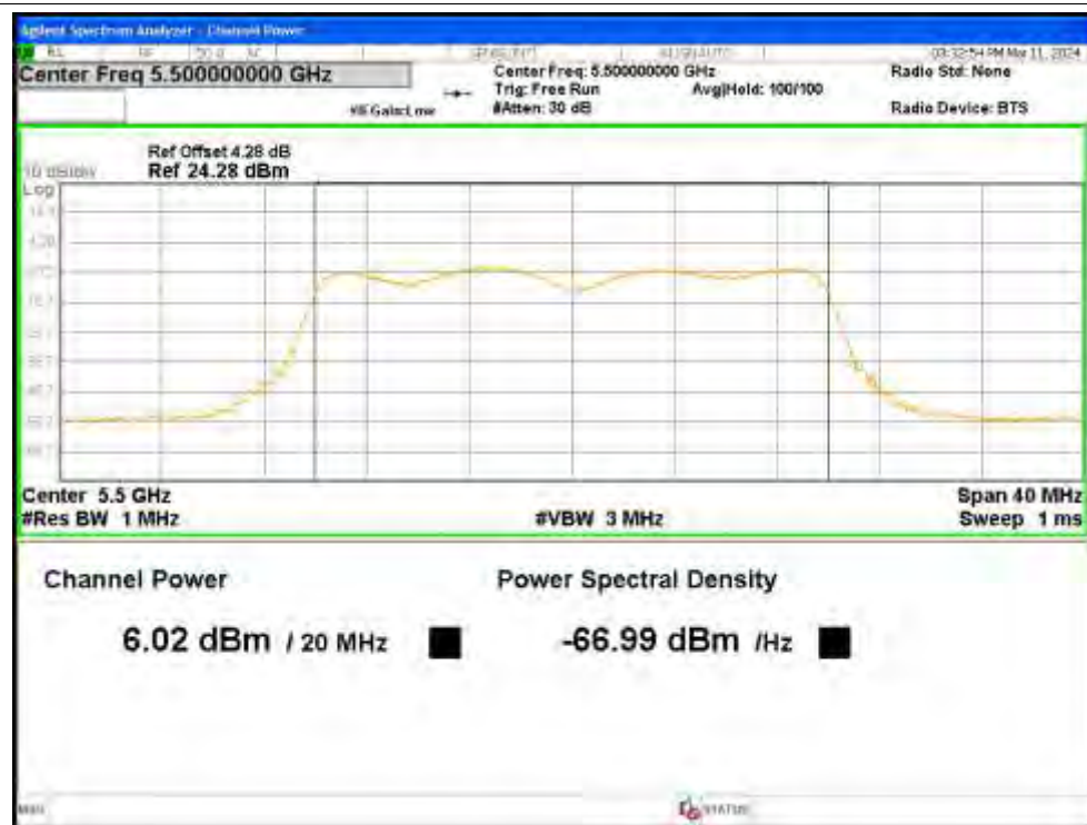
Power NVNT ax20 5500MHz Ant4
