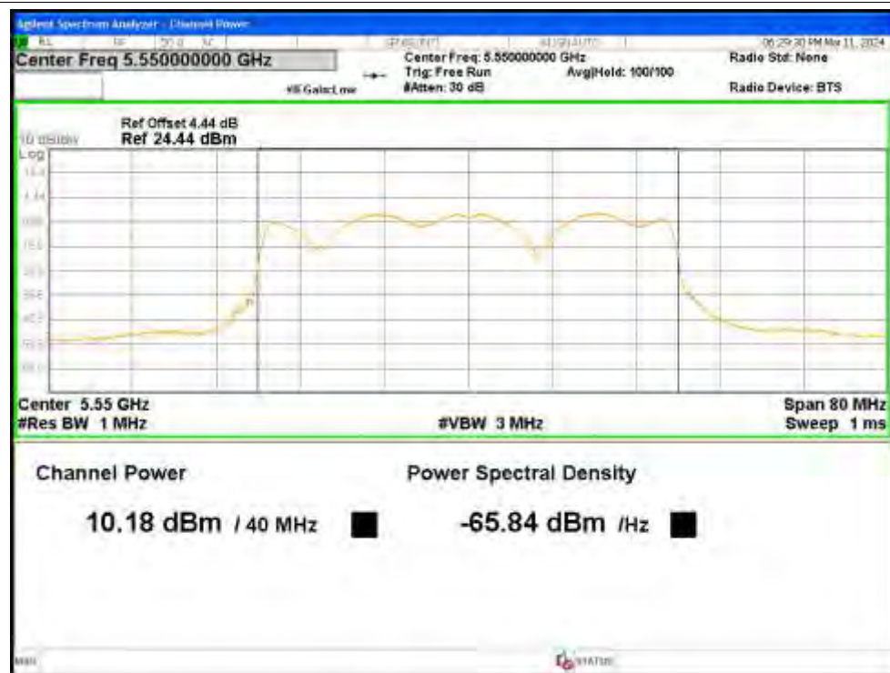
Power NVNT ax40 5550MHz Ant2
