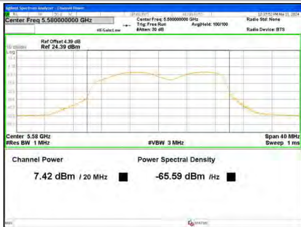
Power NVNT ac20 5580MHz Ant4
