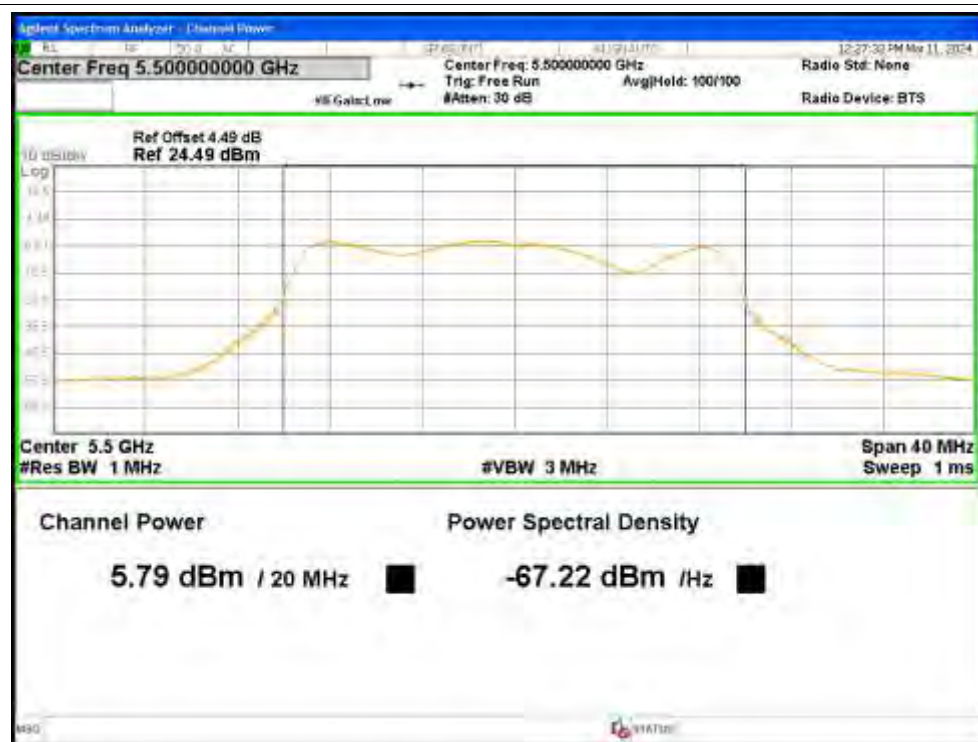
Power NVNT ac20 5500MHz Ant4
