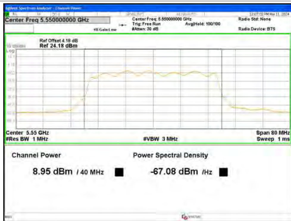
Power NVNT n40 5550MHz Ant4
