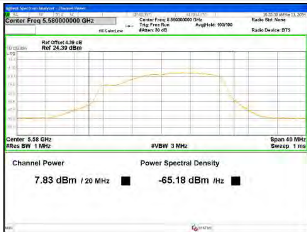
Power NVNT a 5580MHz Ant4
