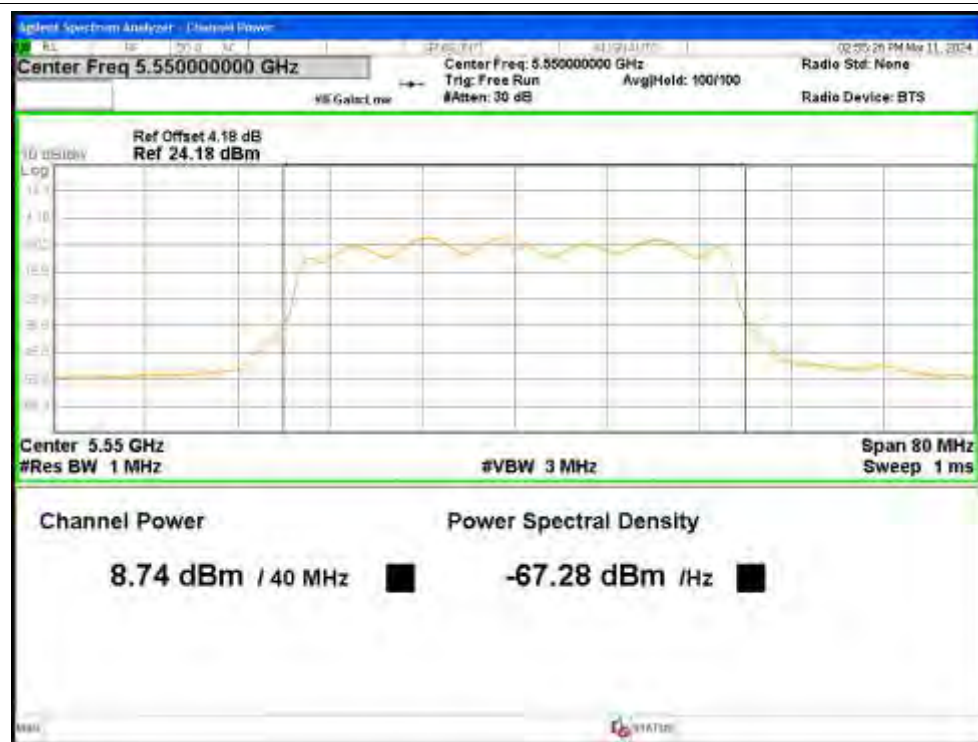
Power NVNT ac40 5550MHz Ant4
