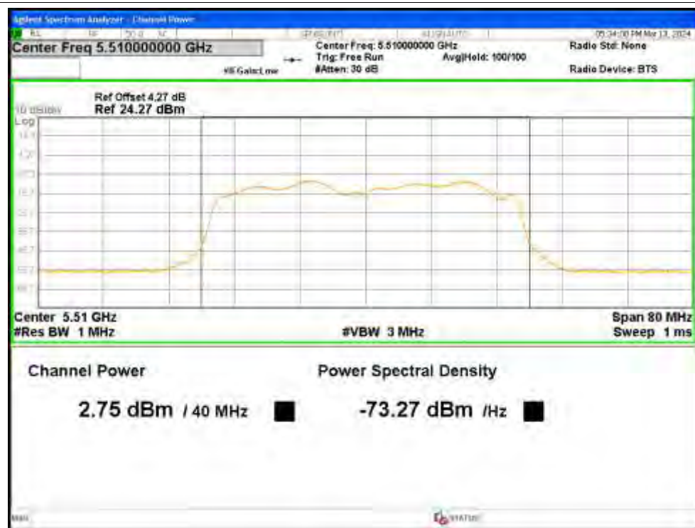
Power NVNT n40 5510MHz Ant4
