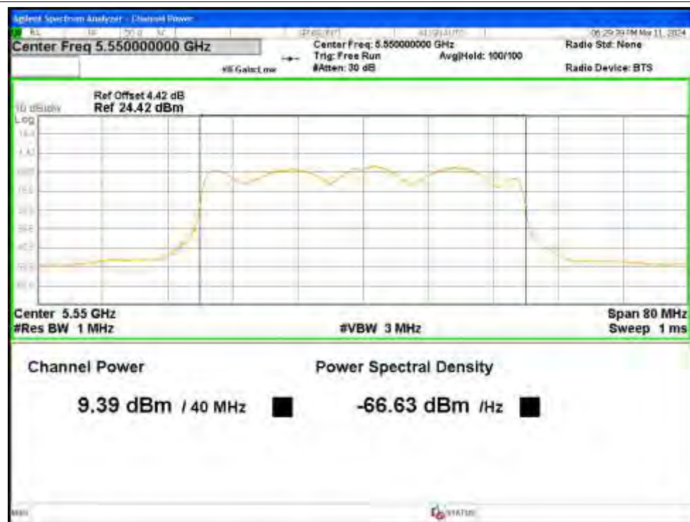
Power NVNT ax40 5550MHz Ant4
