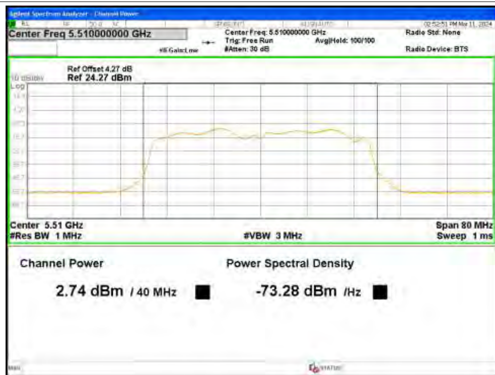
Power NVNT ac40 5510MHz Ant4
