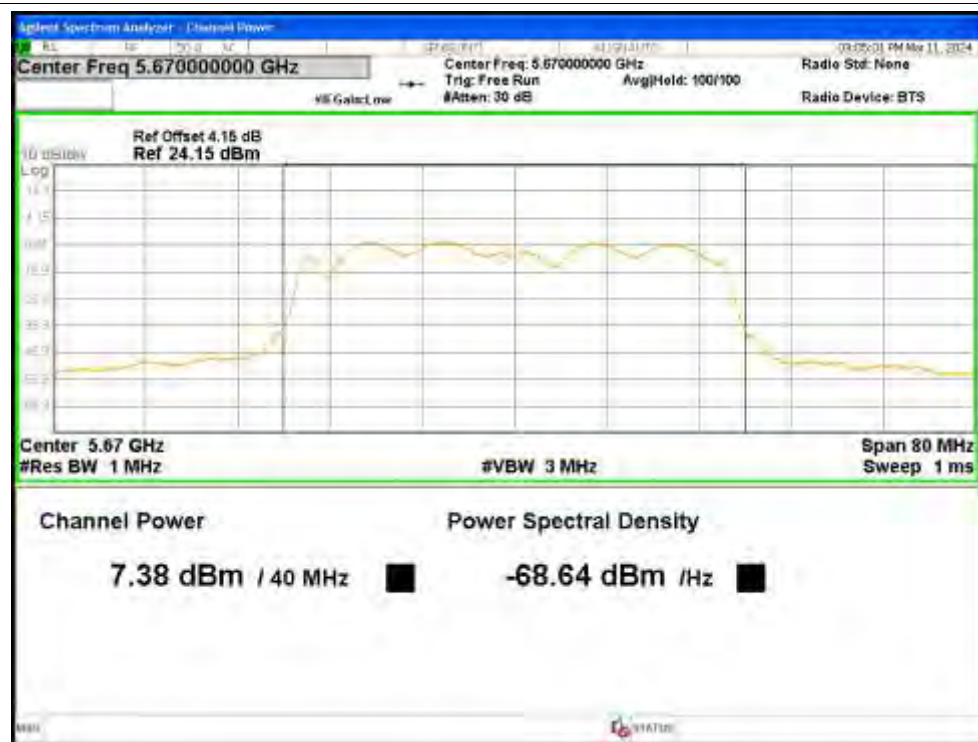
Power NVNT ac40 5670MHz Ant4
