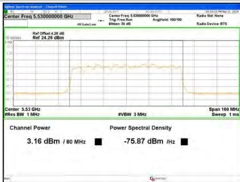
Power NVNT ac80 5530MHz Ant4
