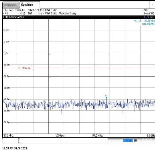
Band25-20MHz-16QAM-26590-1RB#0- Range1:30~1000MHz
