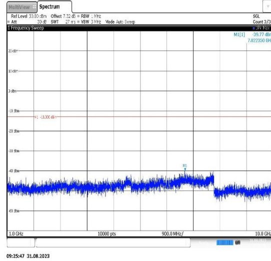
Band26(814-824)-3MHz-16QAM-26740-1RB#0-Range2:1000~10000MHz
