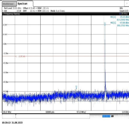
Band26(814-824)-5MHz-16QAM-26740-1RB#0-Range1:30~1000MHz
