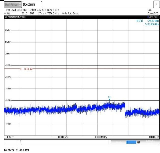
Band26(814-824)-5MHz-16QAM-26740-1RB#0-Range2:1000~10000MHz
