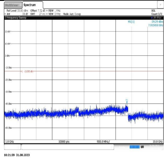
Band26(814-824)-10MHz-QPSK-26740-1RB#0-Range2:1000~10000MHz
