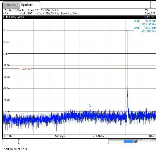
Band26(814-824)-5MHz-16QAM-26765-1RB#0-Range1:30~1000MHz
