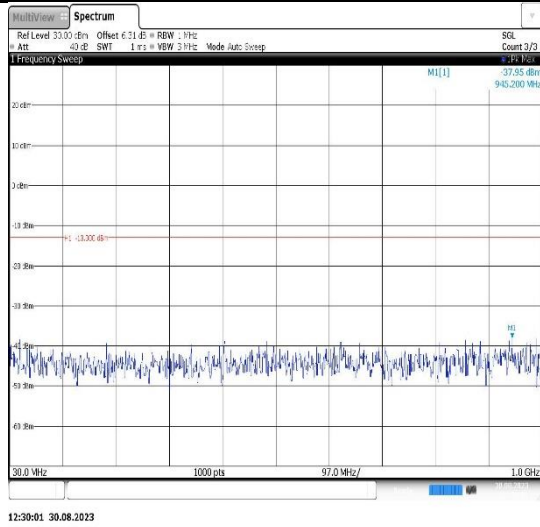
Band25-20MHz-16QAM-26140-1RB#0- Range1:30~1000MHz
