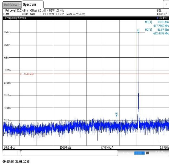
Band26(814-824)-3MHz-QPSK-26775-1RB#0- Range1:30~1000MHz
