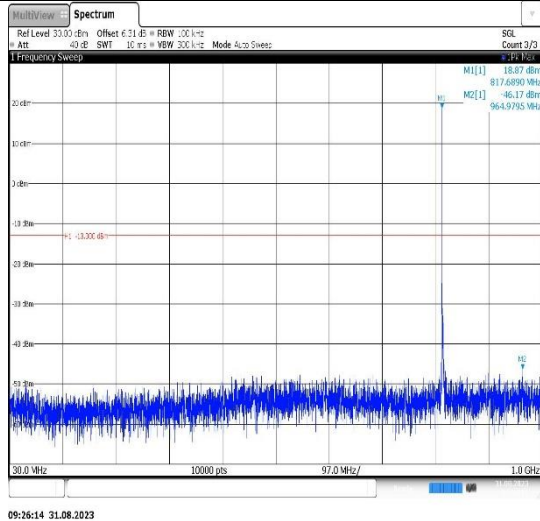
Band26(814-824)-3MHz-16QAM-26775-1RB#0-Range1:30~1000MHz
