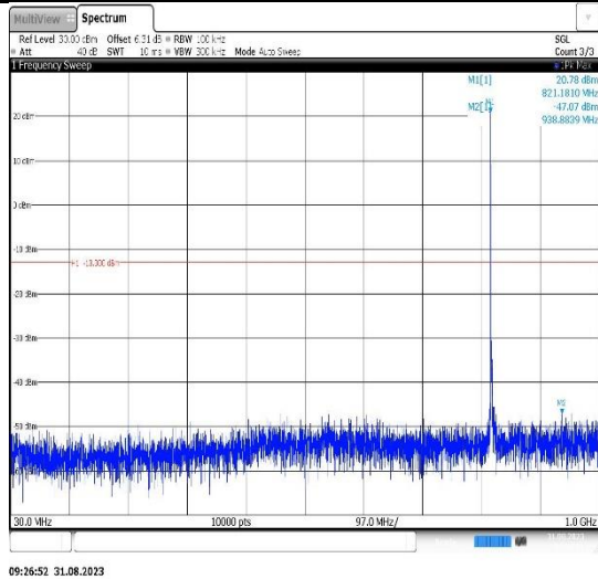
Band26(814-824)-5MHz-QPSK-26715-1RB#0- Range1:30~1000MHz
