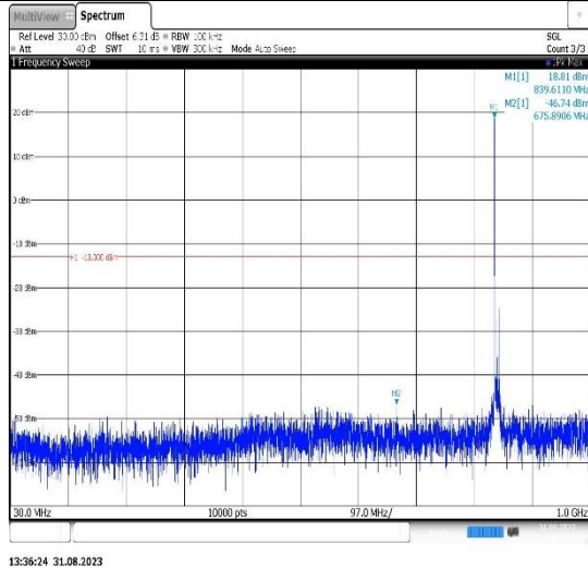
Band26(824-849)-10MHz-16QAM-26840-1RB#0-Range1:30~1000MHz
