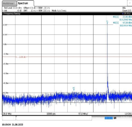
Band26(814-824)-5MHz-QPSK-26740-1RB#0- Range1:30~1000MHz
