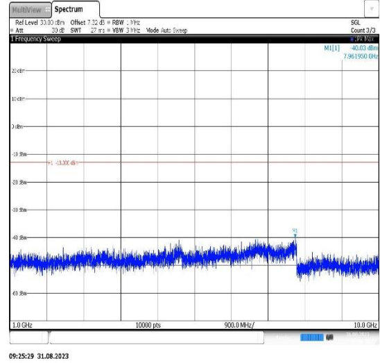
Band26(814-824)-3MHz-QPSK-26740-1RB#0- Range2:1000~10000MHz
