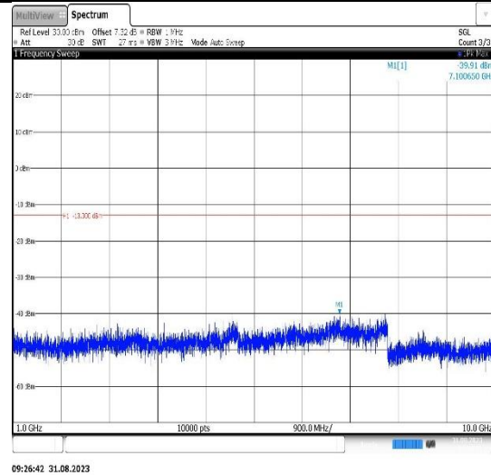
Band26(814-824)-3MHz-16QAM-26705-1RB#0-Range2:1000~10000MHz
