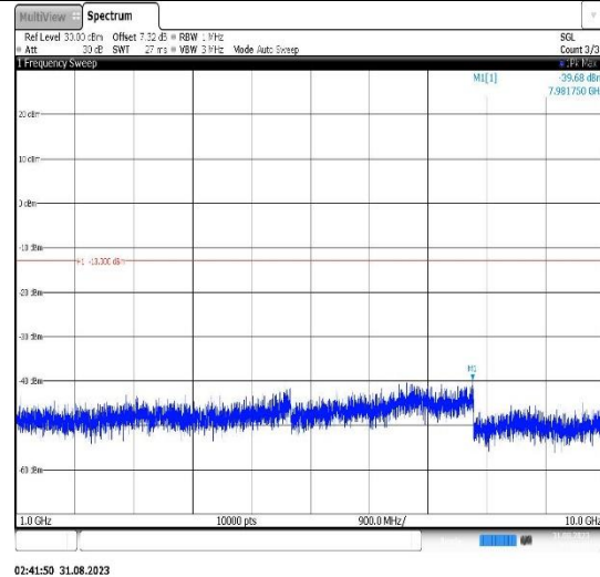
Band26(814-824)-1.4MHz-16QAM-26783-1RB#0-Range2:1000~10000MHz
