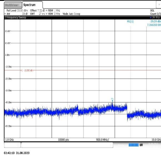
Band26(814-824)-1.4MHz-16QAM-26697-1RB#0-Range2:1000~10000MHz
