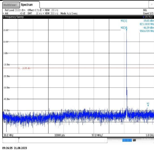
Band26(814-824)-3MHz-16QAM-26705-1RB#0-Range1:30~1000MHz
