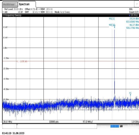
Band26(814-824)-3MHz-QPSK-26705-1RB#0- Range1:30~1000MHz
