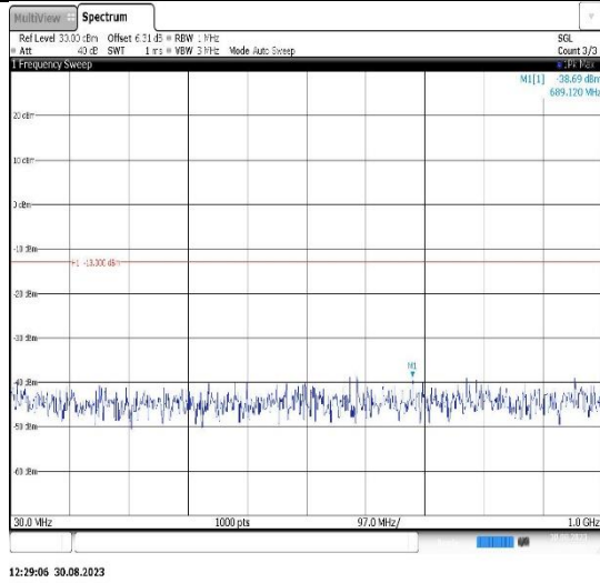
Band25-20MHz-16QAM-26365-1RB#0- Range1:30~1000MHz
