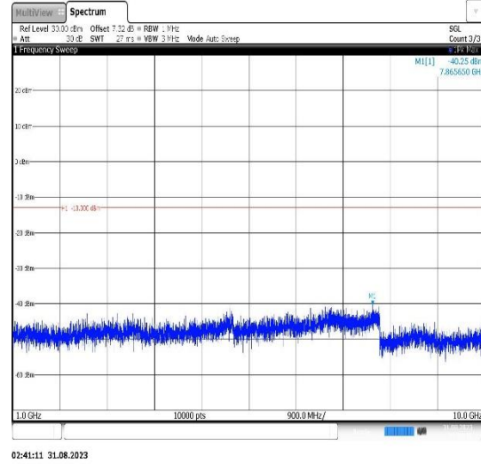
Band26(814-824)-1.4MHz-16QAM-26740-1RB#0-Range2:1000~10000MHz
