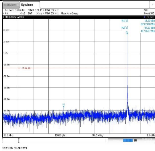
Band26(814-824)-10MHz-QPSK-26740-1RB#0-Range1:30~1000MHz
