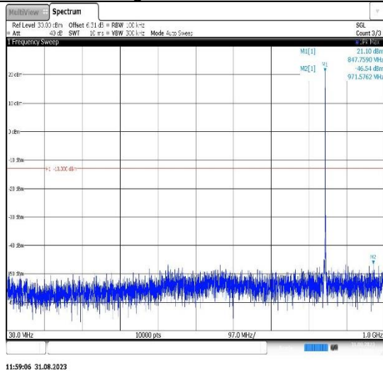
Band26(824-849)-1.4MHz-16QAM-26797-1RB#0-Range1:30~1000MHz
