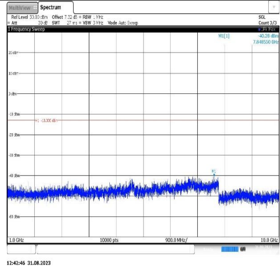
Band26(824-849)-3MHz-16QAM-26805-1RB#0-Range2:1000~10000MHz
