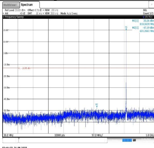
Band26(814-824)-1.4MHz-QPSK-26783-1RB#0-Range1:30~1000MHz
