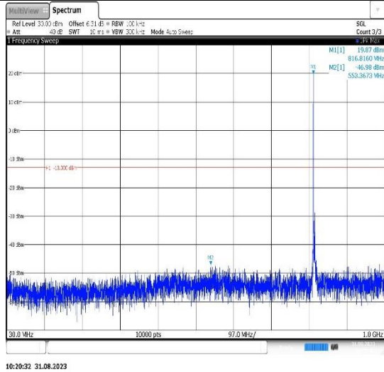
Band26(814-824)-5MHz-QPSK-26765-1RB#0- Range1:30~1000MHz
