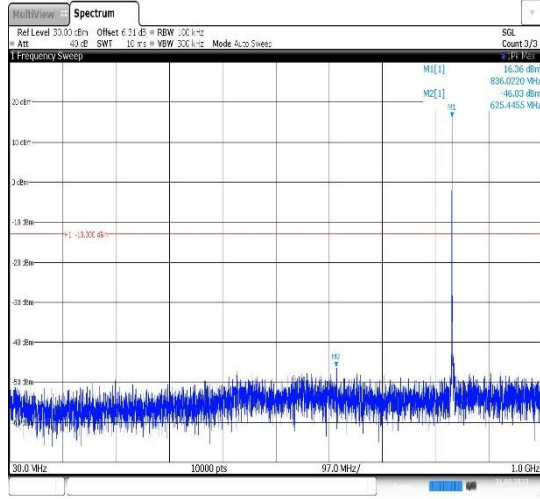
Band26(824-849)-1.4MHz-16QAM-26915-1RB#0- Range1:30~1000MHz
