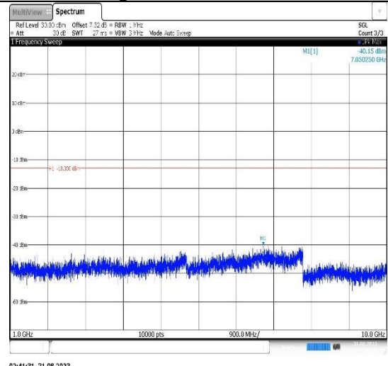
Band26(814-824)-1.4MHz-QPSK-26783-1RB#0-Range2:1000~10000MHz
