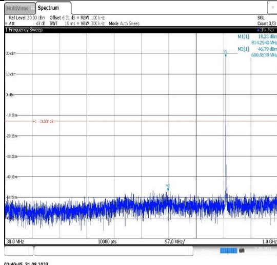
Band26(814-824)-1.4MHz-QPSK-26740-1RB#0-Range1:30~1000MHz
