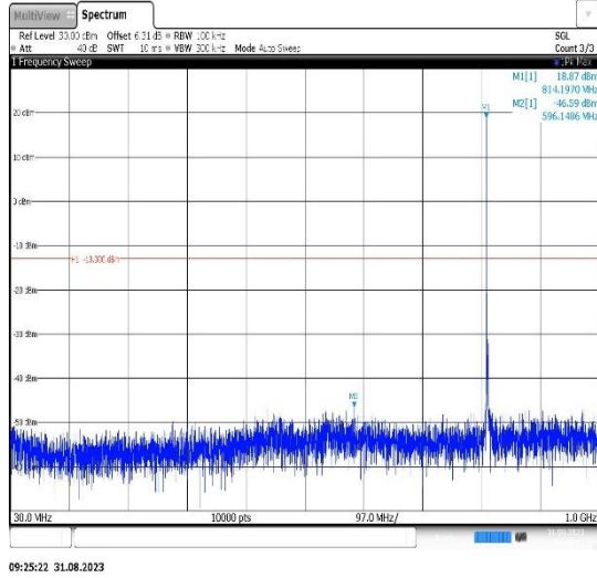
Band26(814-824)-3MHz-QPSK-26740-1RB#0- Range1:30~1000MHz
