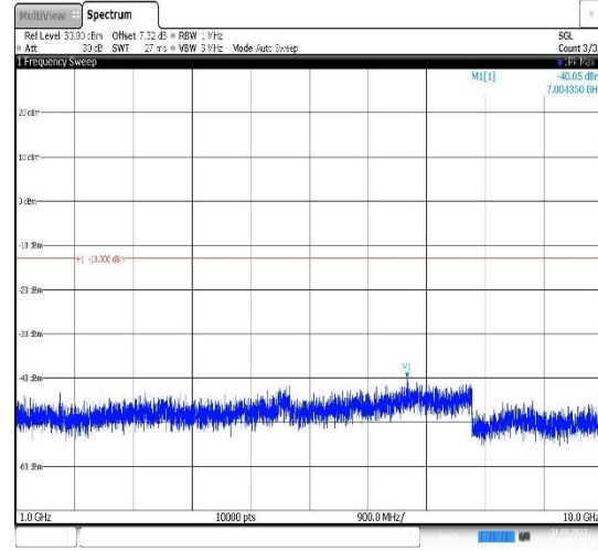
Band26(824-849)-3MHz-16QAM-26915-1RB#0-Range2:1000~10000MHz
