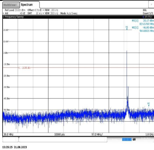
Band26(824-849)-10MHz-16QAM-26915-1RB#0- Range1:30~1000MHz
