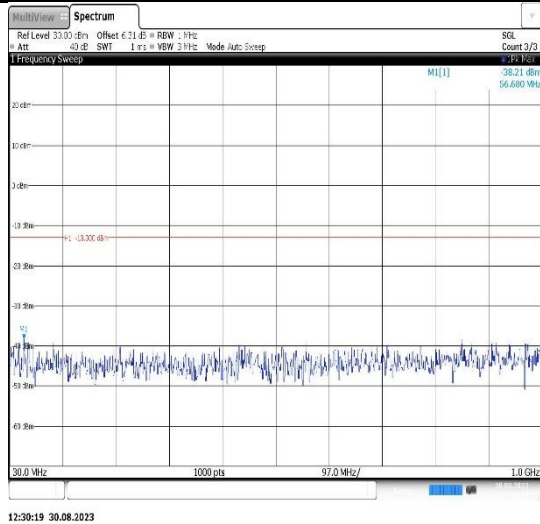
Band26(814-824)-1.4MHz-QPSK-26697-1RB#0-Range1:30~1000MHz
