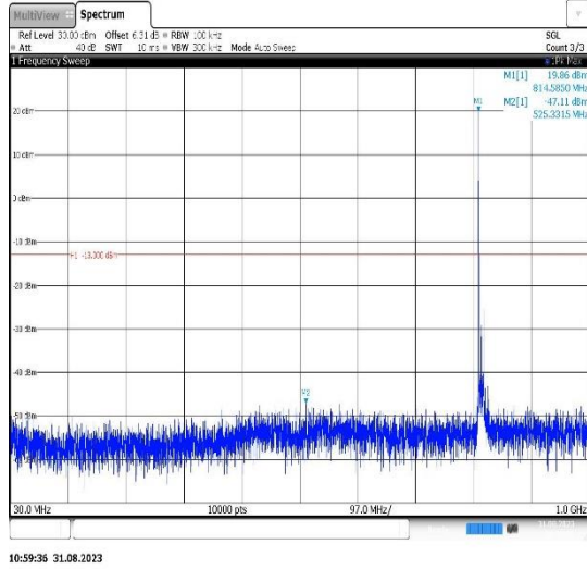
Band26(814-824)-10MHz-16QAM-26740-1RB#0-Range1:30~1000MHz
