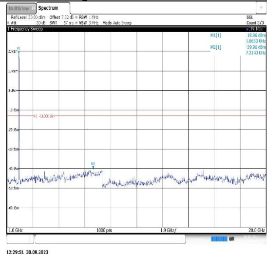
Band25-20MHz-16QAM-26590-1RB#0- Range2:1000~20000MHz
