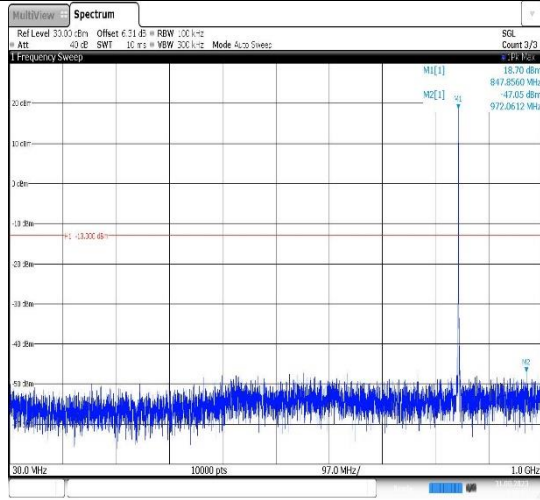
Band26(824-849)-1.4MHz-16QAM-27033-1RB#0- Range1:30~1000MHz
