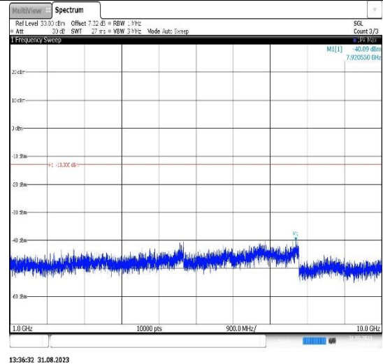
Band26(824-849)-10MHz-16QAM-26840-1RB#0-Range2:1000~10000MHz
