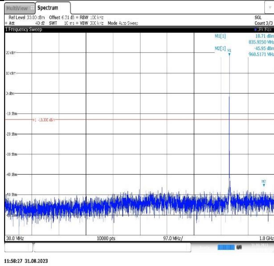
Band26(824-849)-1.4MHz-QPSK-27033-1RB#0-Range1:30~1000MHz
