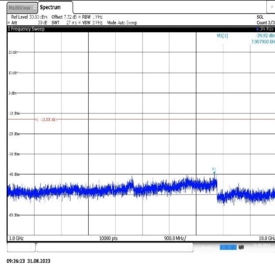
Band26(814-824)-3MHz-16QAM-26775-1RB#0-Range2:1000~10000MHz
