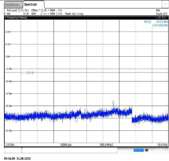
Band26(814-824)-3MHz-QPSK-26775-1RB#0- Range2:1000~10000MHz
