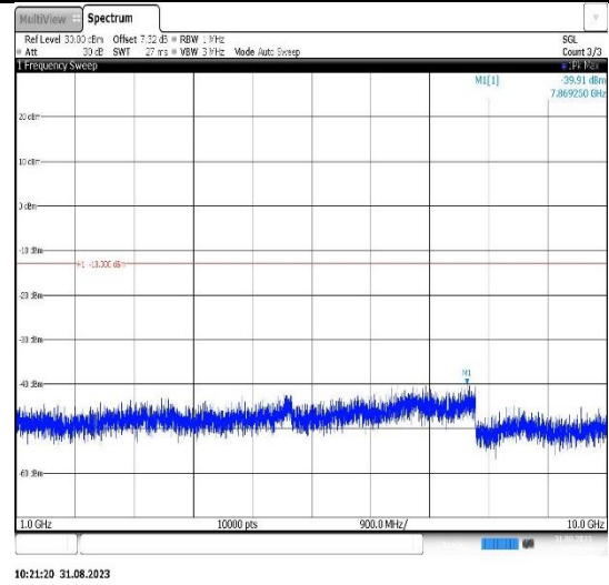
Band26(814-824)-5MHz-16QAM-26715-1RB#0-Range2:1000~10000MHz
