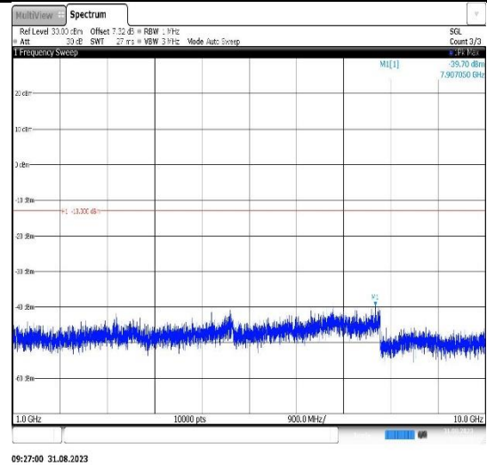
Band26(814-824)-5MHz-QPSK-26715-1RB#0- Range2:1000~10000MHz
