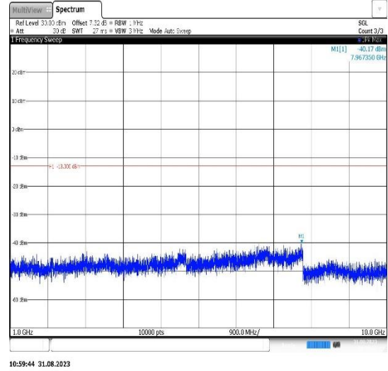
Band26(814-824)-10MHz-16QAM-26740-1RB#0-Range2:1000~10000MHz
