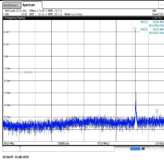
Band26(824-849)-5MHz-QPSK-26915-1RB#0-Range1:30~1000MHz
