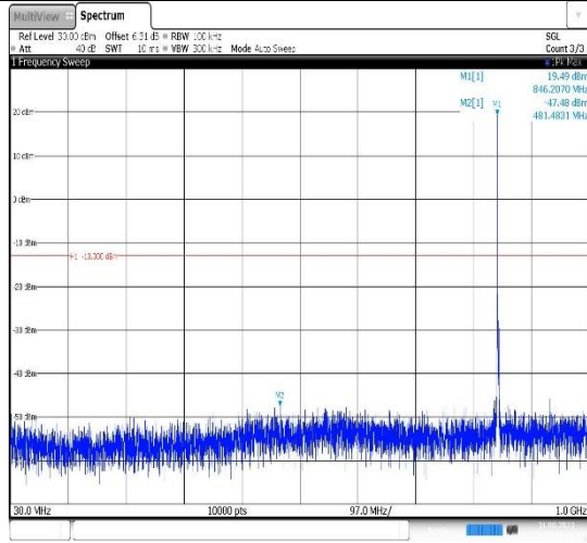
Band26(824-849)-3MHz-16QAM-27025-1RB#0-Range1:30~1000MHz
