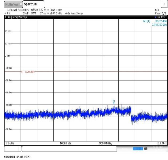
Band26(814-824)-5MHz-QPSK-26740-1RB#0- Range2:1000~10000MHz
