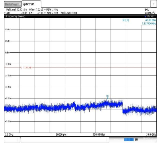
Band26(824-849)-1.4MHz-16QAM-27033-1RB#0- Range2:1000~10000MHz
