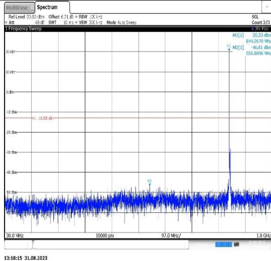
Band26(824-849)-5MHz-16QAM-26815-1RB#0-Range1:30~1000MHz
