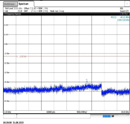
Band26(814-824)-5MHz-16QAM-26765-1RB#0-Range2:1000~10000MHz
