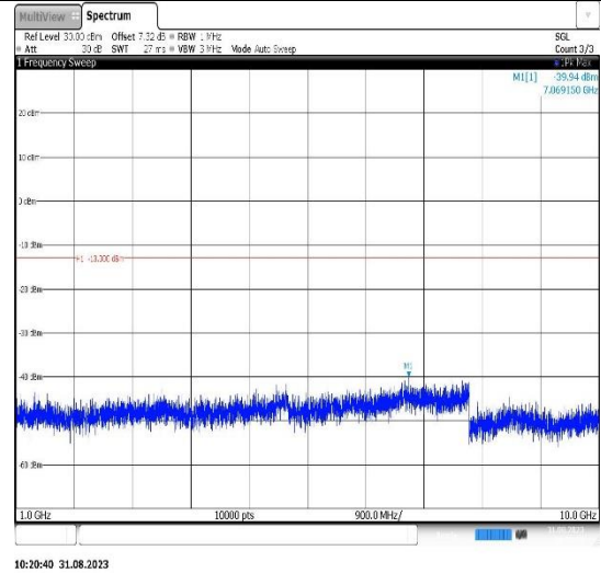
Band26(814-824)-5MHz-QPSK-26765-1RB#0- Range2:1000~10000MHz
