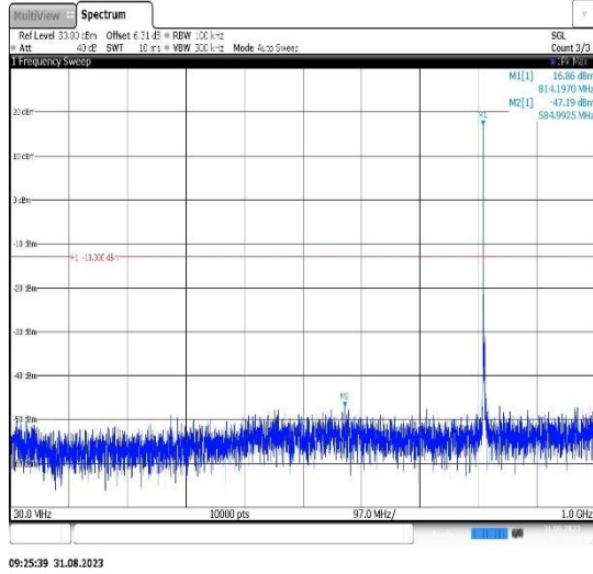
Band26(814-824)-3MHz-16QAM-26740-1RB#0-Range1:30~1000MHz
