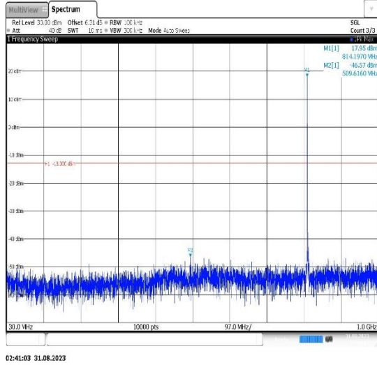
Band26(814-824)-1.4MHz-16QAM-26740-1RB#0-Range1:30~1000MHz
