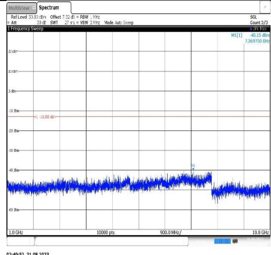
Band26(814-824)-1.4MHz-QPSK-26740-1RB#0-Range2:1000~10000MHz
