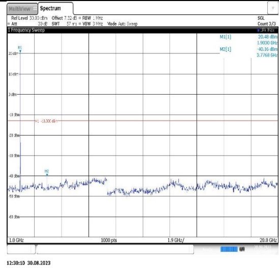
Band25-20MHz-16QAM-26140-1RB#0- Range2:1000~20000MHz
