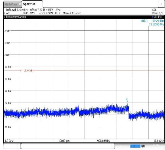
Band26(824-849)-5MHz-16QAM-26915-1RB#0-Range2:1000~10000MHz
