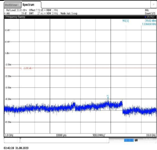
Band26(814-824)-3MHz-QPSK-26705-1RB#0- Range2:1000~10000MHz
