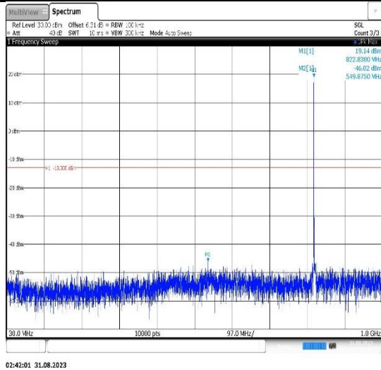
Band26(814-824)-1.4MHz-16QAM-26697-1RB#0-Range1:30~1000MHz
