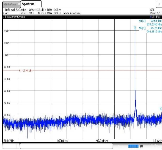
Band26(824-849)-5MHz-16QAM-26915-1RB#0-Range1:30~1000MHz
