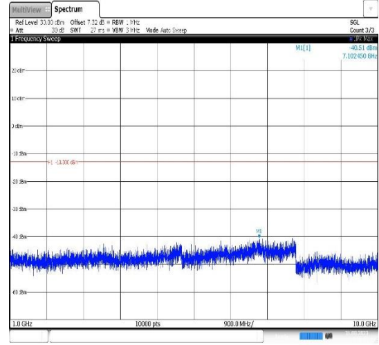
Band26(824-849)-1.4MHz-16QAM-26915-1RB#0- Range2:1000~10000MHz
