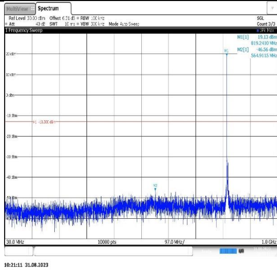
Band26(814-824)-5MHz-16QAM-26715-1RB#0-Range1:30~1000MHz
