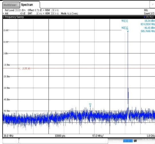
Band26(824-849)-3MHz-16QAM-26915-1RB#0-Range1:30~1000MHz
