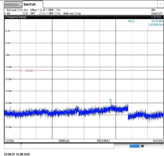
Band26(824-849)-5MHz-16QAM-26815-1RB#0-Range2:1000~10000MHz
