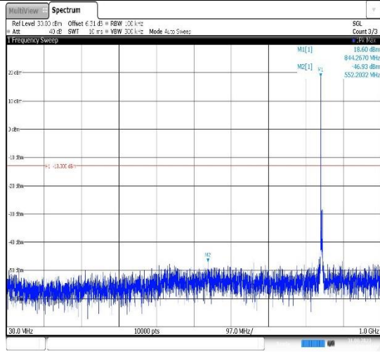
Band26(824-849)-5MHz-16QAM-27015-1RB#0-Range1:30~1000MHz
