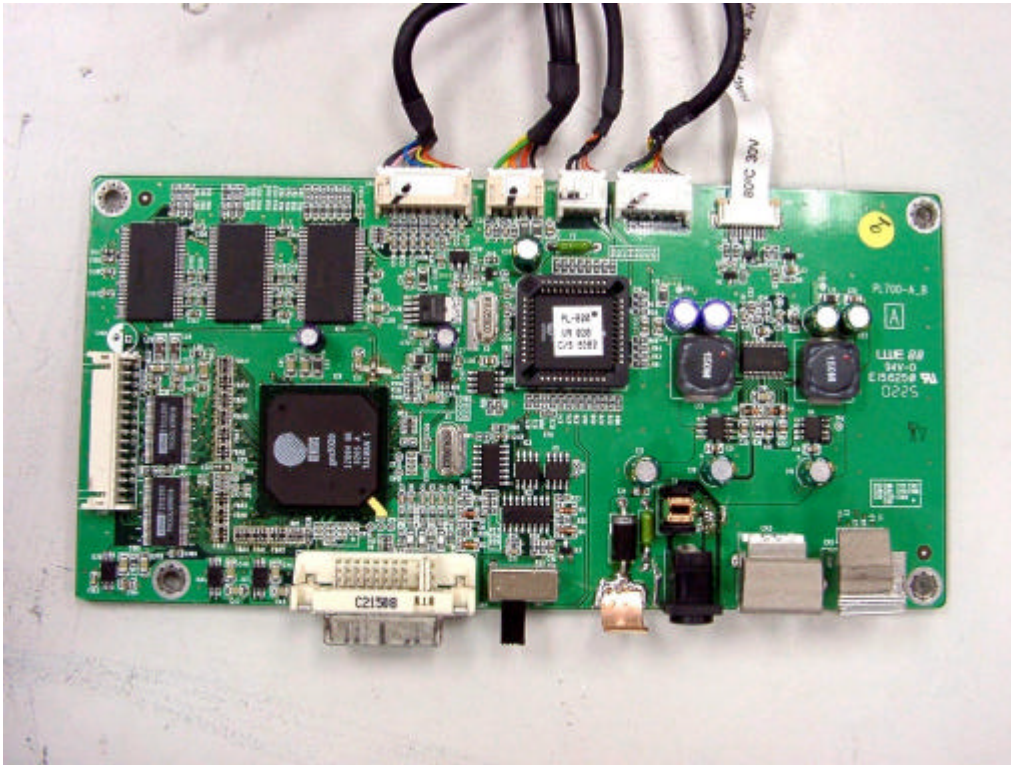
13. Front view of PCB 1 (Monitor)
