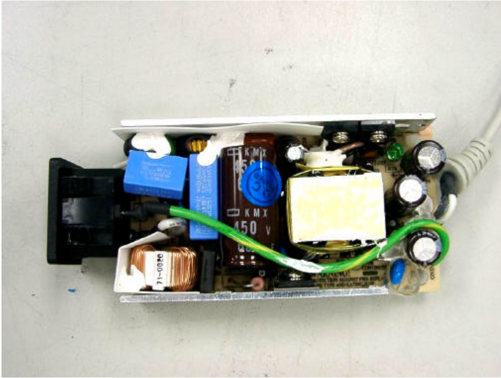
29. Front view of PCB 8 (Adaptor)
