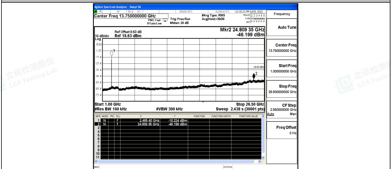
11N40SISO_Ant0_2422_0~Reference
