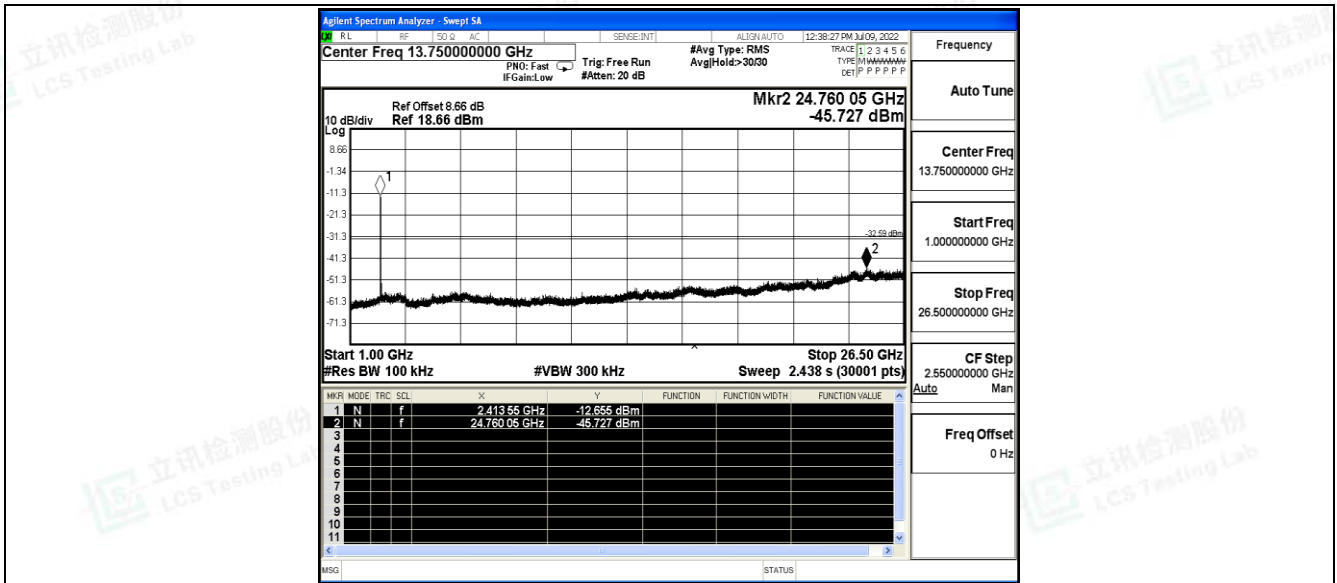
11N40SISO_Ant0_2437_0~Reference
