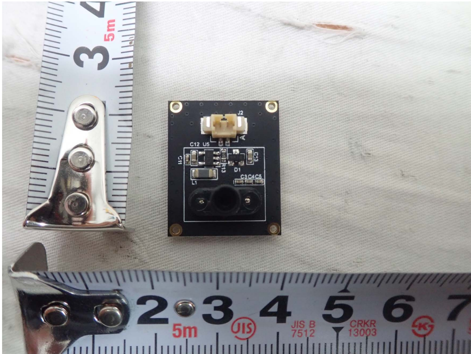
Finger print Module Board REAR
