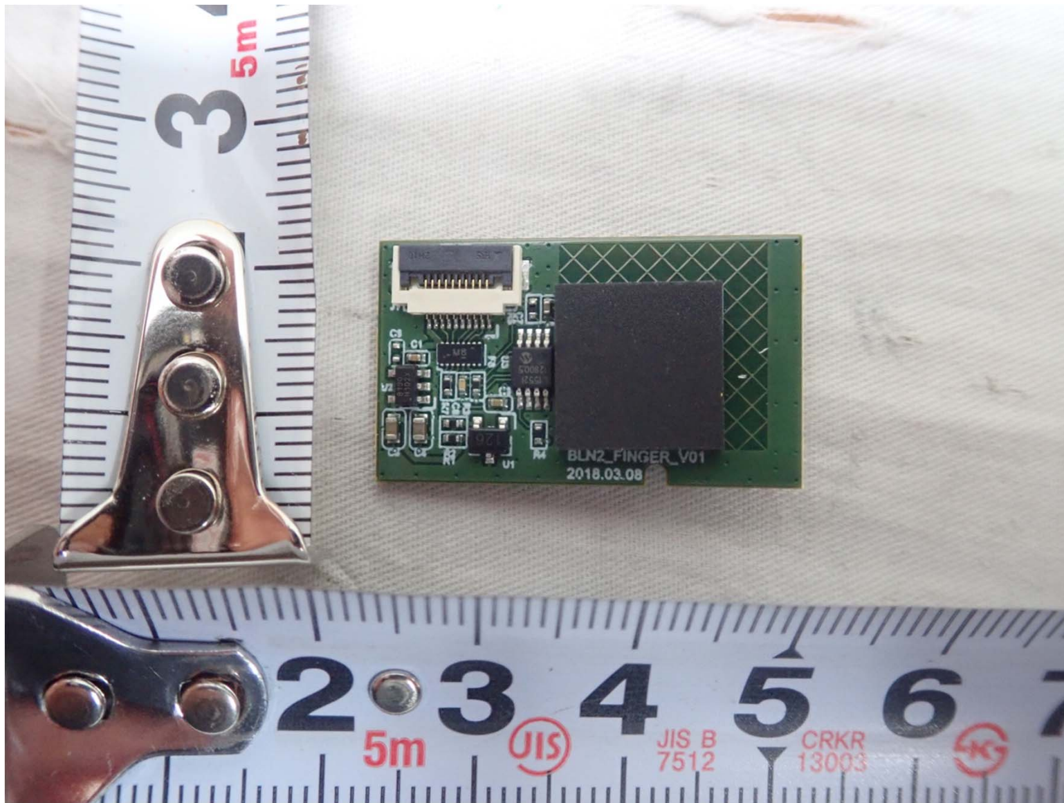
Finger print board FRONT
