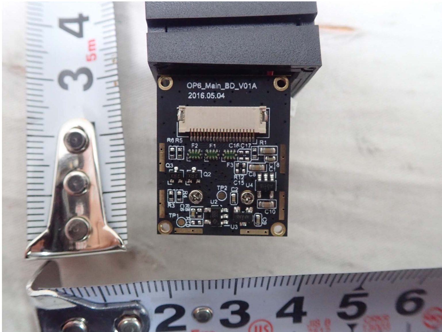
Finger print Module Board FRONT
