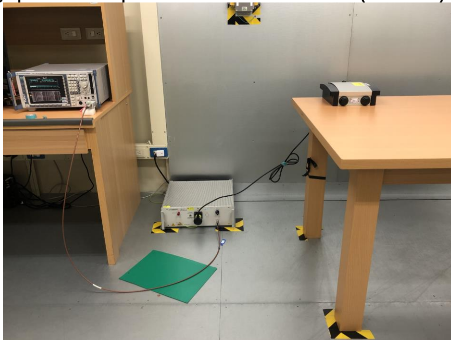
Photograph 6: Test Setup for Mains Conducted Emissions (Front View)
