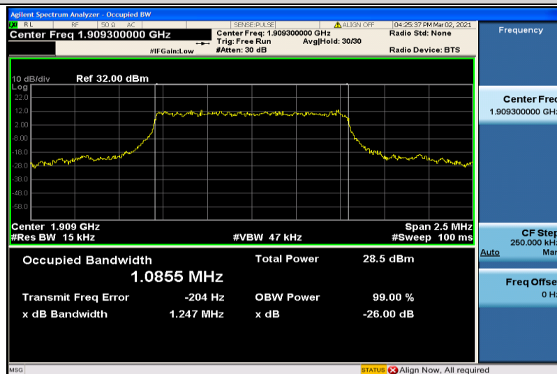
Band2-1.4MHz-QPSK-19193-6RB#0-1.0855
