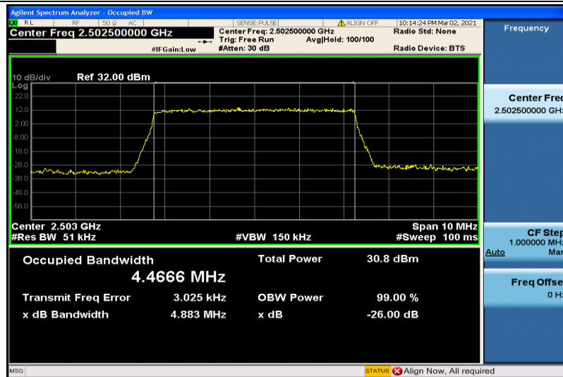
Band7-5MHz-QPSK-20775-25RB#0-4.4666
