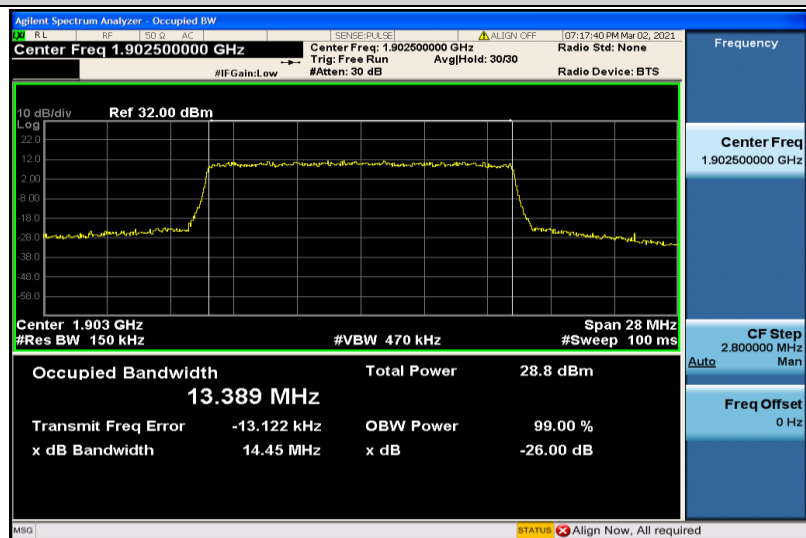
Band2-15MHz-16QAM-19125-75RB#0-13.389
