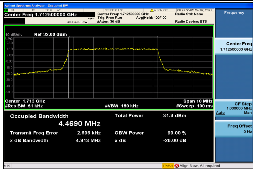
Band4-5MHz-QPSK-19975-25RB#0-4.4690
