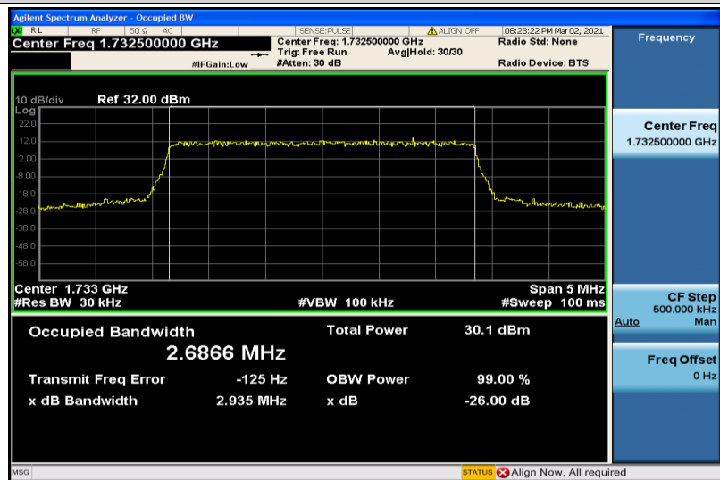
Band4-3MHz-QPSK-20175-15RB#0-2.6866
