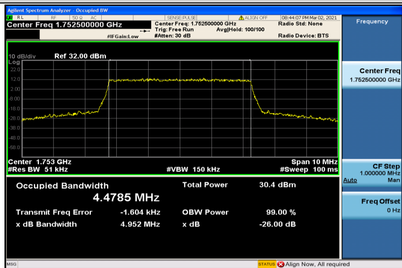
Band4-5MHz-QPSK-20375-25RB#0-4.4785
