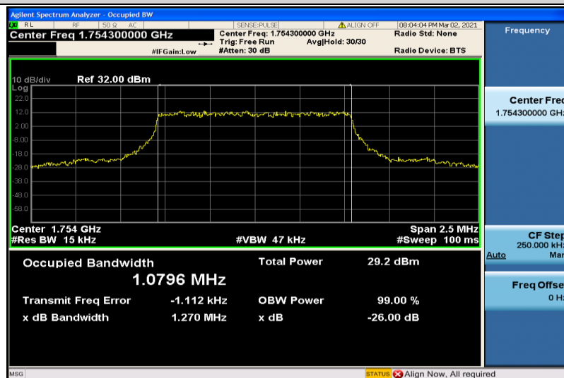
Band4-1.4MHz-QPSK-20393-6RB#0-1.0796
