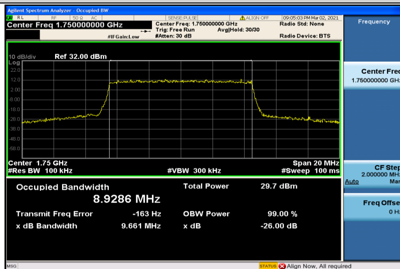
Band4-10MHz-16QAM-20350-50RB#0-8.9286
