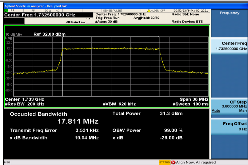
Band4-20MHz-QPSK-20175-100RB#0-17.811
