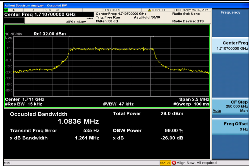
Band4-1.4MHz-16QAM-19957-6RB#0-1.0836
