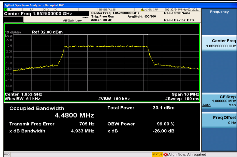
Band2-5MHz-QPSK-18625-25RB#0-4.4800
