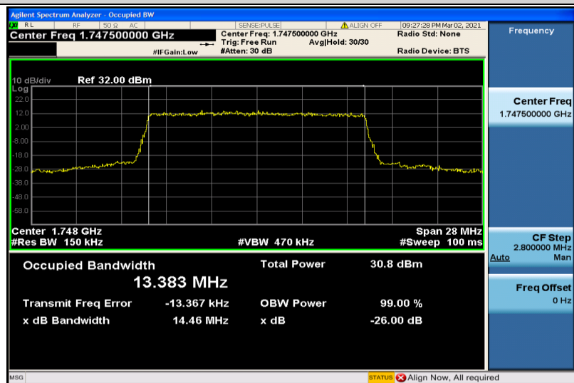
Band4-15MHz-QPSK-20325-75RB#0-13.383
