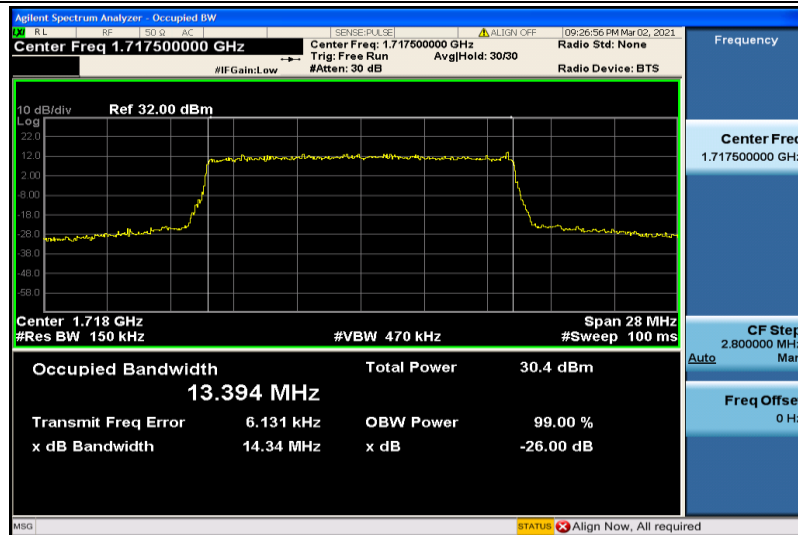
Band4-15MHz-16QAM-20025-75RB#0-13.394
