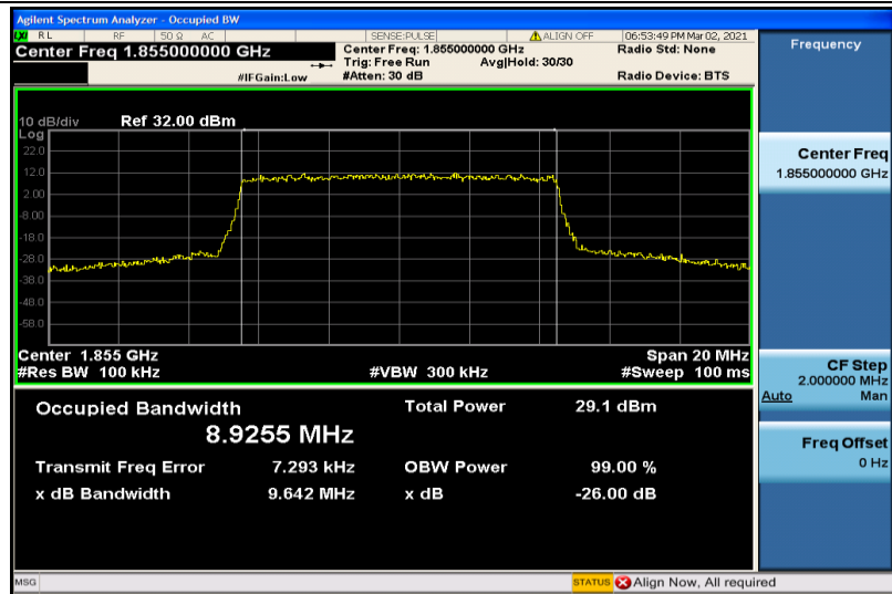
Band2-10MHz-16QAM-18650-50RB#0-8.9255
