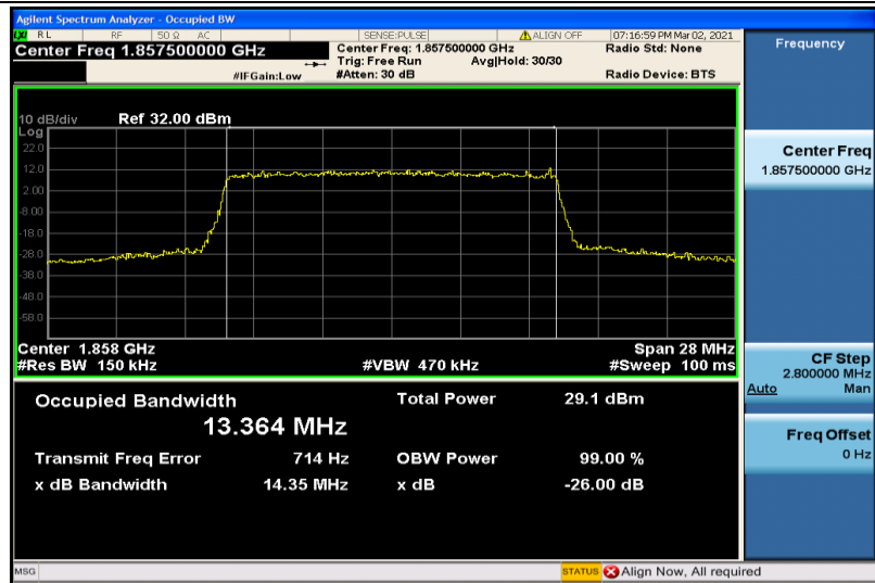
Band2-15MHz-16QAM-18675-75RB#0-13.364
