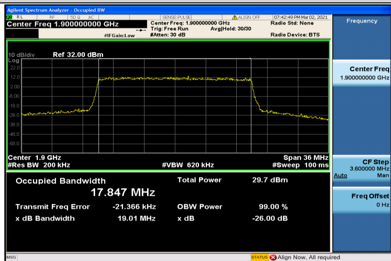
Band2-20MHz-QPSK-19100-100RB#0-17.847
