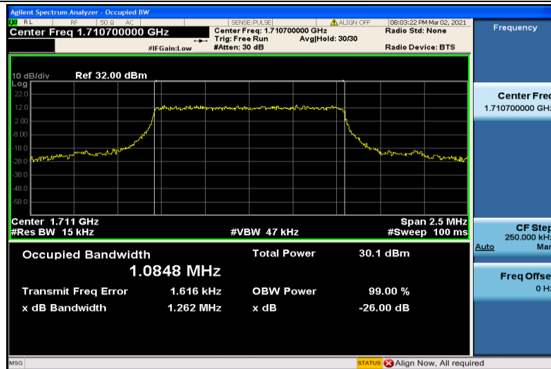
Band4-1.4MHz-QPSK-19957-6RB#0-1.0848
