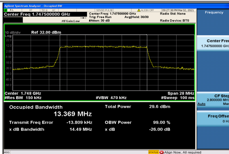
Band4-15MHz-16QAM-20325-75RB#0-13.369
