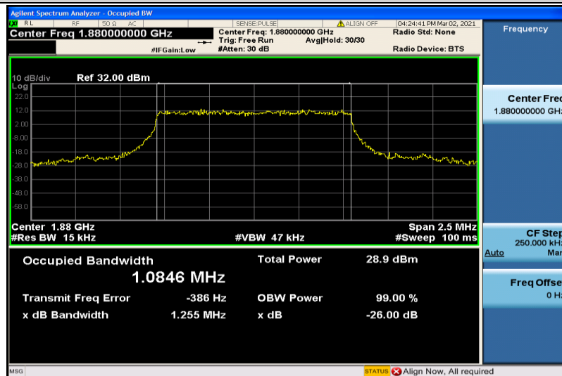
Band2-1.4MHz-QPSK-18900-6RB#0-1.0846
