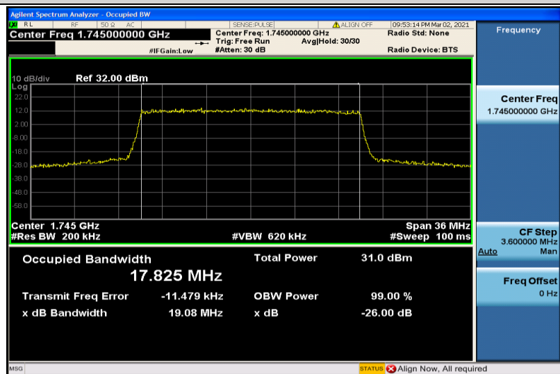
Band4-20MHz-QPSK-20300-100RB#0-17.825
