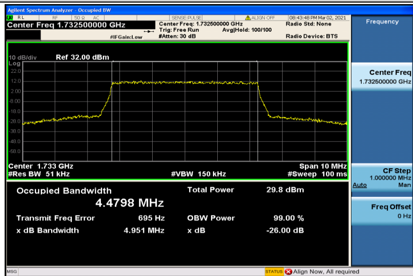
Band4-5MHz-16QAM-20175-25RB#0-4.4798
