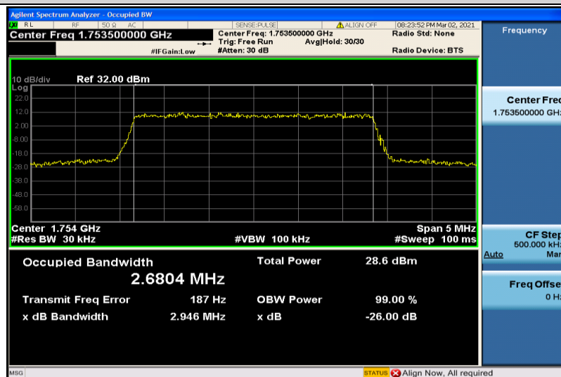
Band4-3MHz-16QAM-20385-15RB#0-2.6804
