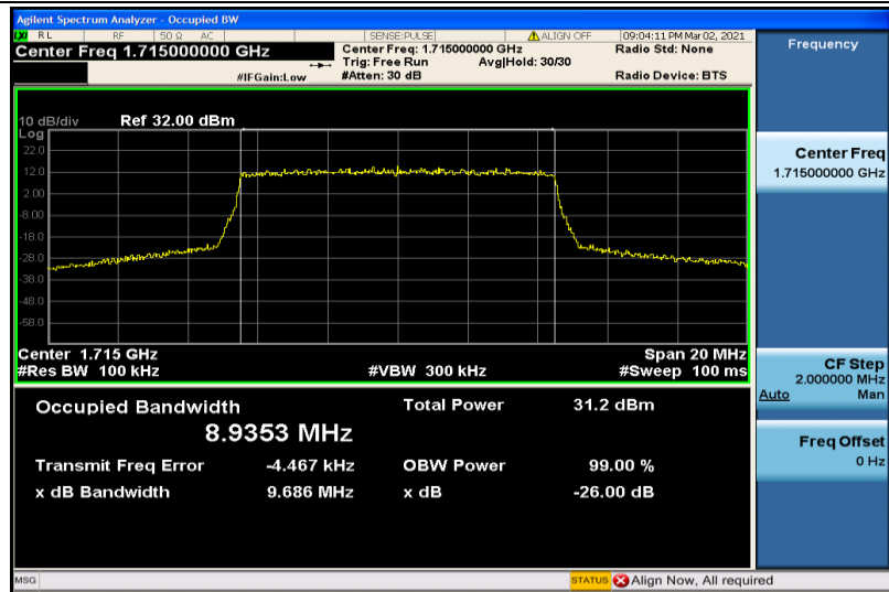
Band4-10MHz-QPSK-20000-50RB#0-8.9353
