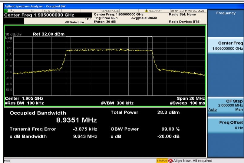
Band2-10MHz-16QAM-19150-50RB#0-8.9351
