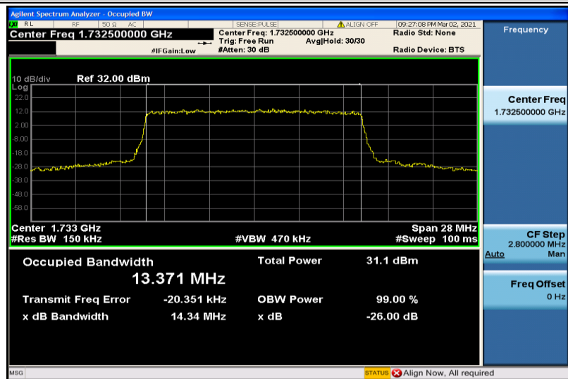
Band4-15MHz-QPSK-20175-75RB#0-13.371
