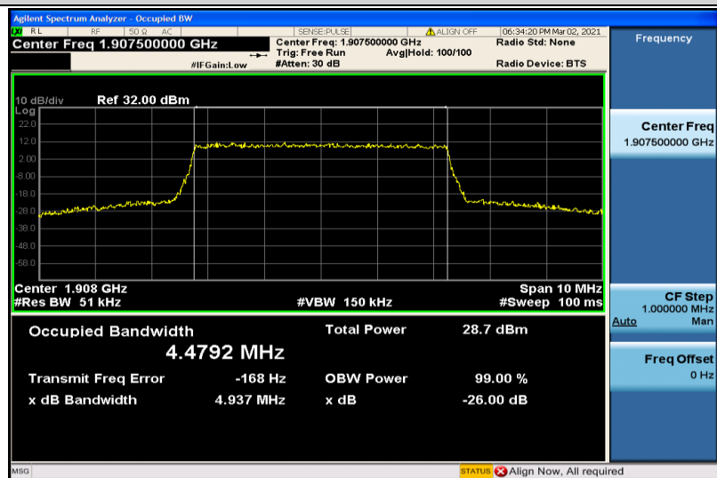
Band2-5MHz-16QAM-19175-25RB#0-4.4792
