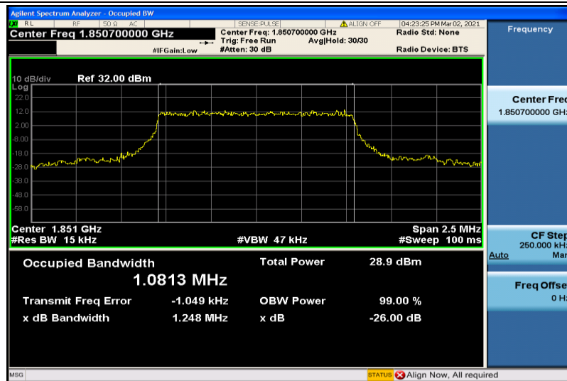
Band2-1.4MHz-QPSK-18607-6RB#0-1.0813
