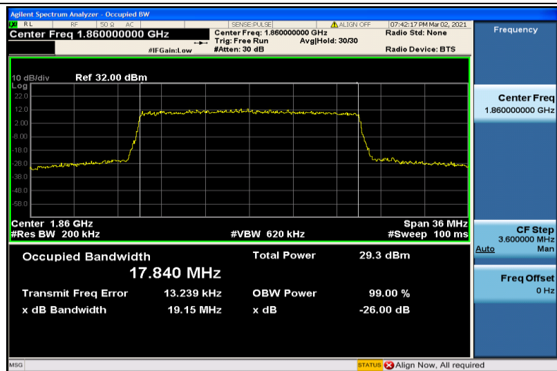
Band2-20MHz-16QAM-18700-100RB#0-17.840
