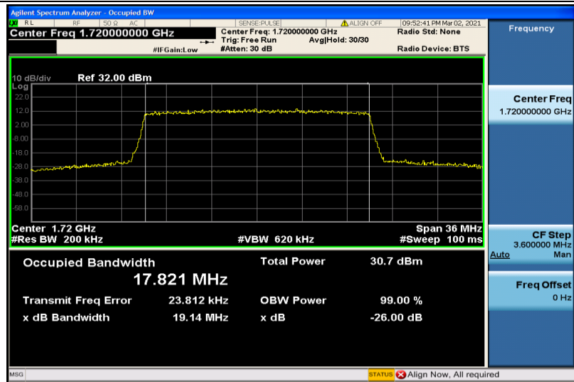
Band4-20MHz-16QAM-20050-100RB#0-17.821
