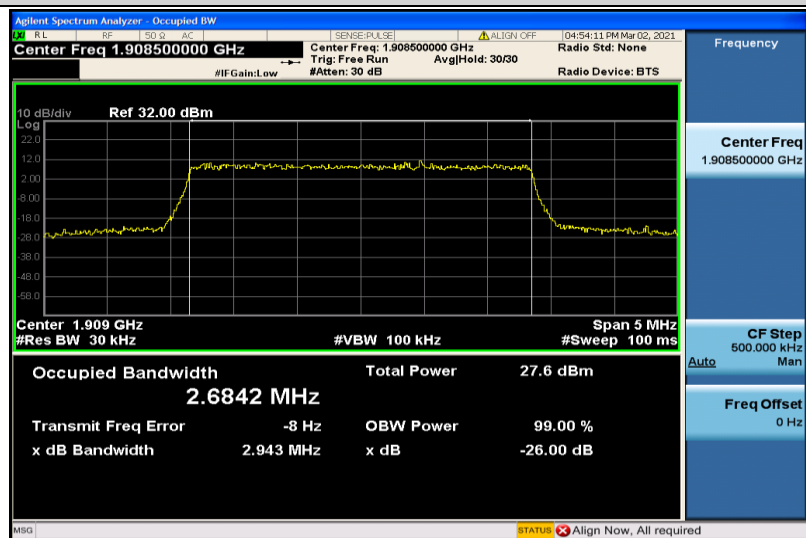
Band2-3MHz-16QAM-19185-15RB#0-2.6842
