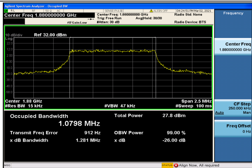
Band2-1.4MHz-16QAM-18900-6RB#0-1.0798
