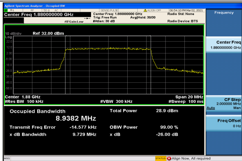
Band2-10MHz-16QAM-18900-50RB#0-8.9382
