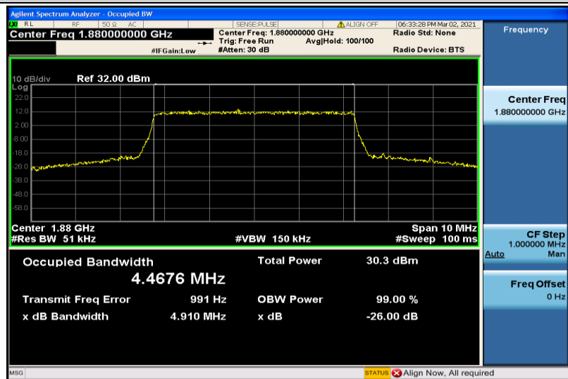
Band2-5MHz-QPSK-18900-25RB#0-4.4676
