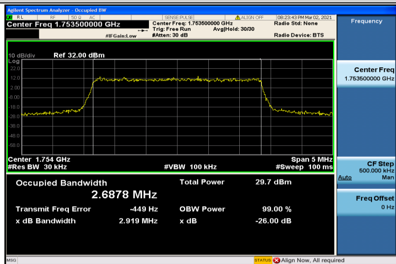
Band4-3MHz-QPSK-20385-15RB#0-2.6878
