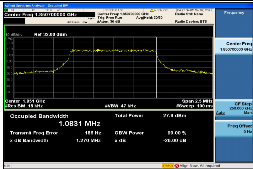
Band2-1.4MHz-16QAM-18607-6RB#0-1.0831
