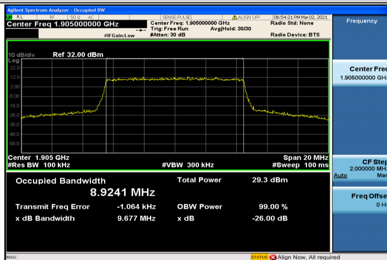
Band2-10MHz-QPSK-19150-50RB#0-8.9241
