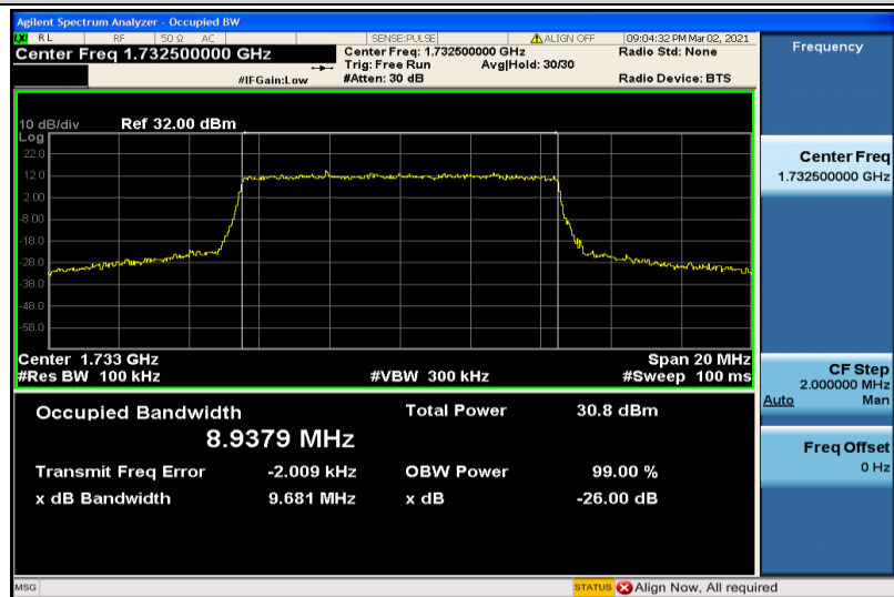
Band4-10MHz-QPSK-20175-50RB#0-8.9379
