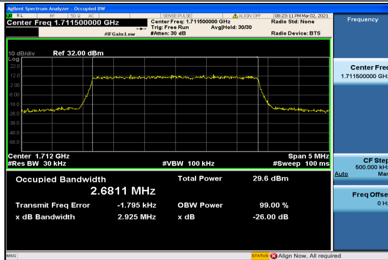
Band4-3MHz-16QAM-19965-15RB#0-2.6811
