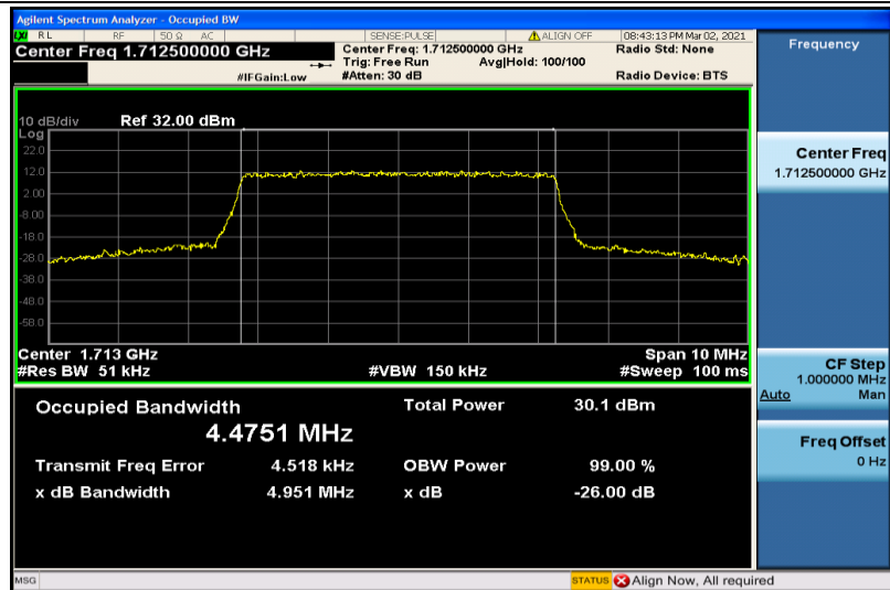
Band4-5MHz-16QAM-19975-25RB#0-4.4751
