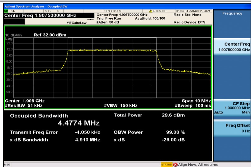
Band2-5MHz-QPSK-19175-25RB#0-4.4774
