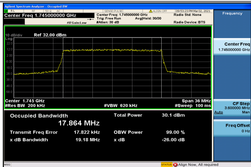
Band4-20MHz-16QAM-20300-100RB#0-17.864
