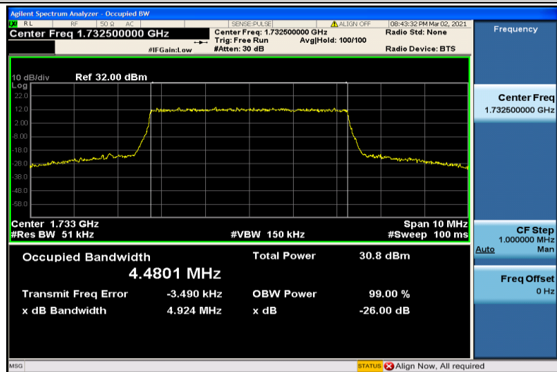
Band4-5MHz-QPSK-20175-25RB#0-4.4801
