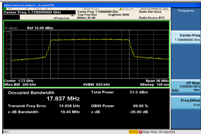
Band4-20MHz-QPSK-20050-100RB#0-17.837
