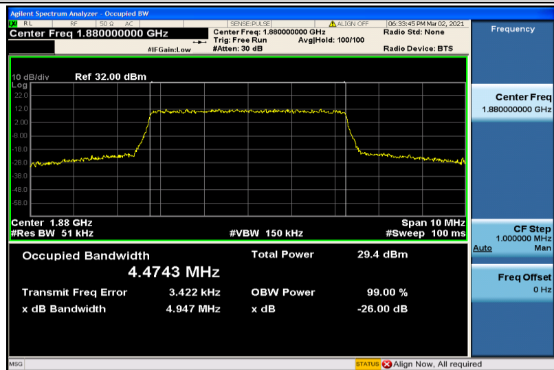
Band2-5MHz-16QAM-18900-25RB#0-4.4743
