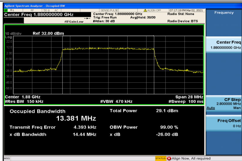
Band2-15MHz-16QAM-18900-75RB#0-13.381
