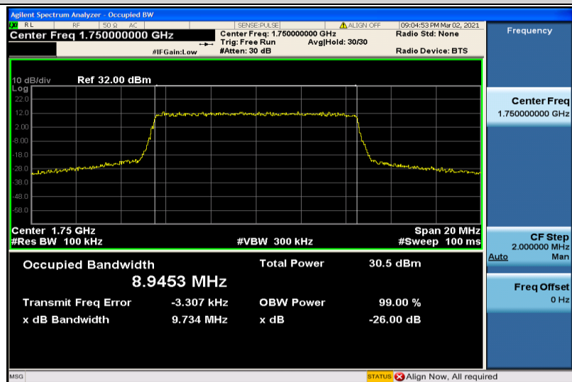
Band4-10MHz-QPSK-20350-50RB#0-8.9453
