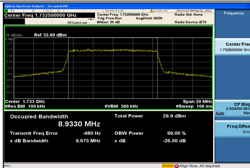
Band4-10MHz-16QAM-20175-50RB#0-8.9330
