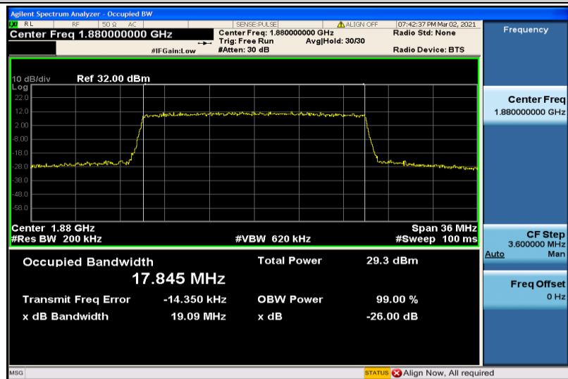
Band2-20MHz-16QAM-18900-100RB#0-17.845
