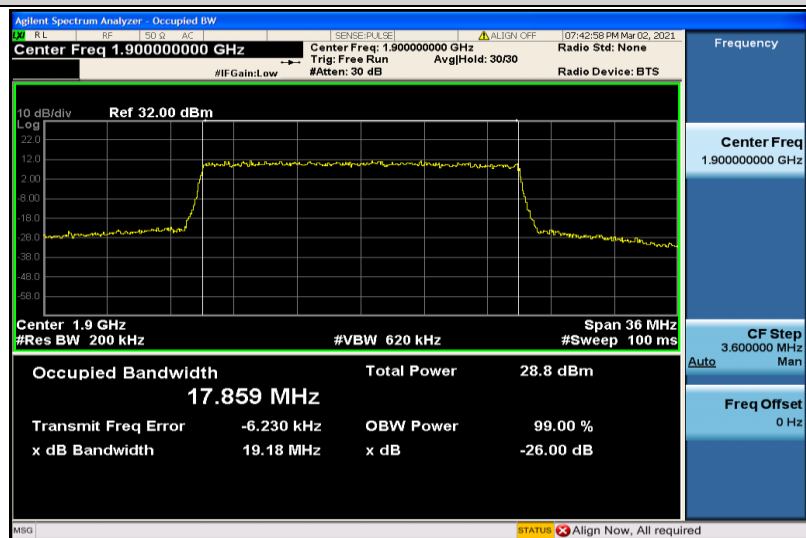
Band2-20MHz-16QAM-19100-100RB#0-17.859
