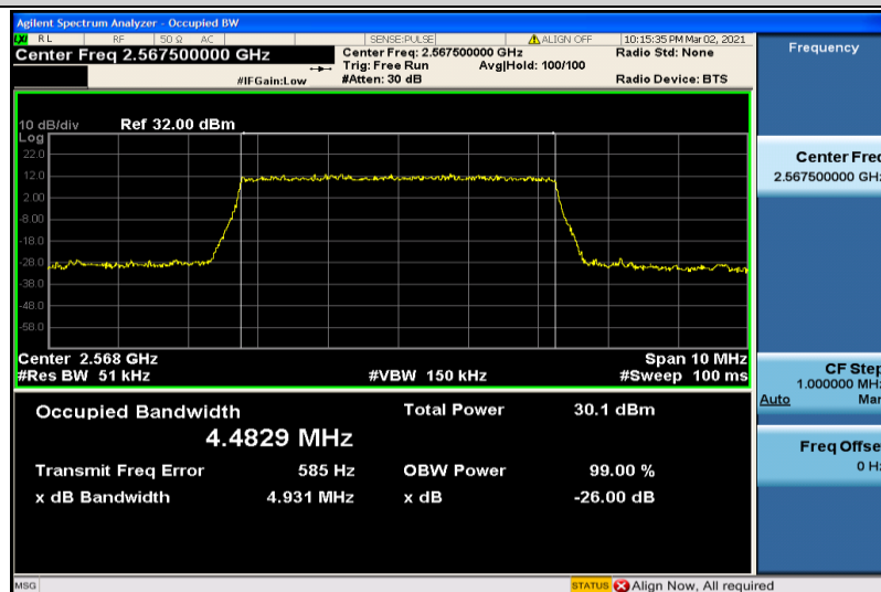
Band7-5MHz-QPSK-21425-25RB#0-4.4829
