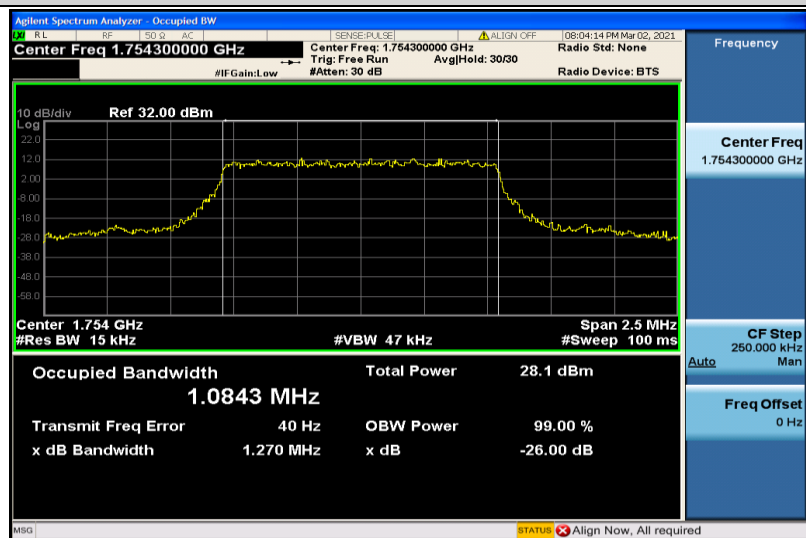
Band4-1.4MHz-16QAM-20393-6RB#0-1.0843
