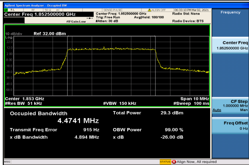
Band2-5MHz-16QAM-18625-25RB#0-4.4741
