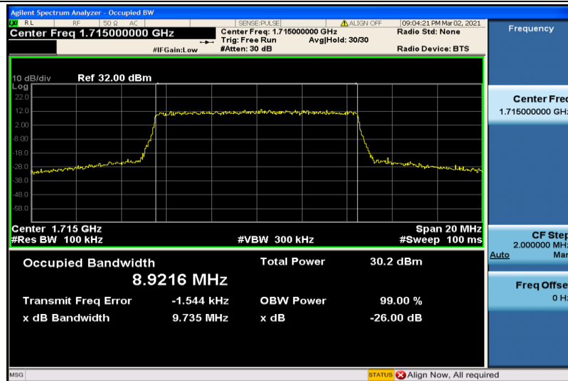
Band4-10MHz-16QAM-20000-50RB#0-8.9216
