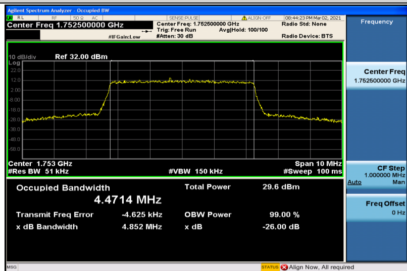
Band4-5MHz-16QAM-20375-25RB#0-4.4714
