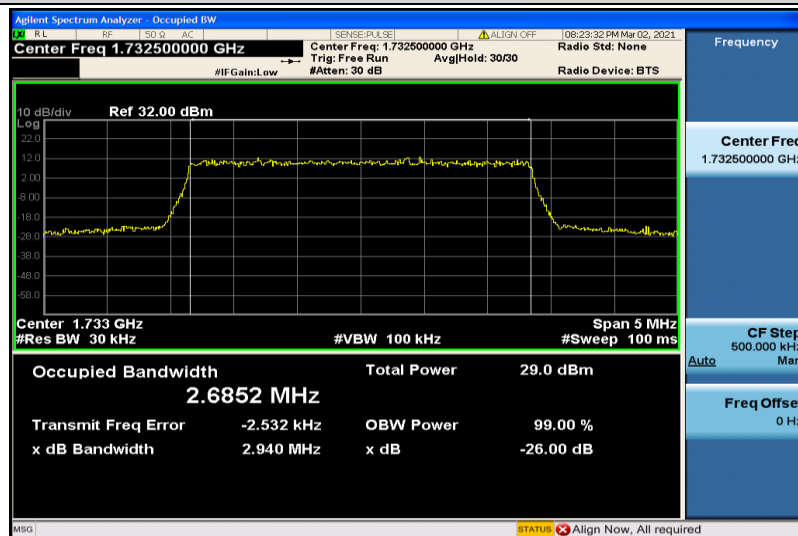
Band4-3MHz-16QAM-20175-15RB#0-2.6852
