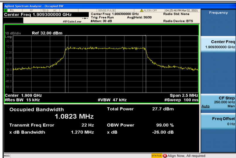
Band2-1.4MHz-16QAM-19193-6RB#0-1.0823
