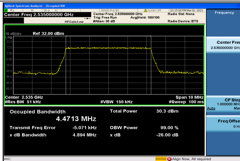
Band7-5MHz-QPSK-21100-25RB#0-4.4713
