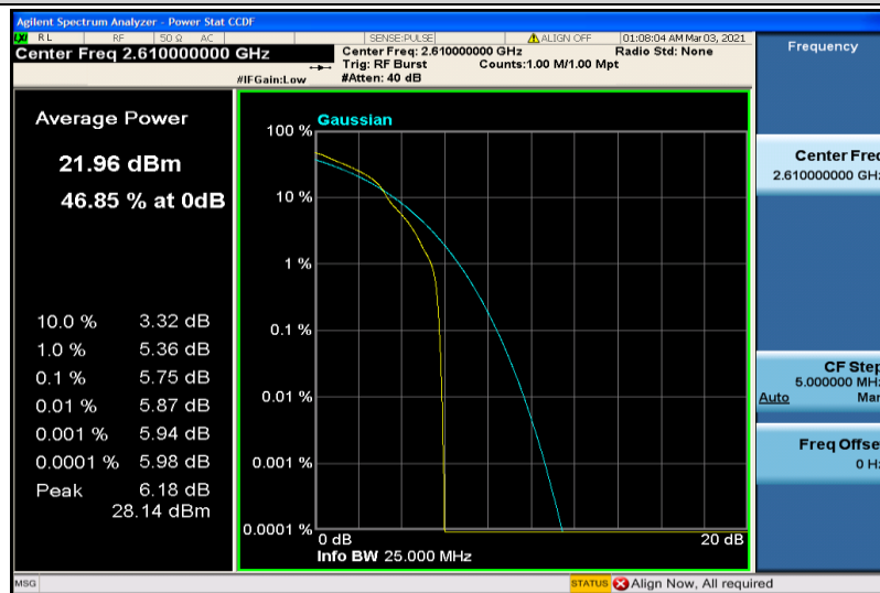
Band38-20MHz-16QAM-38150-1RB#0
