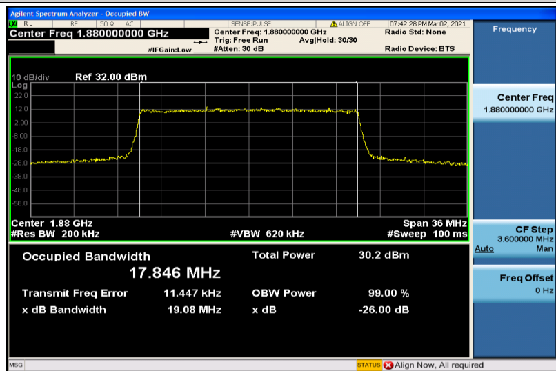
Band2-20MHz-QPSK-18900-100RB#0-17.846
