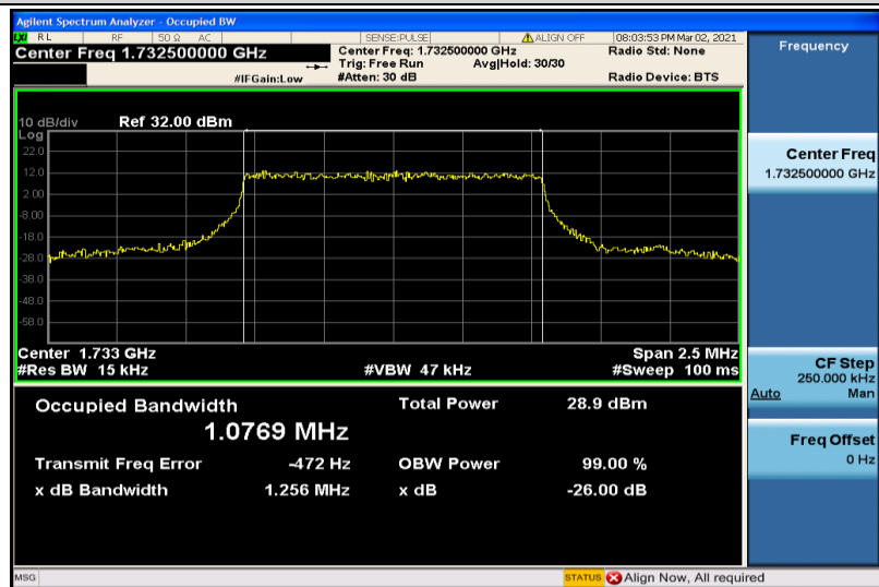
Band4-1.4MHz-16QAM-20175-6RB#0-1.0769
