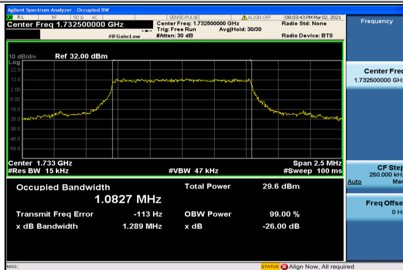
Band4-1.4MHz-QPSK-20175-6RB#0-1.0827
