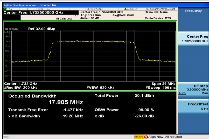
Band4-20MHz-16QAM-20175-100RB#0-17.805
