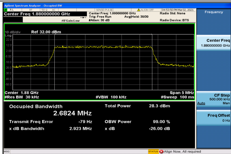
Band2-3MHz-16QAM-18900-15RB#0-2.6824
