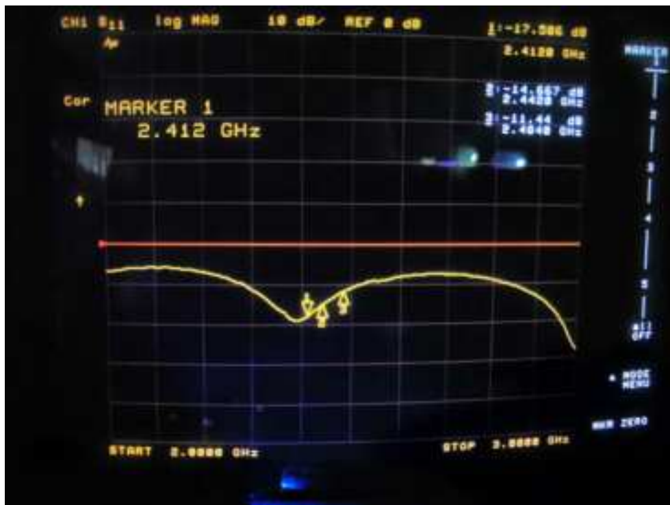
FIG 2 EWN-8822CSS3AH 2.4G Path A
