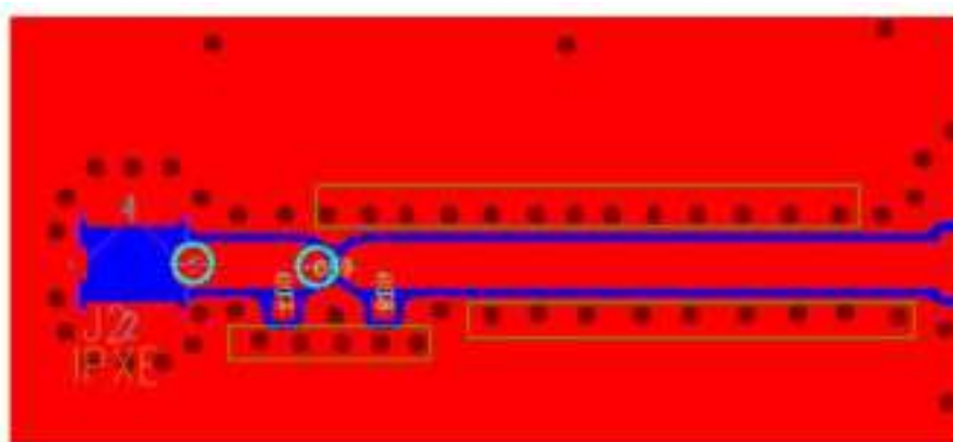
FIG 20 The RF line Layout
