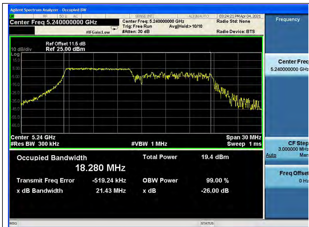
(Channel 48, 5240MHz, 802.11ax (HEW20) RU106)
