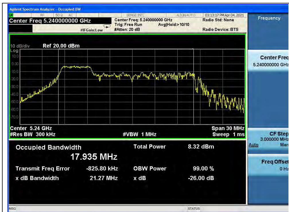
(Channel 48, 5240MHz, 802.11ax (HEW20) RU52)
