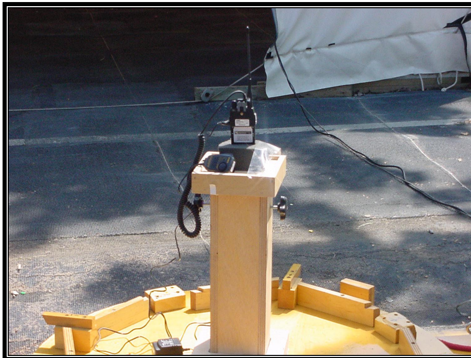
PHOTOGRAPH 4: RADIATED TEST CONFIGURATION (REAR VIEW)
