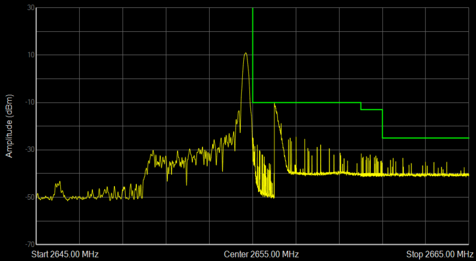
Band41(2555-2655) QPSK BW=5MHz Channel=41215 RB Size=1 Position=#Max
