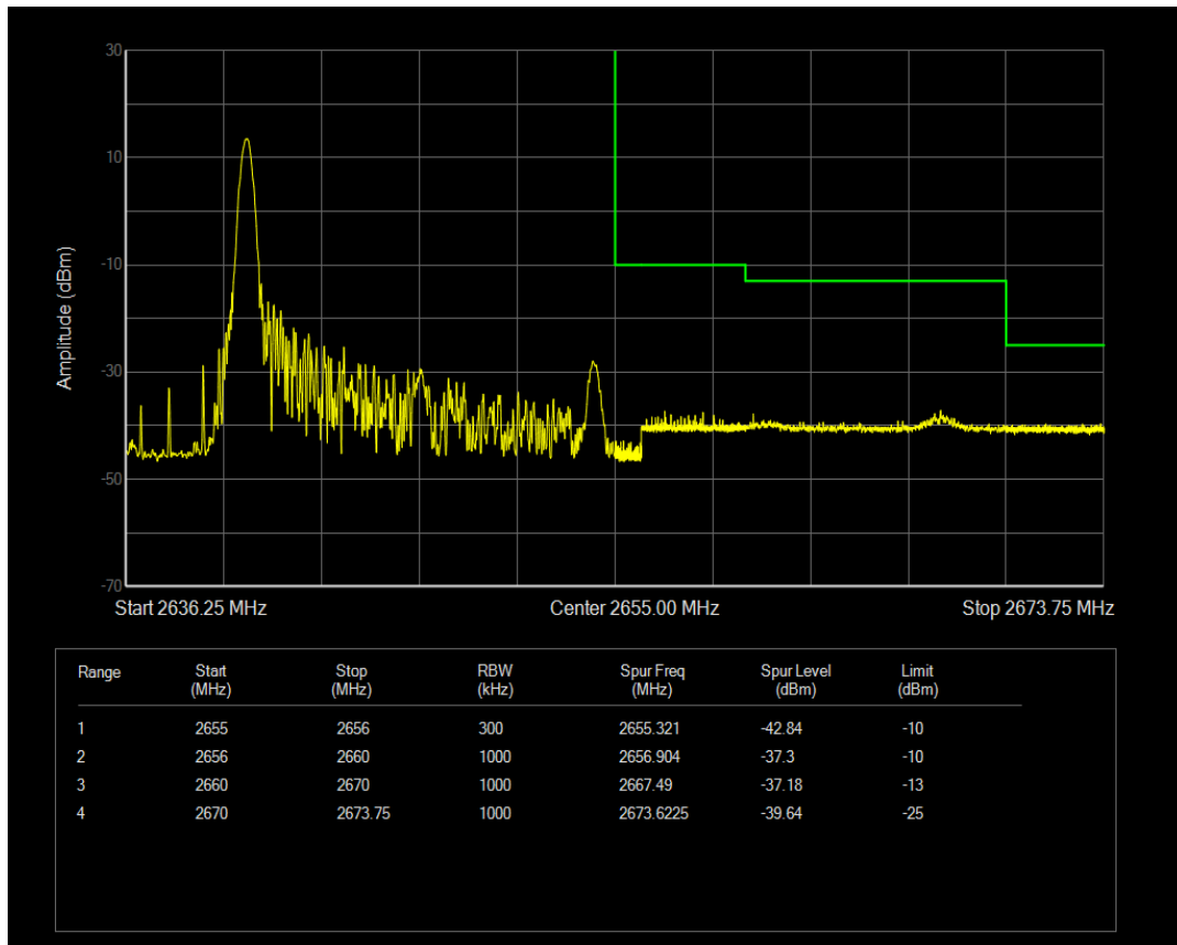
Band41(2555-2655) 16QAM BW=15MHz Channel=41165 RB Size=1 Position=#Max
