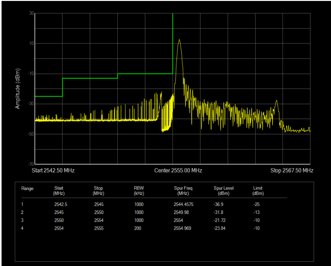
Band41(2555-2655) 16QAM BW=10MHz Channel=40290 RB Size=1 Position=#Max
