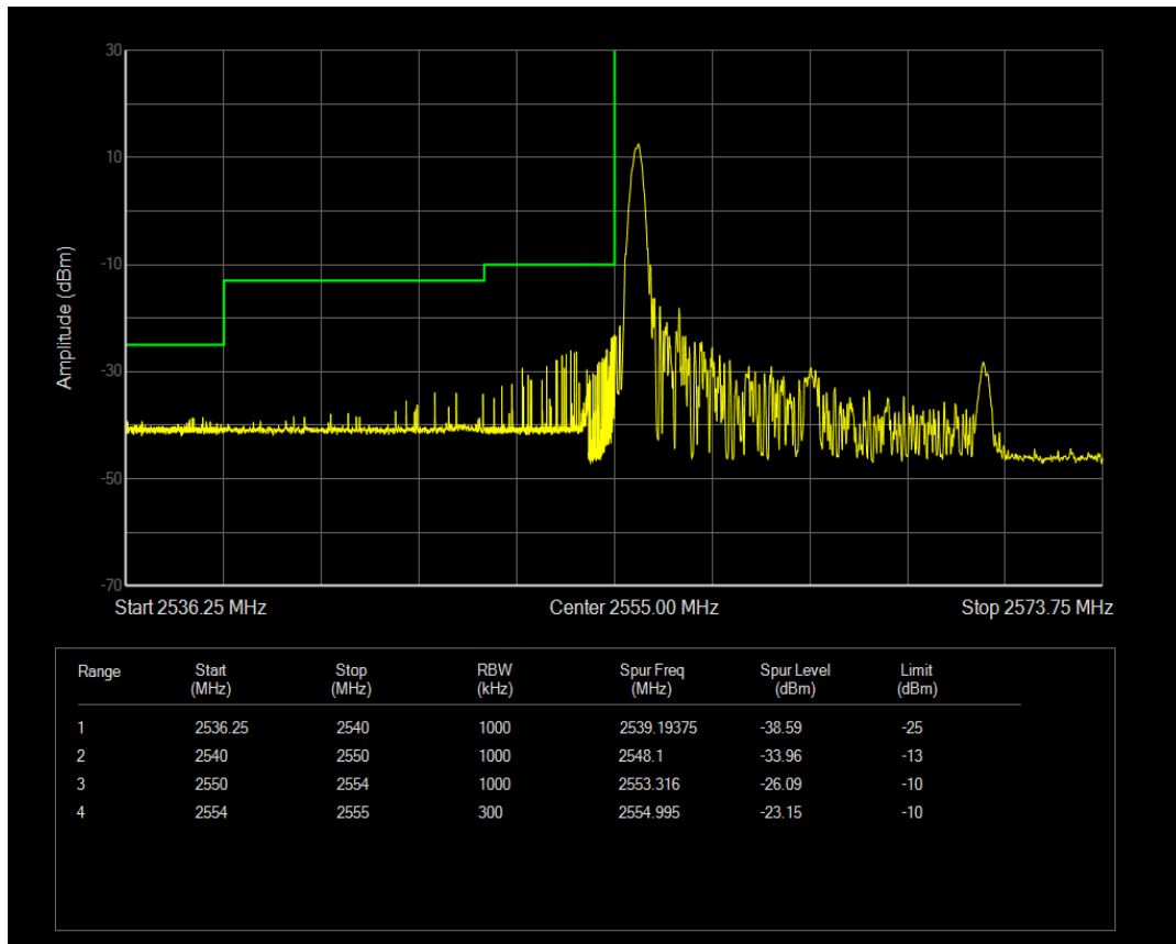
Band41(2555-2655) 16QAM BW=15MHz Channel=40315 RB Size=1 Position=#Max
