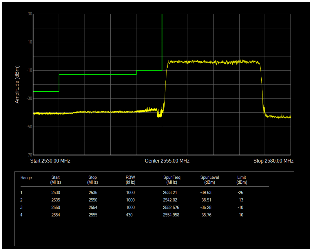
Band41(2555-2655) 16QAM BW=20MHz Channel=40340 RB Size=1 Position=#0
