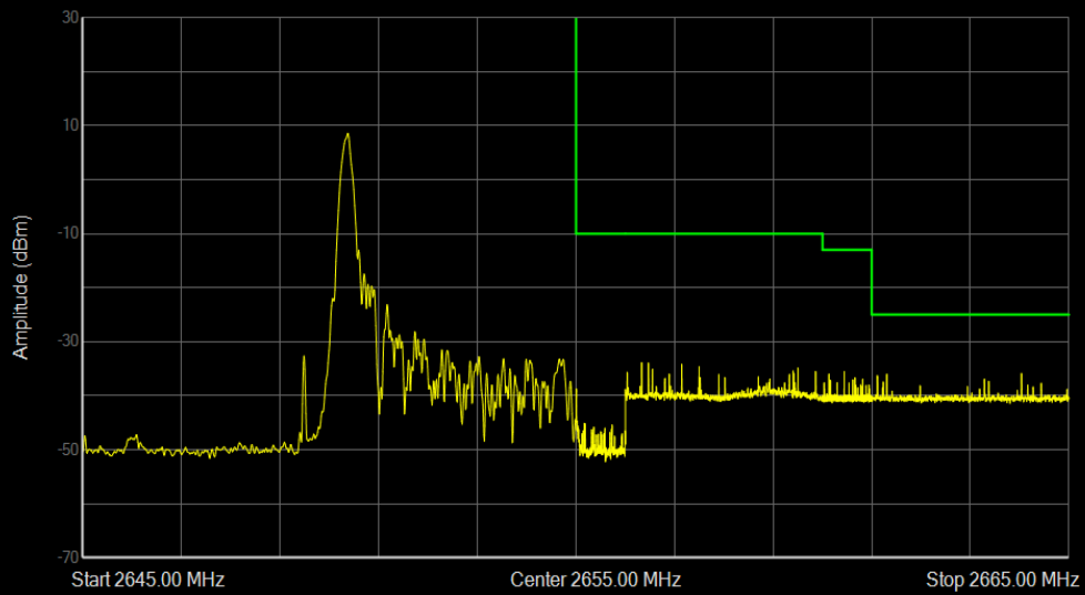
Band41(2555-2655) 16QAM BW=5MHz Channel=41215 RB Size=1 Position=#0
