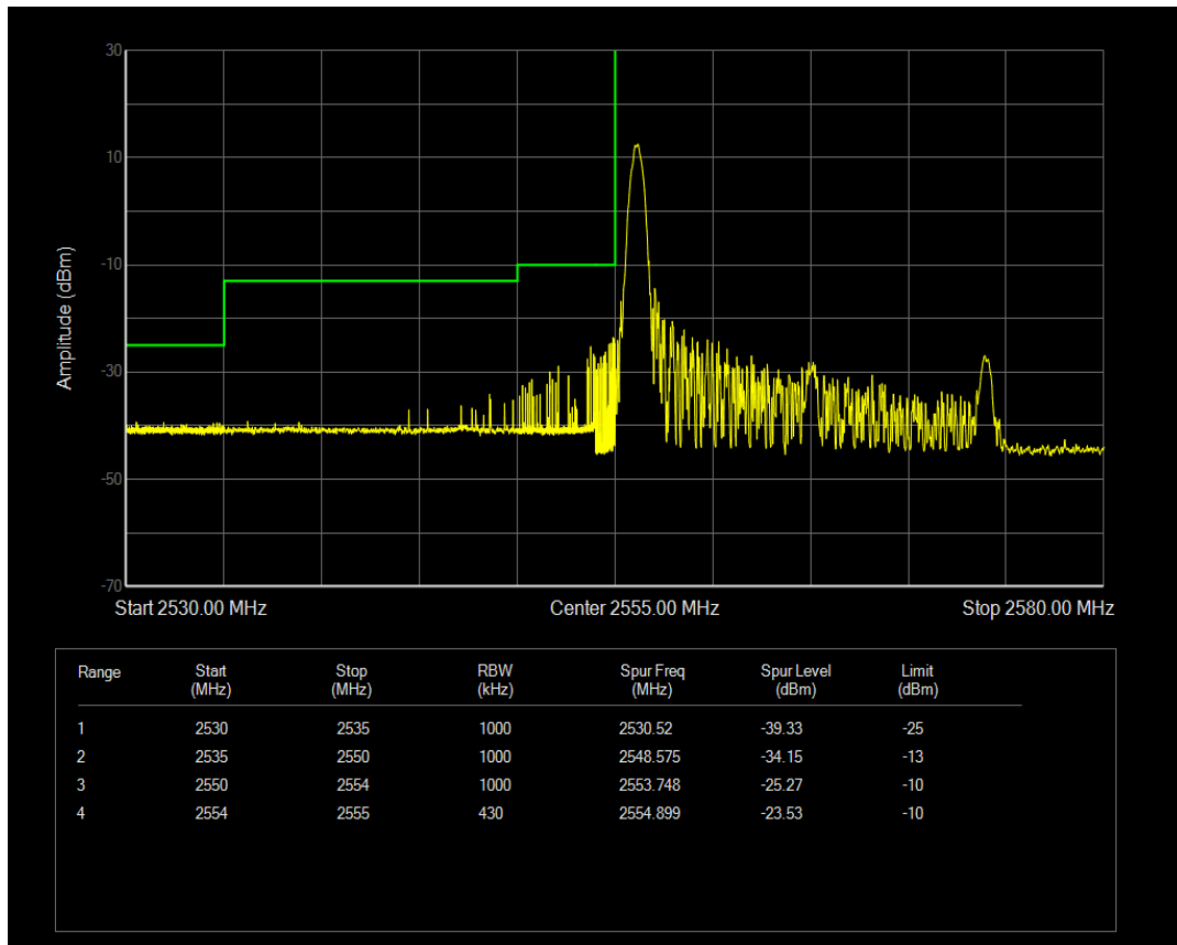
Band41(2555-2655) 16QAM BW=20MHz Channel=40340 RB Size=1 Position=#Max
