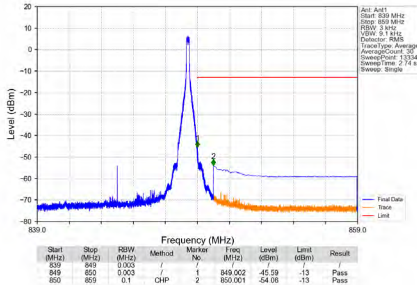
Band5_10MHz_16QAM_HCH_844MHz_RB_1_49_NTNV
