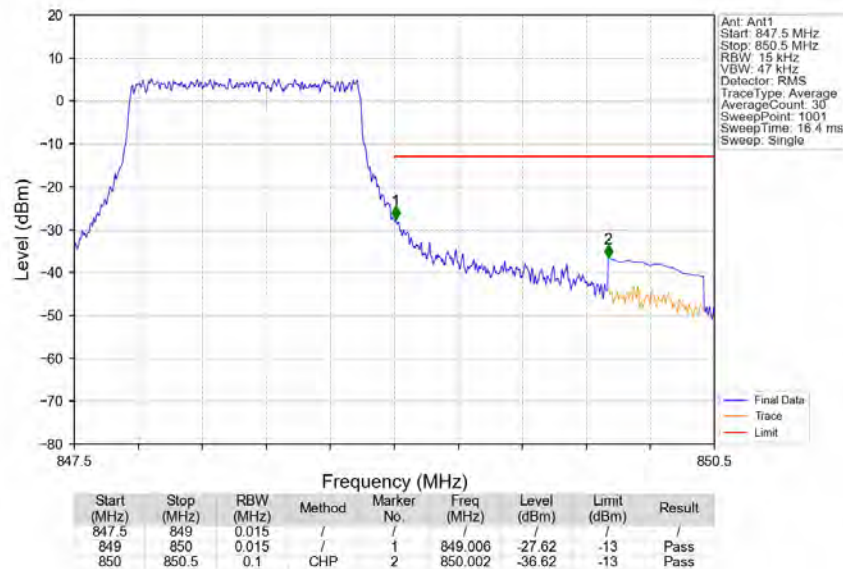
Band5_1.4MHz_QPSK_HCH_848.3MHz_RB_6_0_NTNV
