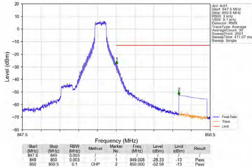
Band5 1.4MHz 16QAM HCH 848.3MHz RB 1 5 NTNV
