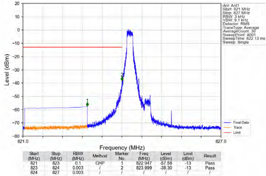
Band5_3MHz_64QAM_LCH_825.5MHz_RB_1_0_NTNV
