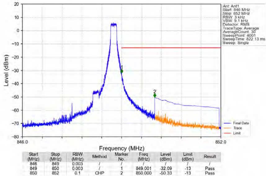
Band5_3MHz_16QAM_HCH_847.5MHz_RB_1_14_NTNV
