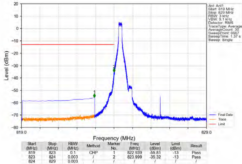
Band5_5MHz_64QAM_LCH_826.5MHz_RB_1_0_NTNV
