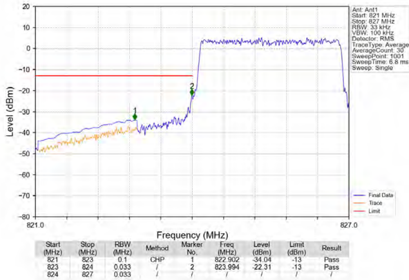
Band5_3MHz_QPSK_LCH_825.5MHz_RB_15_0_NTNV
