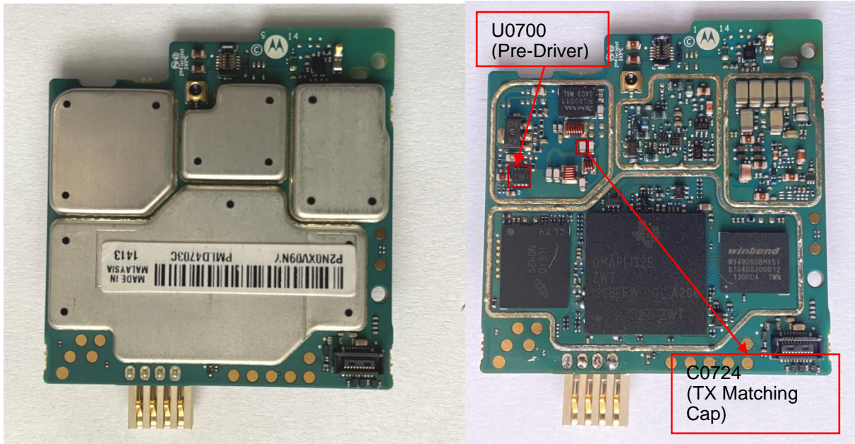
RF board with and without Shields (Bottom)
