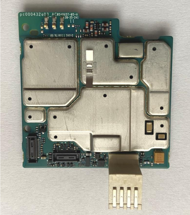
PCB board with chassis and housing (Top)
