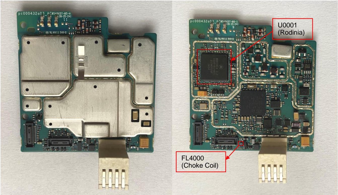
RF board with and without Shields (Top)
