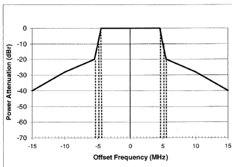
FIG. 12 Class A Transmit Spectrum Mask
