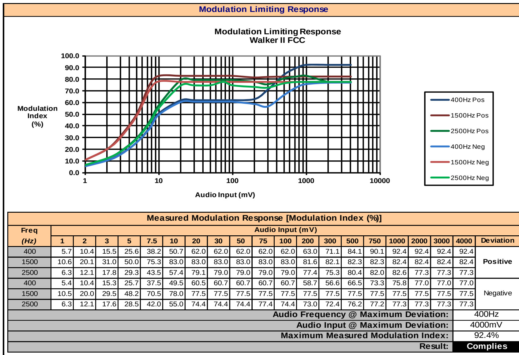
Plot 8.2 – Modulation Limiting Response
