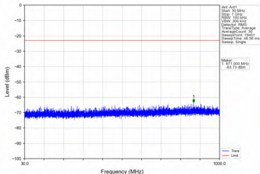
n25_30kHz_SISO_NTNV_10MHz_CP-OFDM QPSK_1855MHz_Edge_1RB_Left
