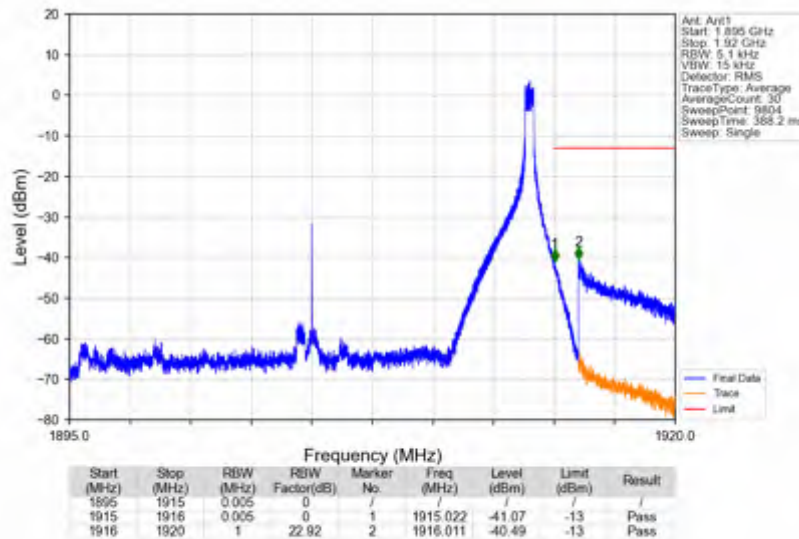
n25_30kHz_SISO_NTNV_20MHz_DFT-s-OFDM_QPSK_1905MHz_Edge_1RB_Right
