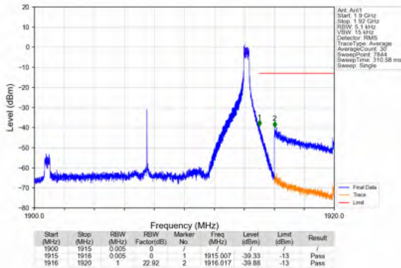
n25_30kHz_SISO_NTNV_15MHz_CP-OFDM QPSK_1907.5MHz_Edge_1RB_Right
