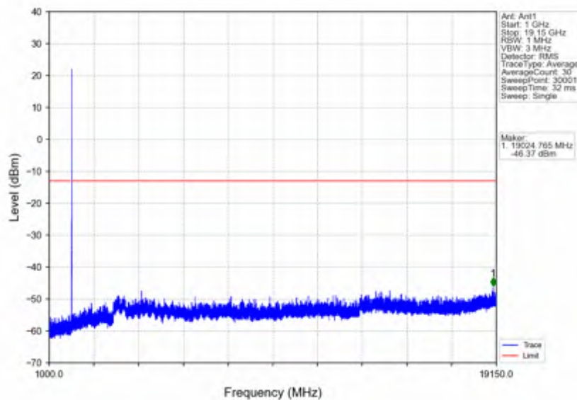
n25_30kHz_SISO_NTNV_10MHz_CP-OFDM QPSK_1910MHz_Outer_Full
