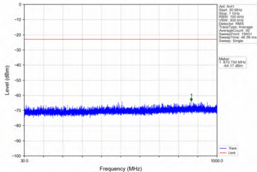
n25_30kHz_SISO_NTNV_15MHz_CP-OFDM_QPSK_1857.5MHz_Outer_Full
