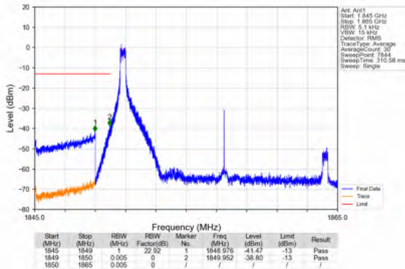
n25_30kHz_SISO_NTNV_15MHz_CP-OFDM_QPSK_1857.5MHz_Edge_1RB_Left
