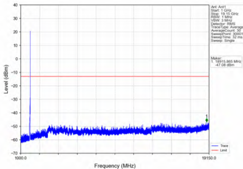
n25_15kHz_SISO_NTNV_40MHz_CP-OFDM QPSK_1895MHz_Outer_Full
