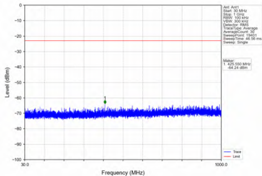
n25_15kHz_SISO_NTNV_40MHz_CP-OFDM QPSK_1895MHz_Inner_1RB_Right
