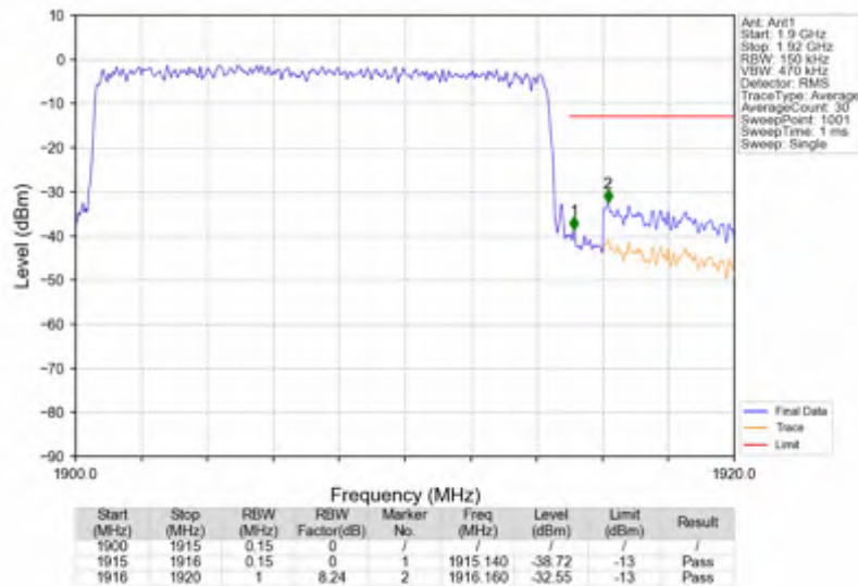
n25_30kHz_SISO_NTNV_15MHz_CP-OFDM QPSK_1907.5MHz_Outer_Full
