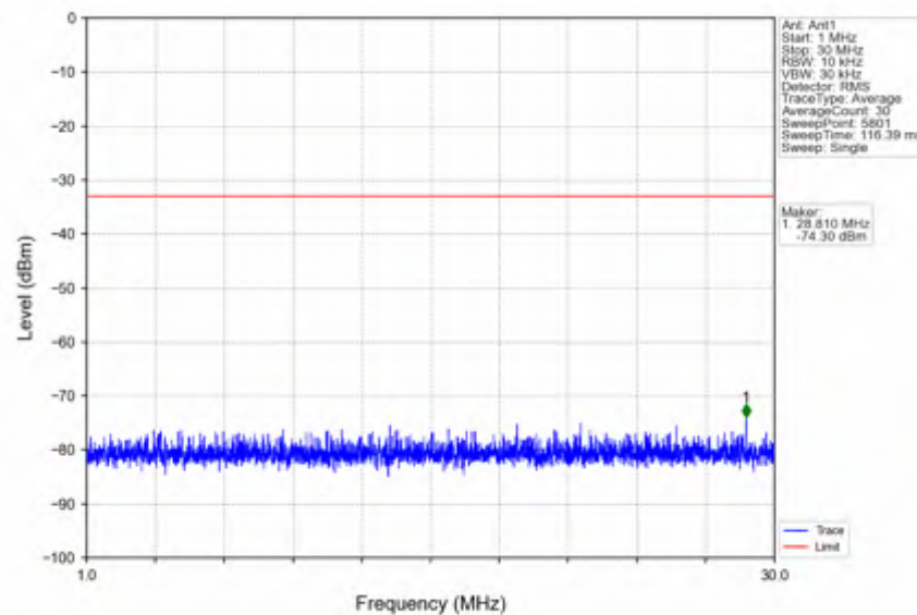
n25_30kHz_SISO_NTNV_20MHz_CP-OFDM QPSK_1905MHz_Edge_1RB_Right
