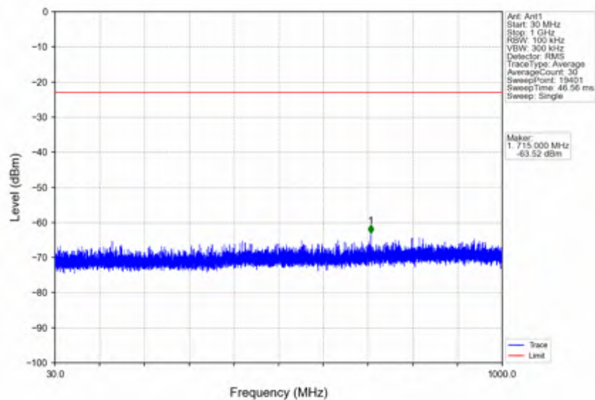
n25_30kHz_SISO_NTNV_15MHz_DFT-s-OFDM_QPSK_1907.5MHz_Edge_1RB_Right
