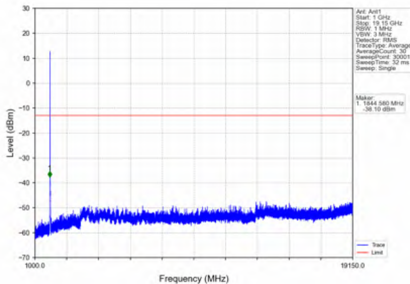
n25_30kHz_SISO_NTNV_15MHz_DFT-s-OFDM_QPSK_1857.5MHz_Inner_1RB_Left
