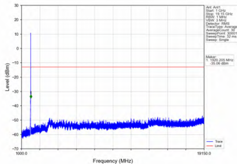
n25_30kHz_SISO_NTNV_15MHz_CP-OFDM QPSK_1907.5MHz_Outer_Full
