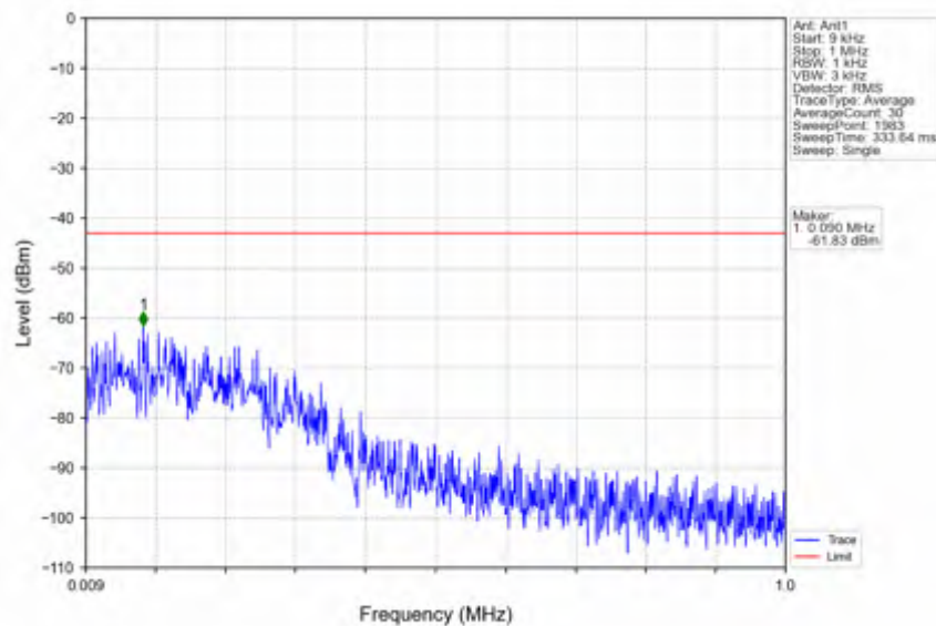
n25_30kHz_SISO_NTV_10MHz_CP-OFDM_QPSK_1882.5MHz_Edge_1RB_Left
