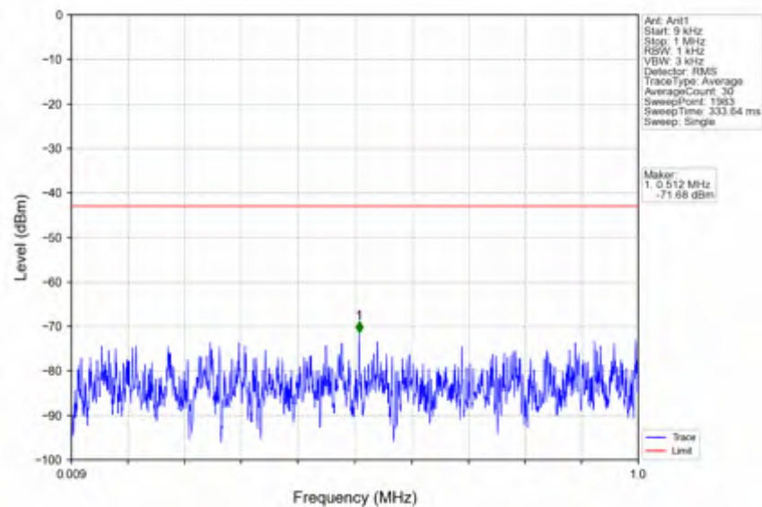
n25_30kHz_SISO_NTNV_10MHz_CP-OFDM_QPSK_1855MHz_Outer_Full
