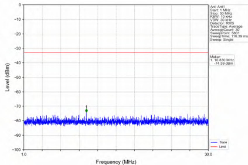
n25_15kHz_SISO_NTNV_40MHz_DFT-s-OFDM_QPSK_1870MHz_Outer_Full
