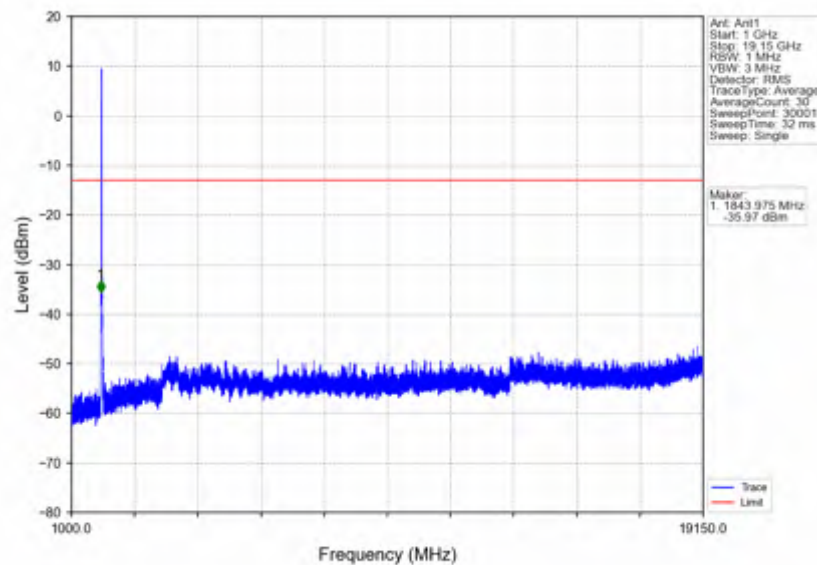
n25_30kHz_SISO_NTV_20MHz_CP-OFDM_QPSK_1860MHz_Outer_Full
