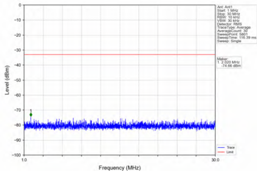
n25_30kHz_SISO_NTNV_10MHz_DFT-s-OFDM QPSK_1910MHz_Edge_1RB_Right
