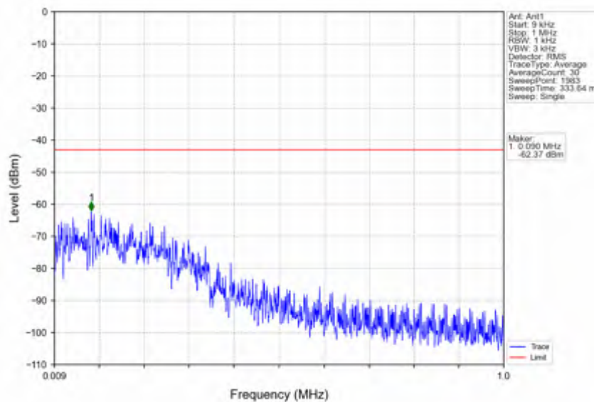
n25_30kHz_SISO_NTNV_15MHz_CP-OFDM_QPSK_1857.5MHz_Edge_1RB_Left
