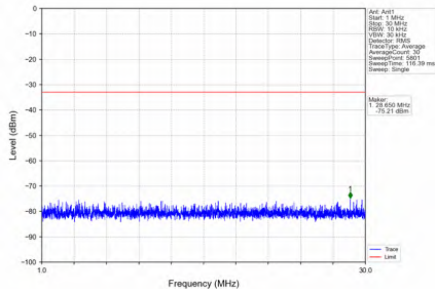
n25_30kHz_SISO_NTNV_10MHz_DFT-s-OFDM QPSK_1910MHz_Outer_Full
