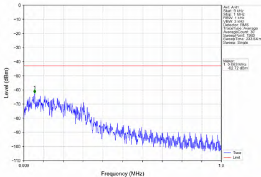
n25_30kHz_SISO_NTNV_15MHz_CP-OFDM QPSK_1907.5MHz_Edge_1RB_Right
