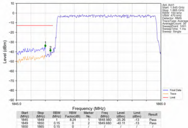
n25_30kHz_SISO_NTV_15MHz_CP-OFDM_QPSK_1857.5MHz_Outer_Full
