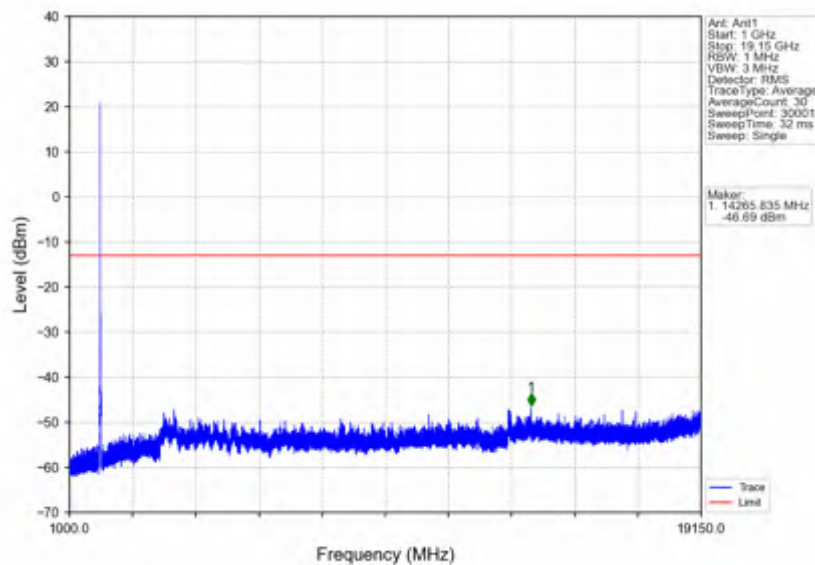
n25_30kHz_SISO_NTV_15MHz_CP-OFDM_QPSK_1882.5MHz_Edge_1RB_Left
