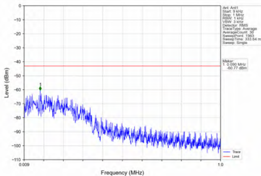
n25_30kHz_SISO_NTNV_20MHz_CP-OFDM QPSK_1905MHz_Edge_1RB_Right
