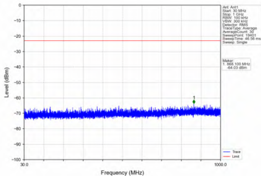
n25_15kHz_SISO_NTNV_40MHz_CP-OFDM QPSK_1870MHz_Edge_1RB_Left
