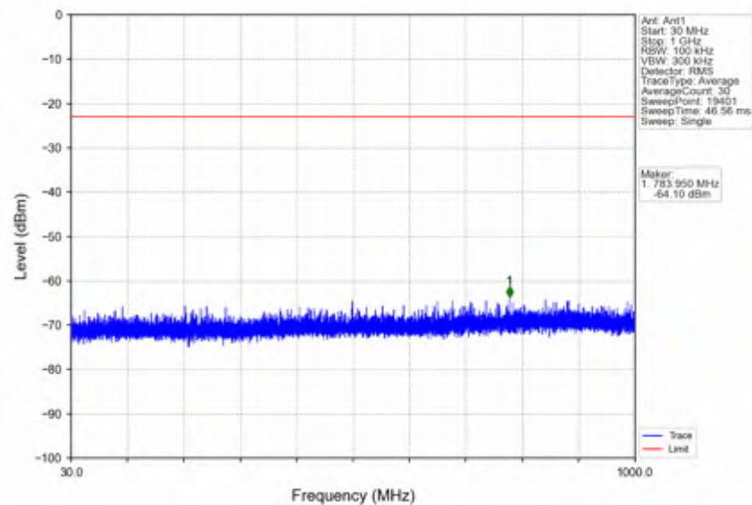
n25_15kHz_SISO_NTNV_40MHz_CP-OFDM QPSK_1895MHz_Edge_1RB_Right
