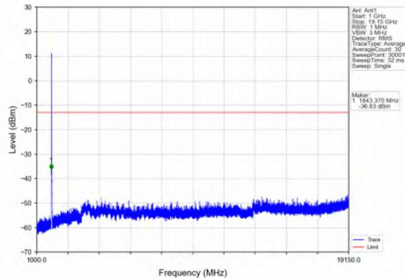
n25_30kHz_SISO_NTNV_15MHz_CP-OFDM_QPSK_1857.5MHz_Outer_Full
