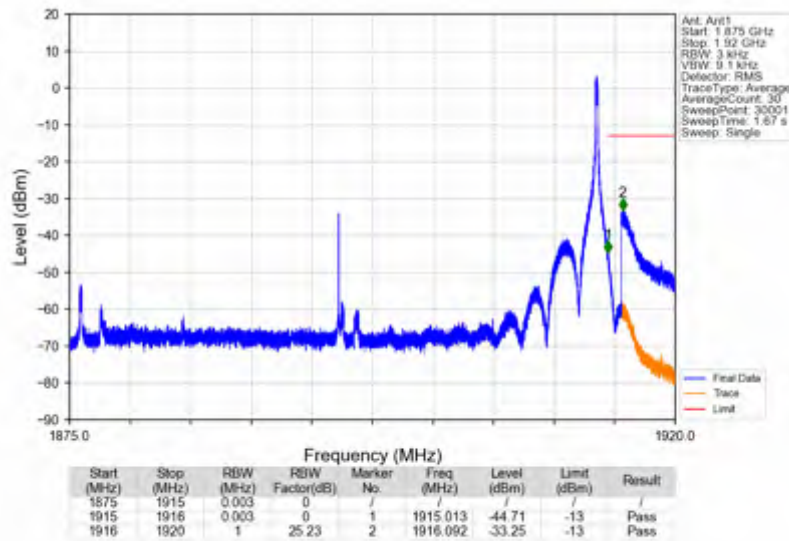
n25_15kHz_SISO_NTNV_40MHz_CP-OFDM QPSK_1895MHz_Inner_1RB_Right
