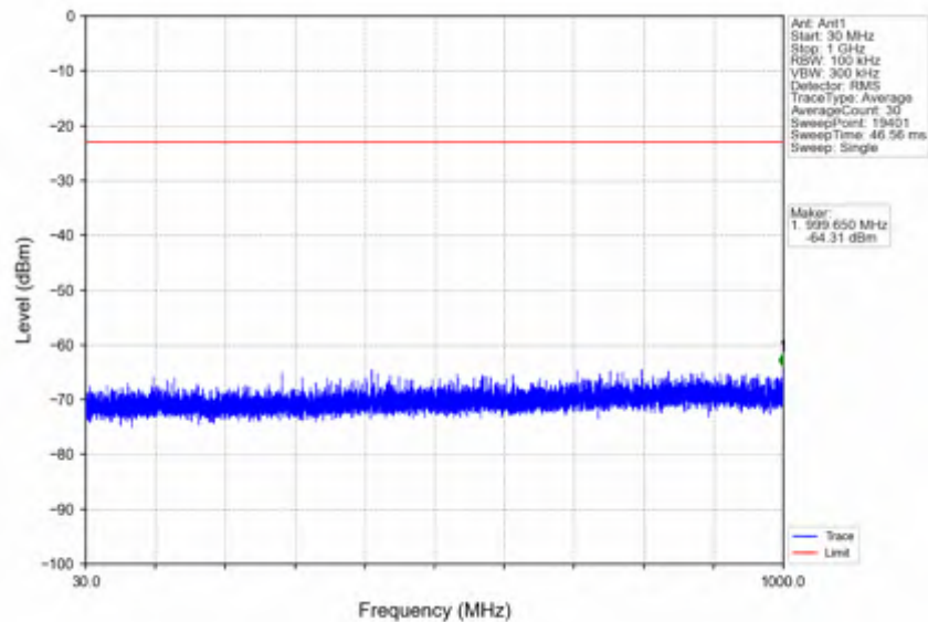
n25_30kHz_SISO_NTNV_20MHz_DFT-s-OFDM_PI/2_BPSK_1905MHz_Outer_Full
