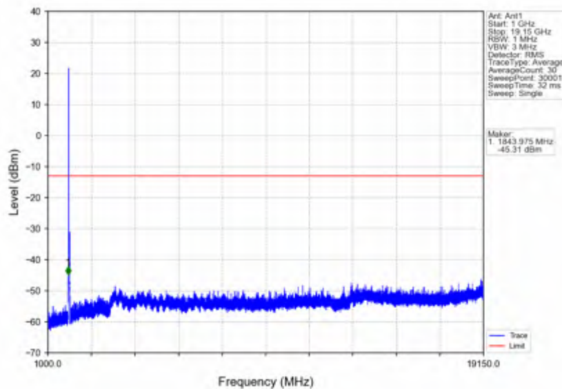
n25_15kHz_SISO_NTNV_40MHz_DFT-s-OFDM_QPSK_1895MHz_Edge_1RB_Right
