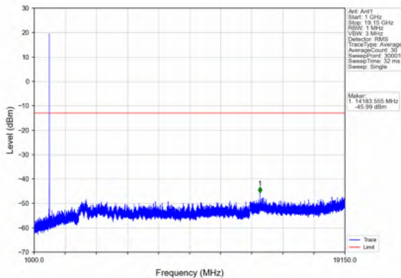
n25_30kHz_SISO_NTNV_10MHz_CP-OFDM QPSK_1882.5MHz_Edge_1RB_Left
