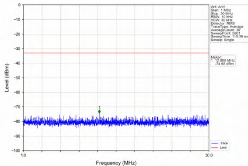
n25_30kHz_SISO_NTNV_20MHz_CP-OFDM_QPSK_1882.5MHz_Edge_1RB_Left
