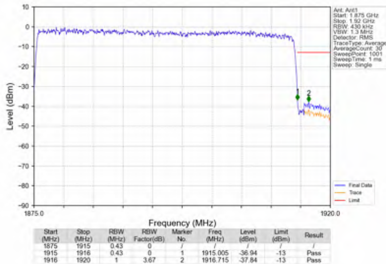
n25_15kHz_SISO_NTNV_40MHz_CP-OFDM QPSK_1895MHz_Outer_Full
