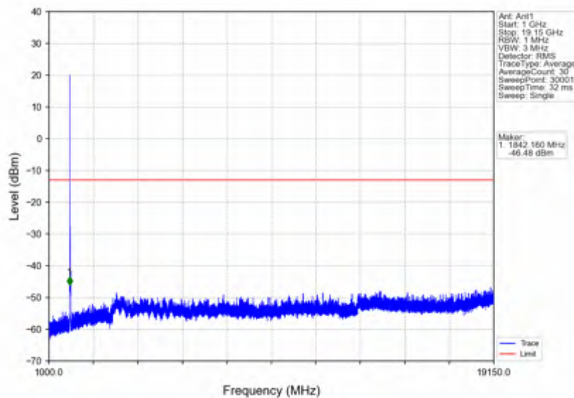
n25_30kHz_SISO_NTNV_20MHz_CP-OFDM QPSK_1860MHz_Outer_Full
