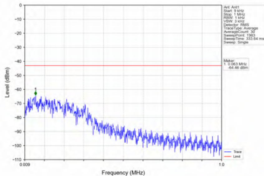
n25_30kHz_SISO_NTNV_15MHz_CP-OFDM_QPSK_1882.5MHz_Edge_1RB_Left
