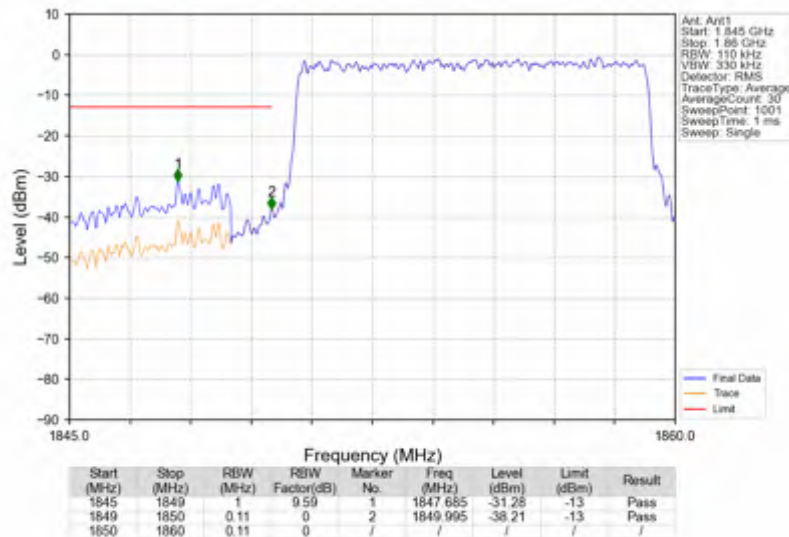
n25_30kHz_SISO_NTNV_10MHz_CP-OFDM QPSK_1855MHz_Outer_Full
