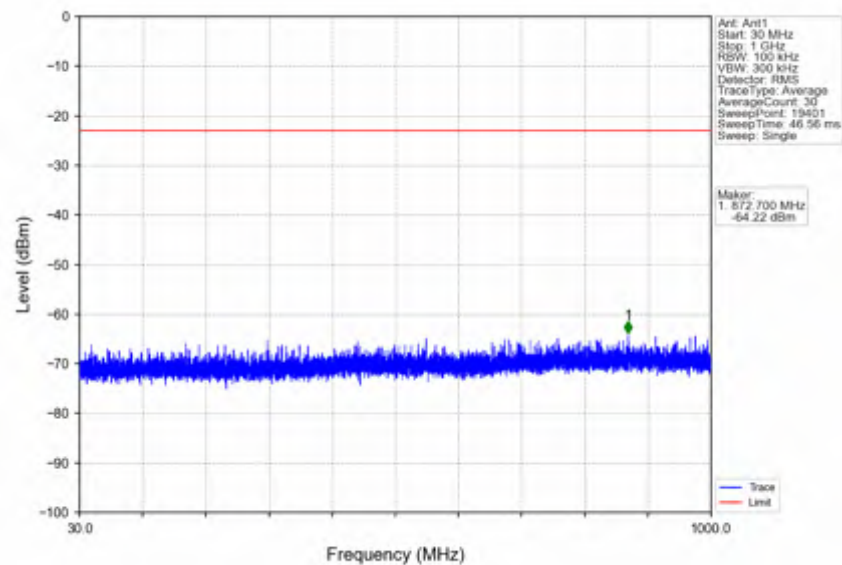
n25_15kHz_SISO_NTNV_40MHz_CP-OFDM_QPSK_1870MHz_Outer_Full
