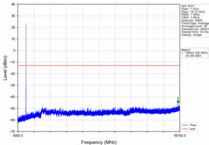
n25_30kHz_SISO_NTNV_10MHz_DFT-s-OFDM QPSK_1855MHz_Edge_1RB_Left
