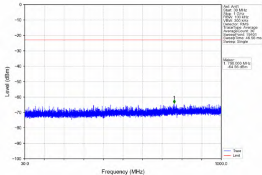
n25_15kHz_SISO_NTNV_40MHz_DFT-s-OFDM QPSK_1895MHz_Edge_1RB_Right
