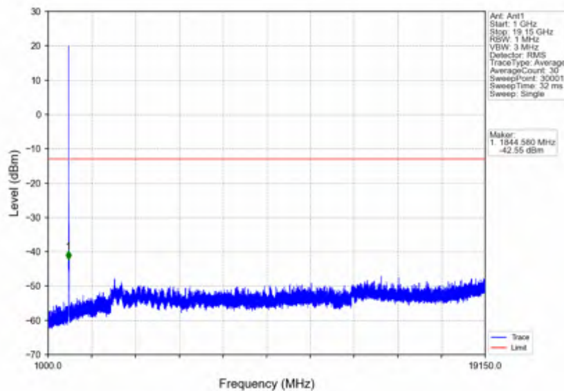
n25_30kHz_SISO_NTV_15MHz_CP-OFDM_QPSK_1857.5MHz_Outer_Full
