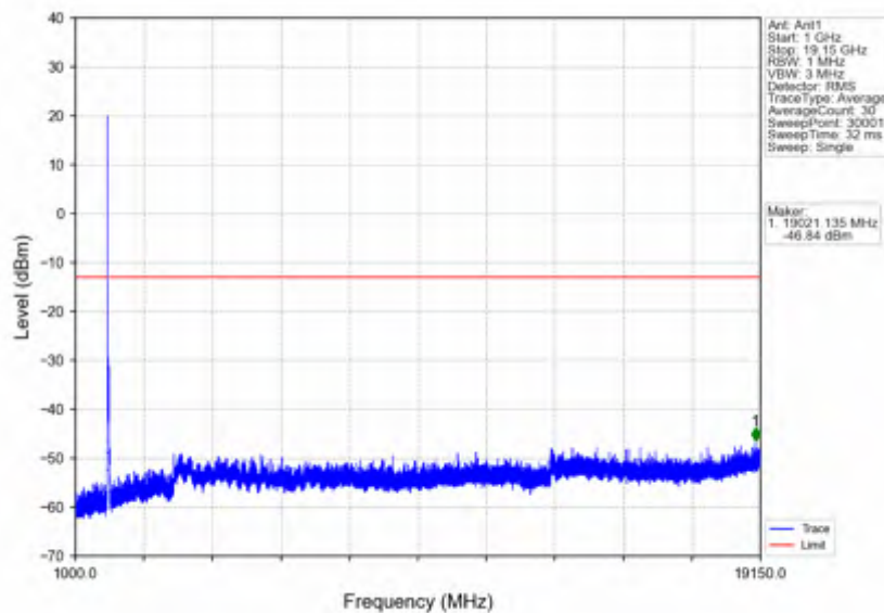
n25_15kHz_SISO_NTNV_40MHz_CP-OFDM QPSK_1870MHz_Outer_Full
