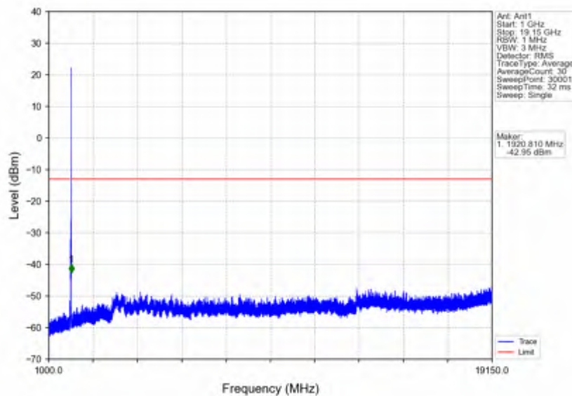
n25_30kHz_SISO_NTNV_15MHz_DFT-s-OFDM_QPSK_1907.5MHz_Edge_1RB_Right
