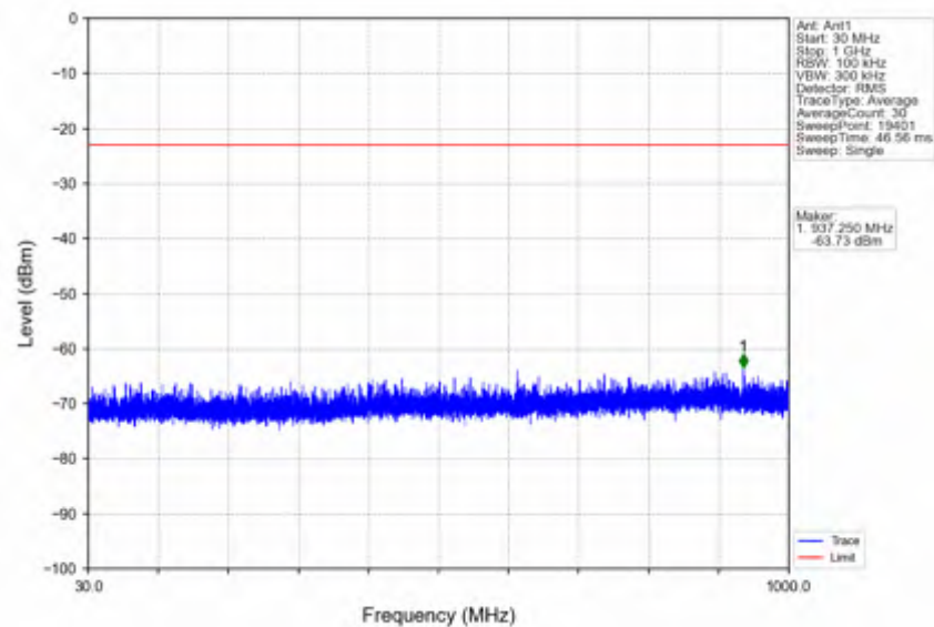
n25_30kHz_SISO_NTV_20MHz_CP-OFDM_QPSK_1905MHz_Outer_Full
