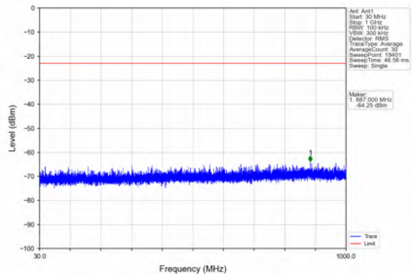
n25_30kHz_SISO_NTNV_10MHz_DFT-s-OFDM QPSK_1855MHz_Outer_Full
