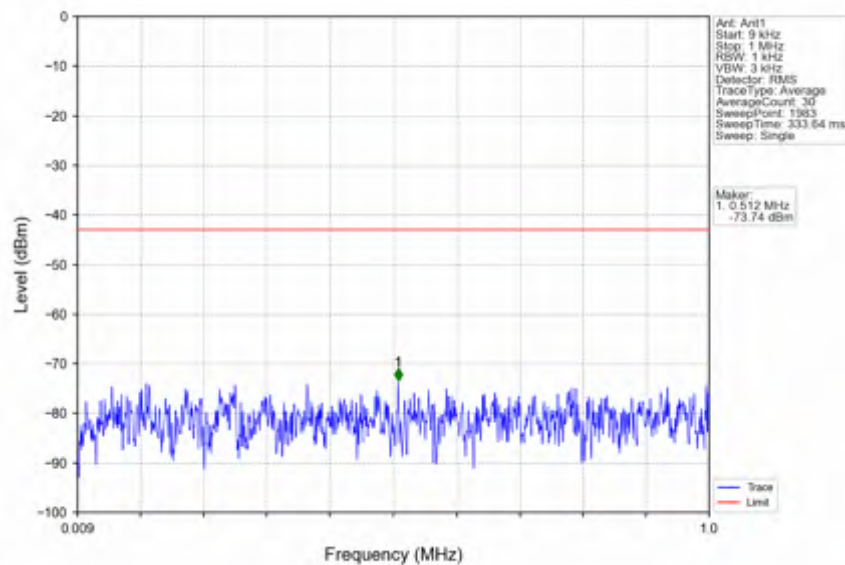
n25_30kHz_SISO_NTNV_10MHz_CP-OFDM QPSK_1910MHz_Outer_Full
