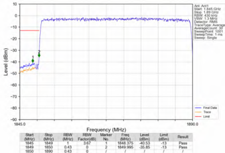
n25_15kHz_SISO_NTNV_40MHz_CP-OFDM QPSK_1870MHz_Outer_Full
