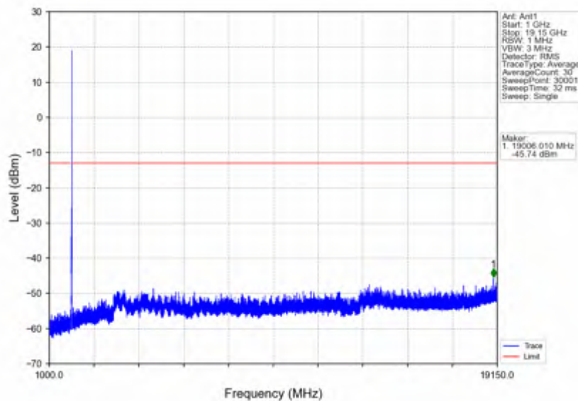
n25_30kHz_SISO_NTNV_15MHz_CP-OFDM QPSK_1907.5MHz_Outer_Full
