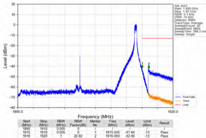
n25_30kHz_SISO_NTNV_20MHz_CP-OFDM QPSK_1905MHz_Edge_1RB_Right
