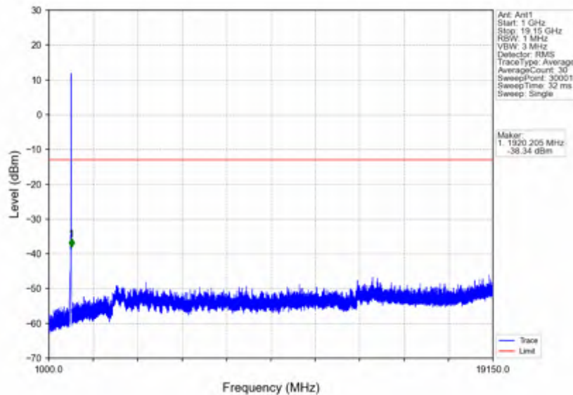
n25_30kHz_SISO_NTNV_20MHz_DFT-s-OFDM_PI/2_BPSK_1905MHz_Outer_Full
