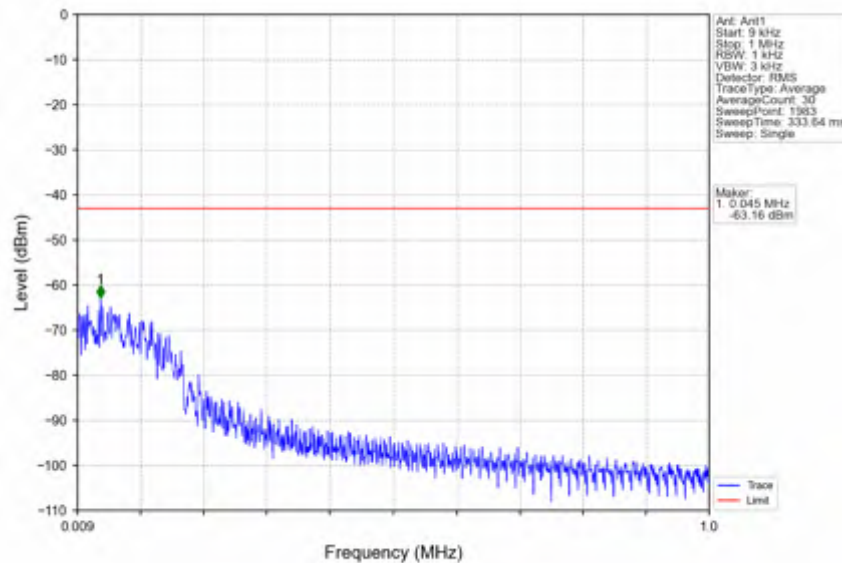
n25_15kHz_SISO_NTNV_40MHz_CP-OFDM_QPSK_1882.5MHz_Edge_1RB_Left
