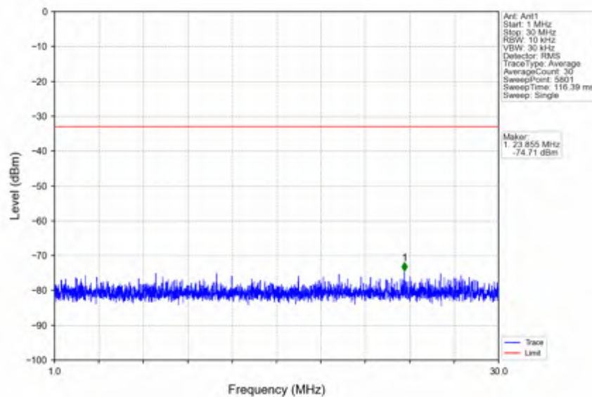
n25_30kHz_SISO_NTNV_15MHz_CP-OFDM QPSK_1907.5MHz_Edge_1RB_Right
