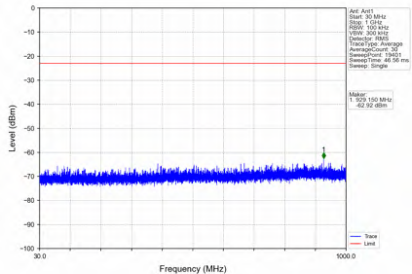
n25_30kHz_SISO_NTNV_20MHz_DFT-s-OFDM QPSK_1905MHz_Outer_Full
