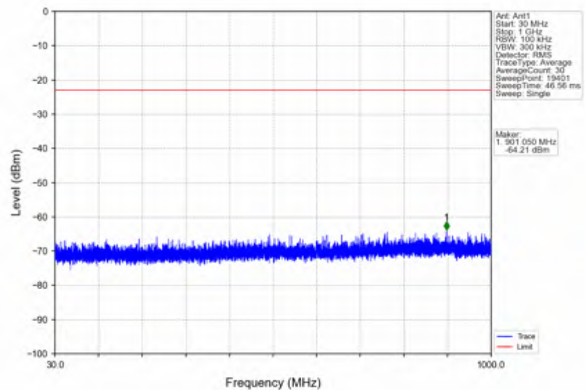
n25_15kHz_SISO_NTNV_40MHz_DFT-s-OFDM QPSK_1895MHz_Outer_Full
