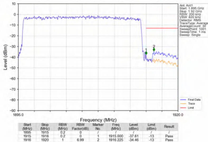
n25_30kHz_SISO_NTNV_20MHz_CP-OFDM QPSK_1905MHz_Outer_Full
