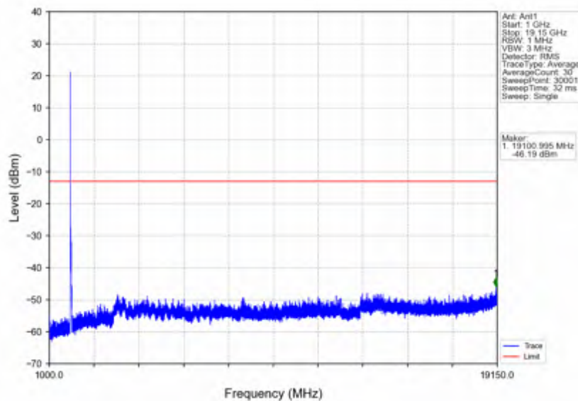
n25_15kHz_SISO_NTNV_40MHz_CP-OFDM QPSK_1882.5MHz_Edge_1RB_Left
