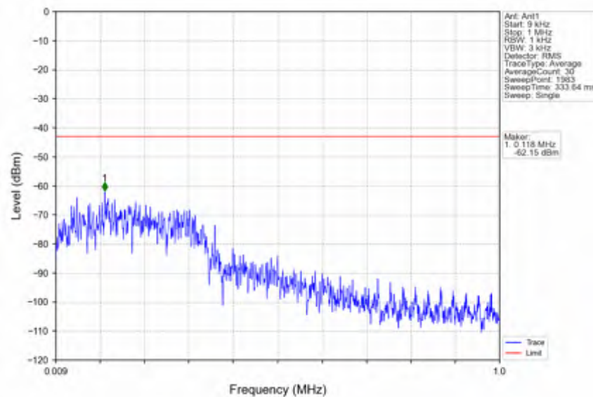
n25_30kHz_SISO_NTNV_10MHz_DFT-s-OFDM QPSK_185MHz_Edge_1RB_Left
