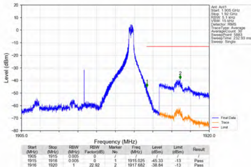
n25_30kHz_SISO_NTNV_10MHz_DFT-s-OFDM QPSK_1910MHz_Inner_1RB_Right
