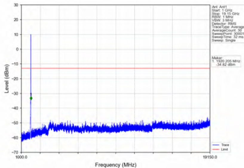
n25_30kHz_SISO_NTV_20MHz_CP-OFDM_QPSK_1905MHz_Outer_Full
