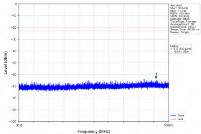
n25_30kHz_SISO_NTNV_15MHz_CP-OFDM_QPSK_1857.5MHz_Edge_1RB_Left
