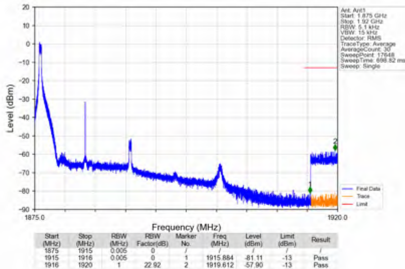
n25_30kHz_SISO_NTV_15MHz_CP-OFDM QPSK_1882.5MHz_Edge_1RB_Left
