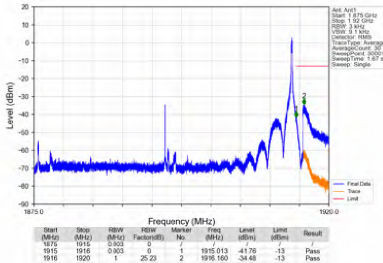
n25_15kHz_SISO_NTNV_40MHz_CP-OFDM_QPSK_1895MHz_Edge_1RB_Right
