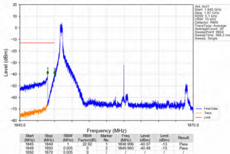
n25_30kHz_SISO_NTNV_20MHz_DFT-s-OFDM QPSK_1860MHz_Edge_1RB_Left
