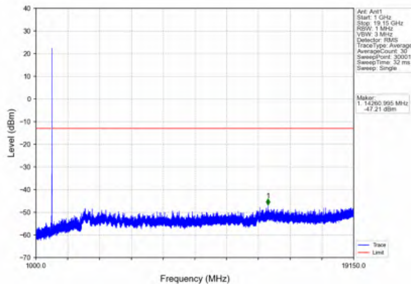
n25_30kHz_SISO_NTNV_10MHz_DFT-s-OFDM_QPSK_1910MHz_Edge_1RB_Right
