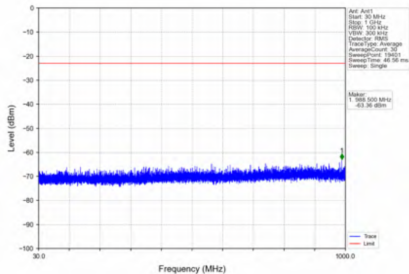
n25_30kHz_SISO_NTV_20MHz_CP-OFDM_QPSK_1860MHz_Outer_Full
