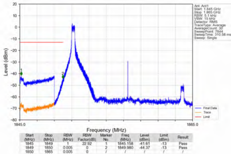
n25_30kHz_SISO_NTV_15MHz_CP-OFDM_QPSK_1857.5MHz_Inner_1RB_Left
