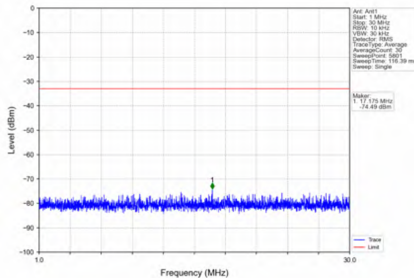
n25_30kHz_SISO_NTV_15MHz_CP-OFDM_QPSK_1857.5MHz_Inner_1RB_Left
