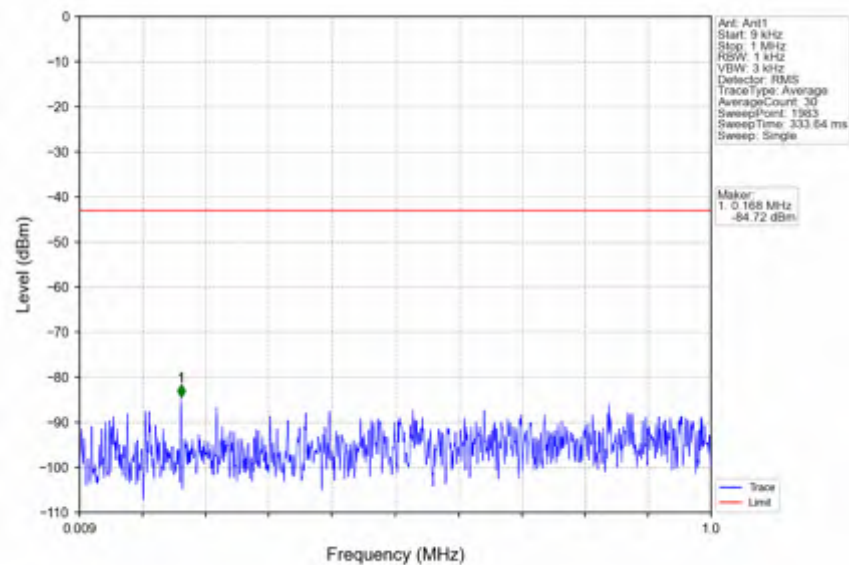
n25_30kHz_SISO_NTNV_20MHz_DFT-s-OFDM_PI/2_BPSK_1860MHz_Outer_Full
