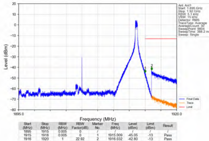
n25_30kHz_SISO_NTNV_20MHz_DFT-s-OFDM QPSK_1905MHz_Inner_1RB_Right
