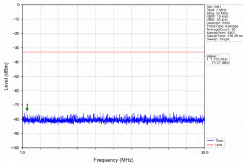
n25_30kHz_SISO_NTNV_20MHz_CP-OFDM QPSK_1860MHz_Edge_1RB_Left
