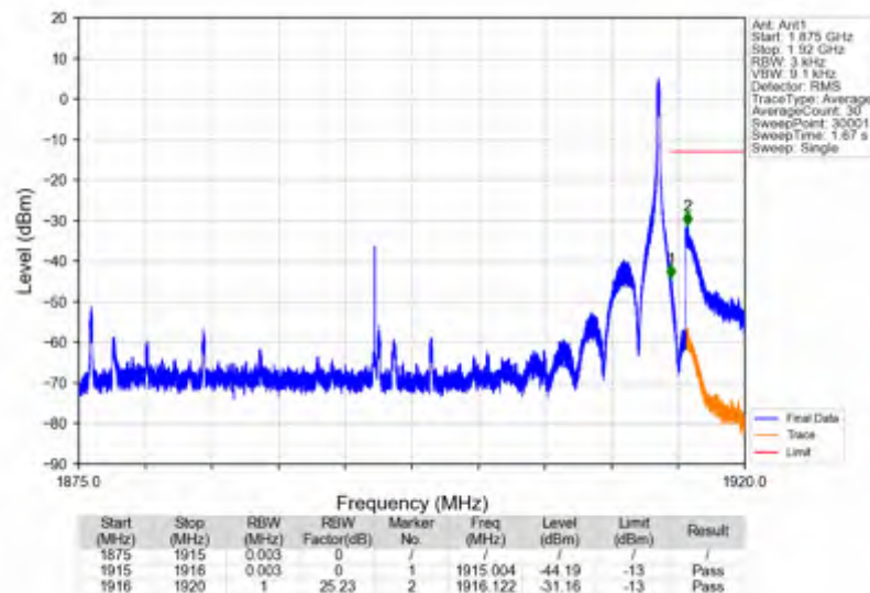
n25_15kHz_SISO_NTNV_40MHz_DFT-s-OFDM QPSK_1895MHz_Inner_1RB_Right
