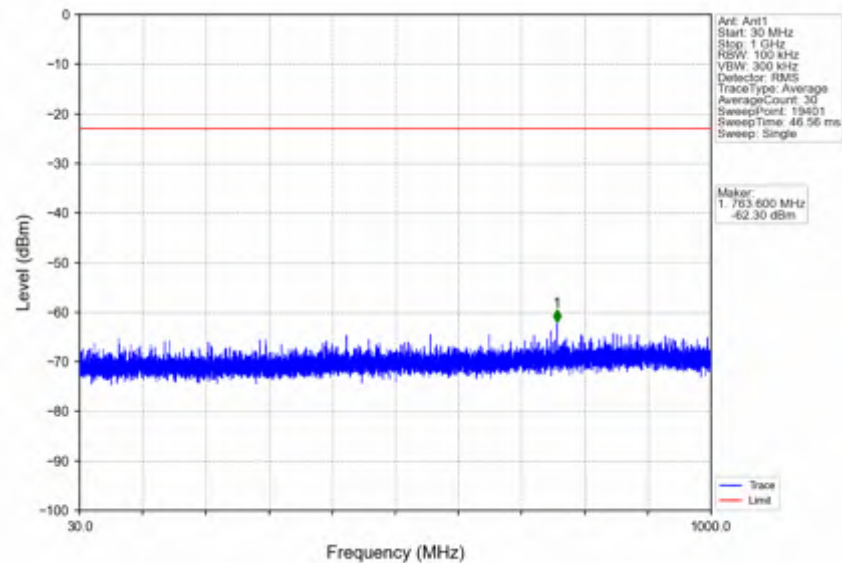
n25_30kHz_SISO_NTNV_10MHz_DFT-s-OFDM_QPSK_1910MHz_Edge_1RB_Right
