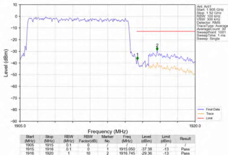
n25_30kHz_SISO_NTNV_10MHz_CP-OFDM QPSK_1910MHz_Outer_Full
