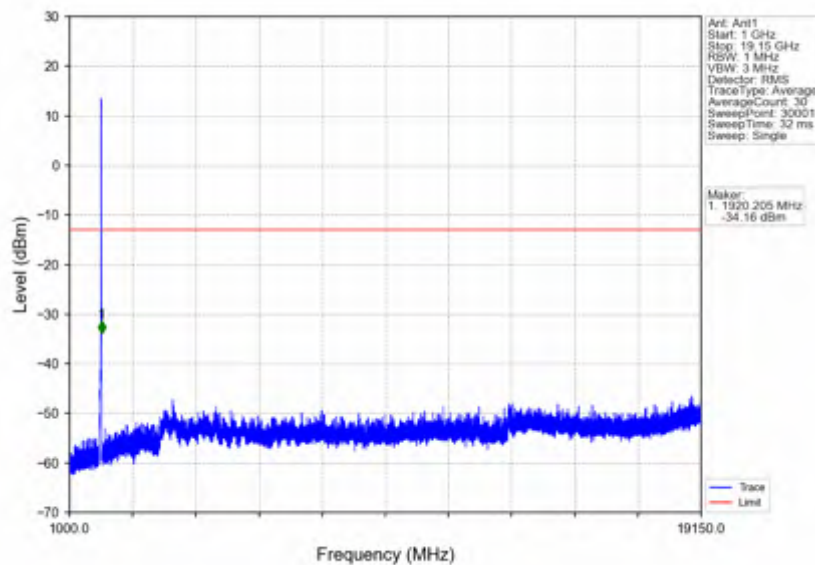
n25_30kHz_SISO_NTNV_15MHz_DFT-s-OFDM QPSK_1907.5MHz_Inner_1RB_Right
