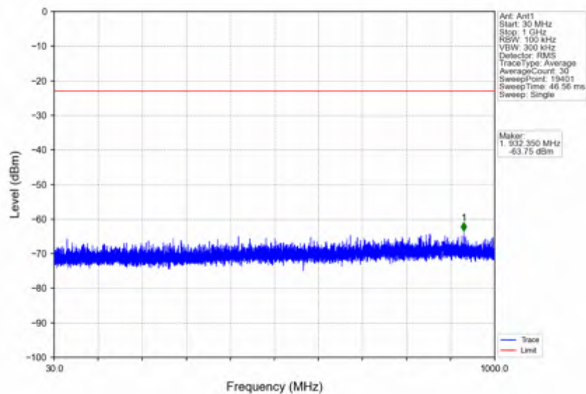
n25_30kHz_SISO_NTNV_20MHz_CP-OFDM QPSK_1882.5MHz_Edge_1RB_Left
