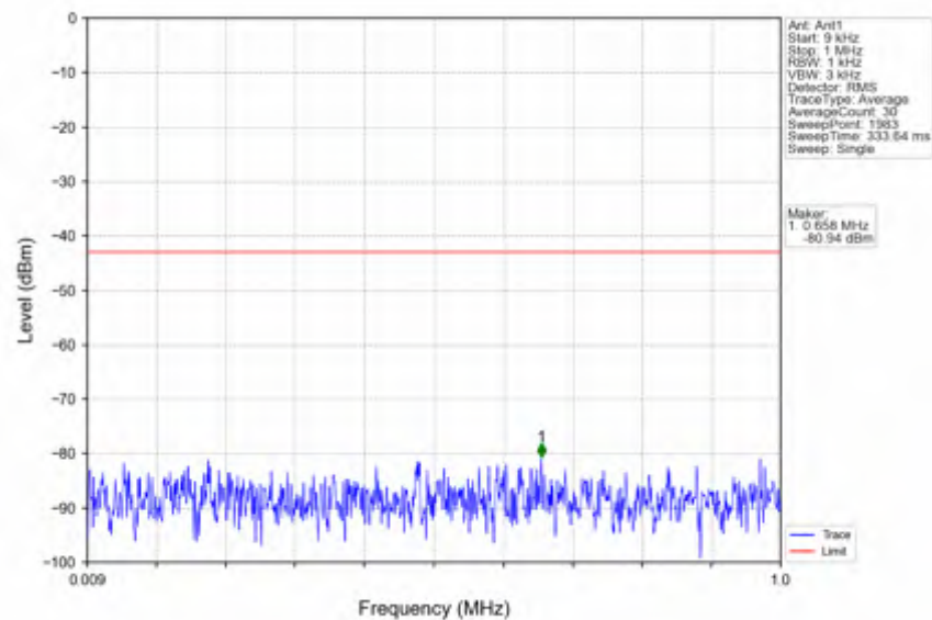
n25_15kHz_SISO_NTNV_40MHz_CP-OFDM QPSK_1895MHz_Outer_Full
