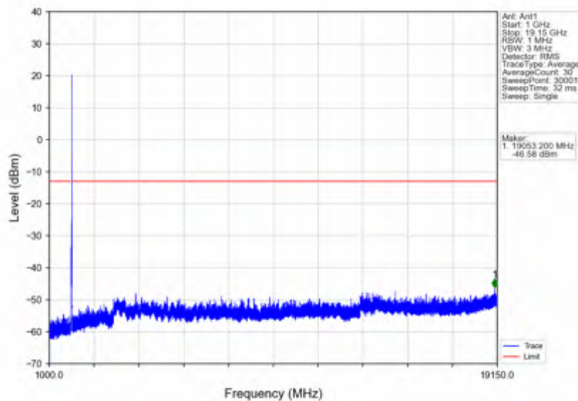
n25_30kHz_SISO_NTNV_20MHz_CP-OFDM QPSK_1905MHz_Outer_Full
