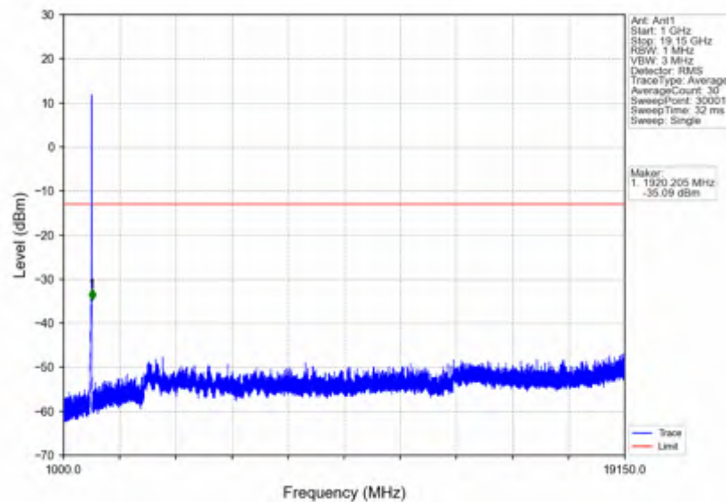
n25_30kHz_SISO_NTNV_20MHz_DFT-s-OFDM QPSK_1905MHz_Inner_1RB_Right
