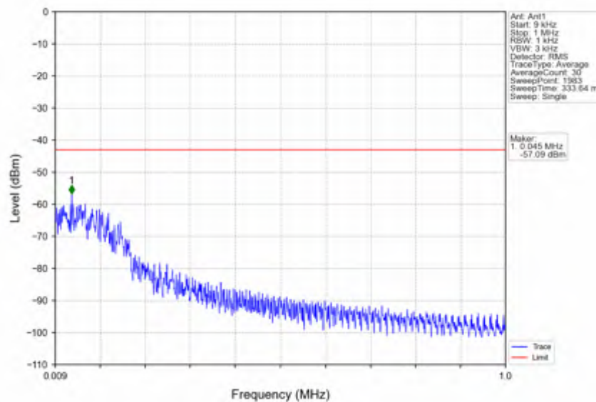
n25_15kHz_SISO_NTNV_40MHz_CP-OFDM QPSK_1895MHz_Inner_1RB_Right
