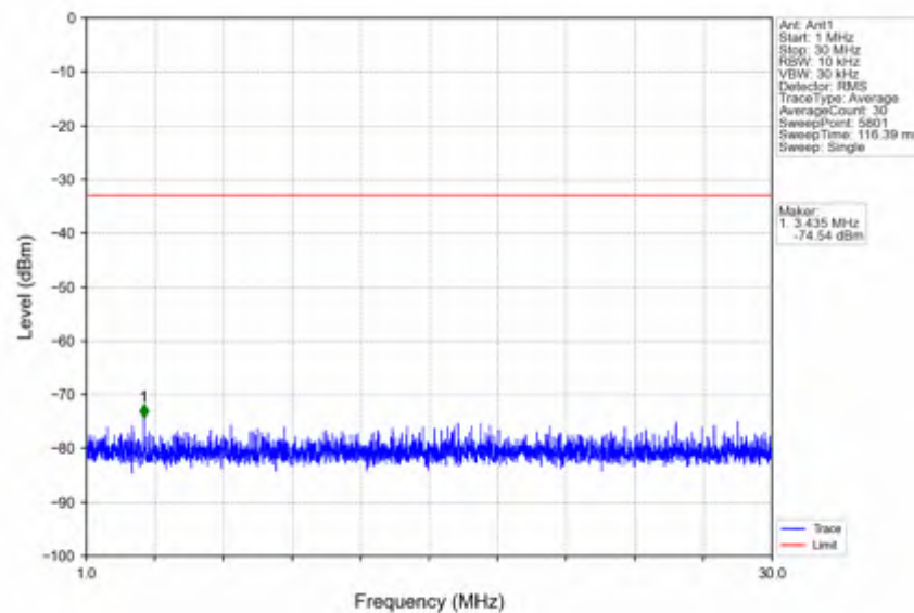
n25_30kHz_SISO_NTNV_10MHz_CP-OFDM QPSK_1910MHz_Edge_1RB_Right
