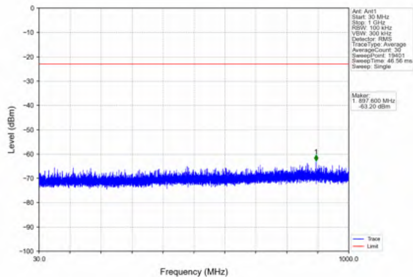
n25_30kHz_SISO_NTNV_15MHz_CP-OFDM QPSK_1907.5MHz_Outer_Full
