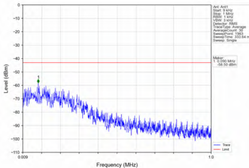
n25_30kHz_SISO_NTV_15MHz_CP-OFDM_QPSK_1857.5MHz_Inner_1RB_Left
