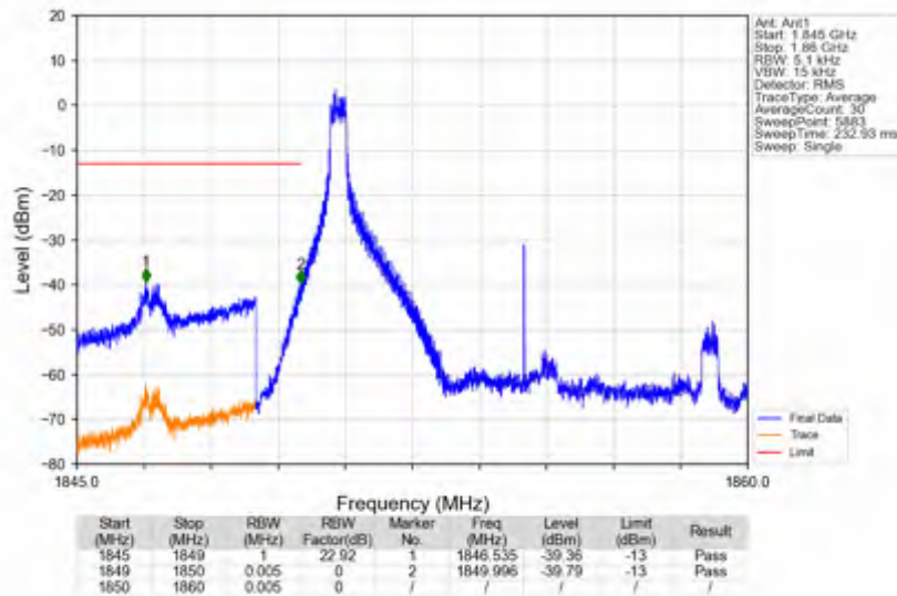
n25_30kHz_SISO_NTNV_10MHz_DFT-s-OFDM QPSK_1855MHz_Edge_1RB_Left
