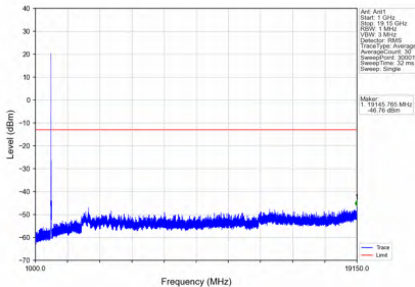
n25_30kHz_SISO_NTNV_20MHz_CP-OFDM QPSK_1882.5MHz_Edge_1RB_Left
