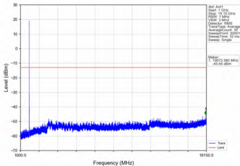
n25_30kHz_SISO_NTNV_10MHz_CP-OFDM QPSK_1855MHz_Outer_Full
