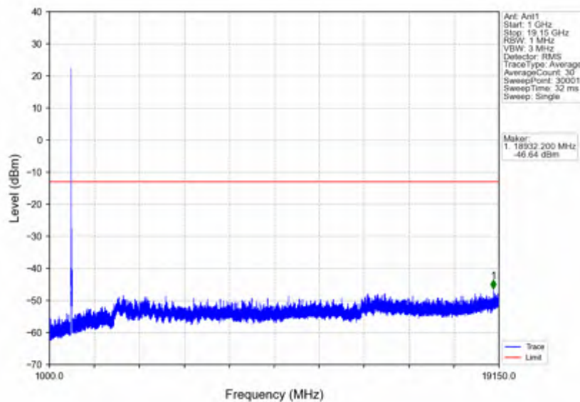
n25_30kHz_SISO_NTNV_20MHz_DFT-s-OFDM_QPSK_1905MHz_Edge_1RB_Right
