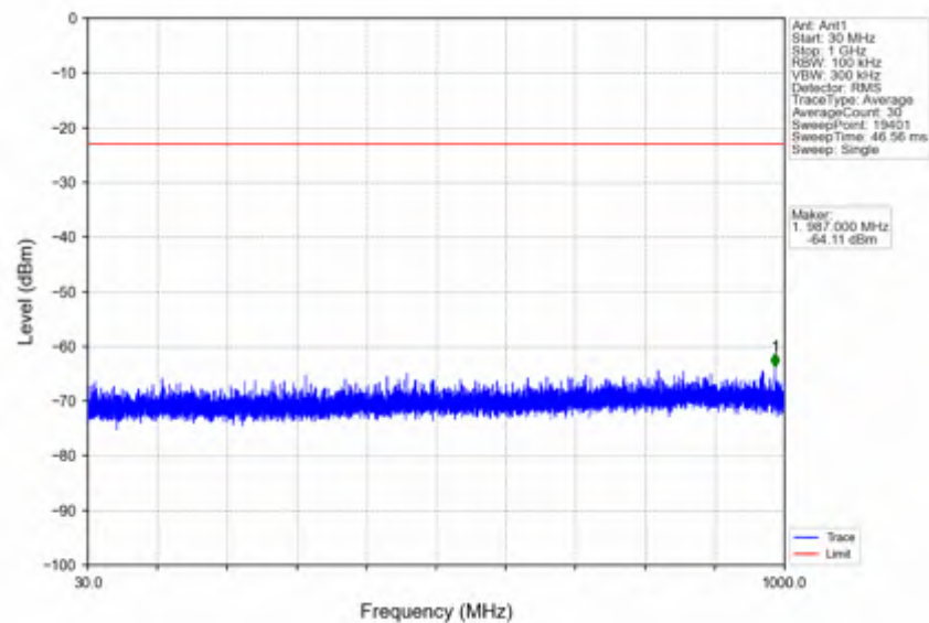
n25_30kHz_SISO_NTNV_10MHz_DFT-s-OFDM_QPSK_1855MHz_Edge_1RB_Left
