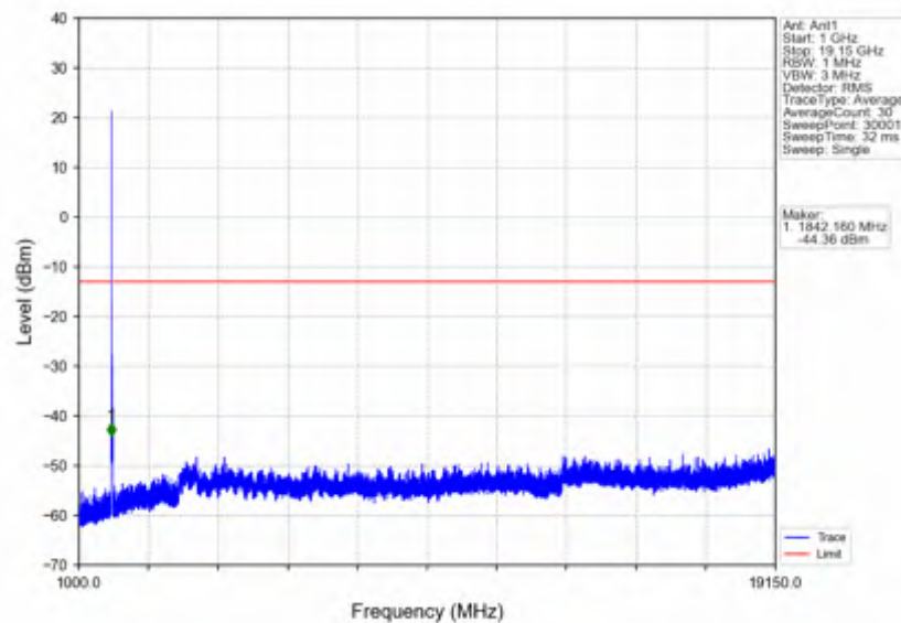
n25_30kHz_SISO_NTNV_20MHz_DFT-s-OFDM_QPSK_1860MHz_Edge_1RB_Left
