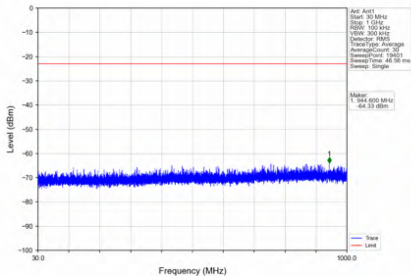
n25_30kHz_SISO_NTNV_10MHz_CP-OFDM QPSK_1910MHz_Outer_Full
