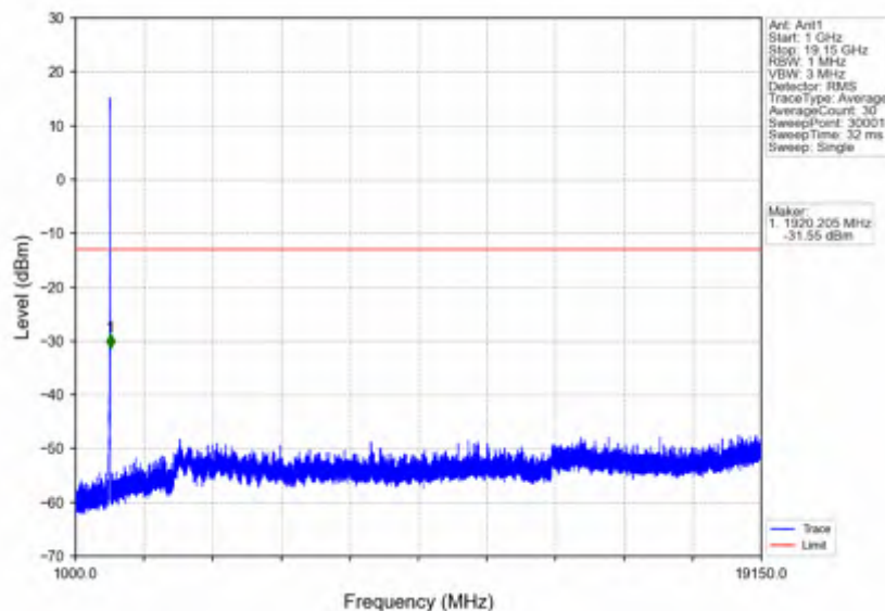
n25_30kHz_SISO_NTNV_10MHz_DFT-s-OFDM QPSK_1910MHz_Inner_1RB_Right
