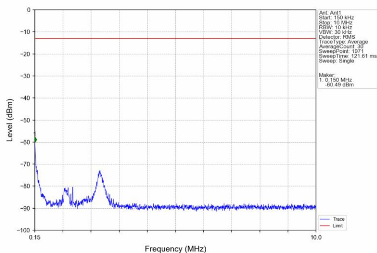
Band26b_3MHz_16QAM_LCH_825.5MHz_RB_1_0_NTNV
