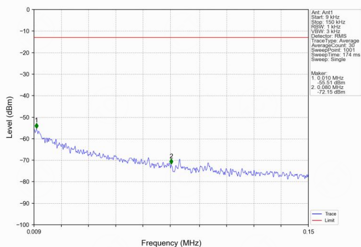
Band26b_5MHz_QPSK_MCH_836.5MHz_RB_1_0_NTNV
