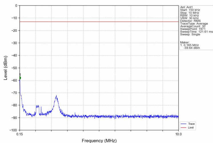
Band26b_3MHz_QPSK_LCH_825.5MHz_RB_1_0_NTNV
