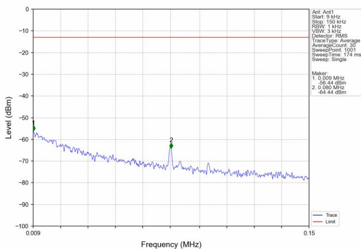
Band26b_3MHz_QPSK_LCH_825.5MHz_RB_1_0_NTNV
