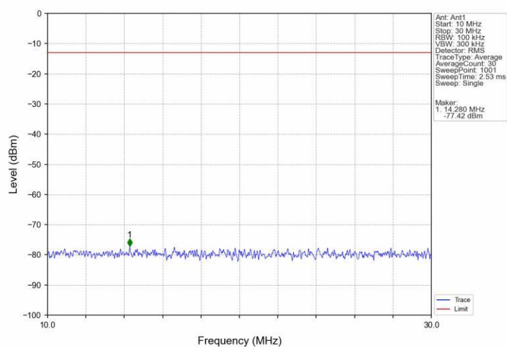
Band26b_3MHz_16QAM_LCH_825.5MHz_RB_1_0_NTNV
