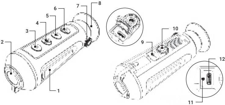
FIGURE 1-1. MAIN PARTS
