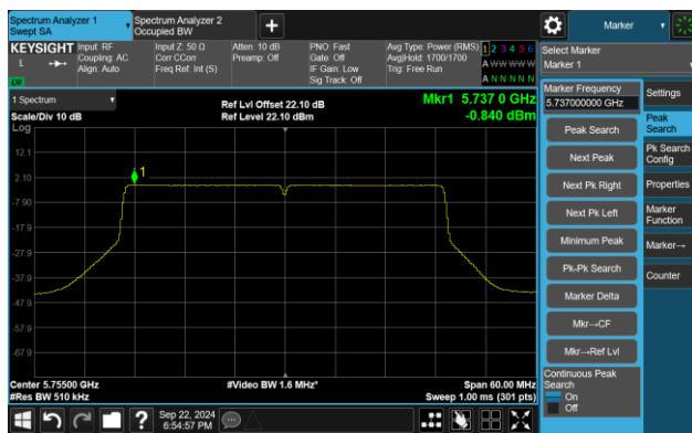
Channel 151 (5755MHz)
