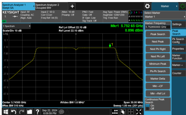
Channel 149 (5745MHz)
