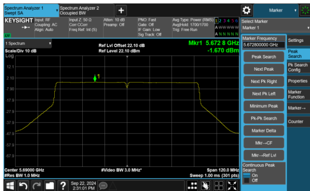
Channel 138 (5690MHz)
