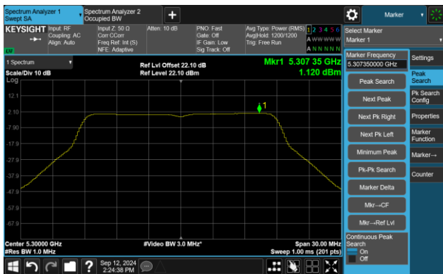
Channel 60 (5300MHz)
