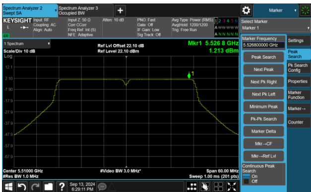
Channel 102 (5510MHz)
