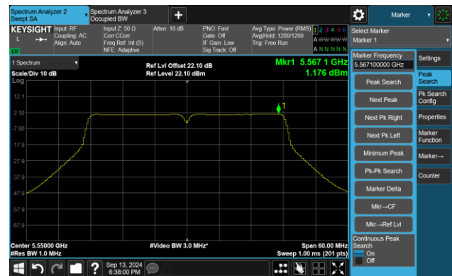
Channel 110 (5550MHz)
