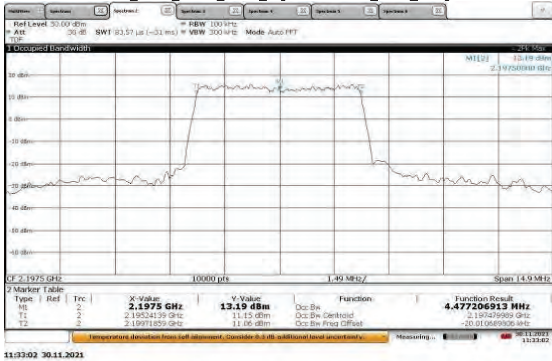
B66_ANT0_QPSK_5MHz_High 2197.5 MHz_OBW_0 deg
