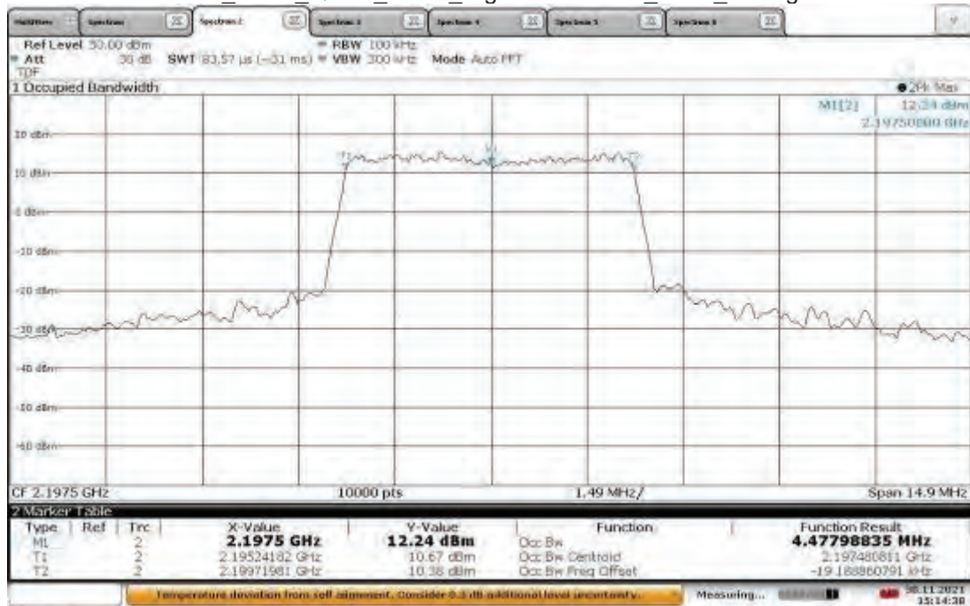
B66_ANT0_QPSK_5MHz_High 2197.5 MHz_OBW_50 deg
