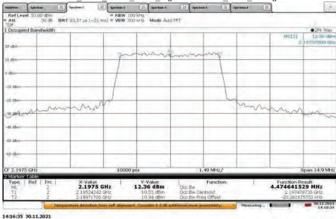
B66_ANT0_QPSK_5MHz_High 2197.5 MHz_OBW_30 deg
