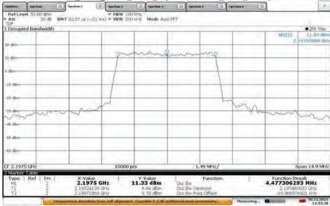
B66_ANT0_QPSK_5MHz_High 2197.5 MHz_OBW_40 deg
