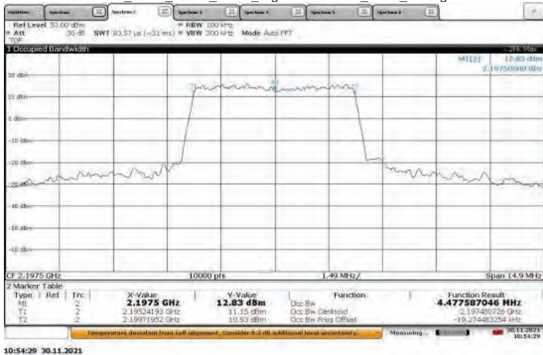
B66_ANT0_QPSK_5MHz_High 2197.5 MHz_OBW_10 deg
