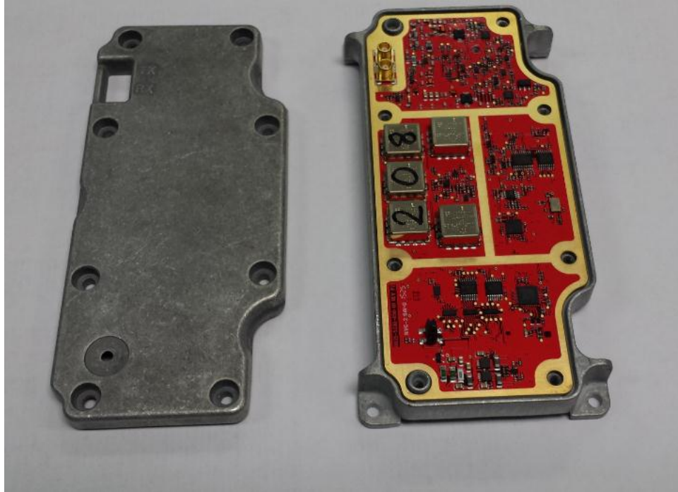
RF Board in Chassis with Cover Removed
