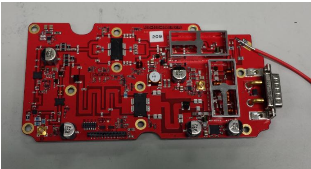
Transmitter Power Amplifier Board Top (Shield Frame Removed)
