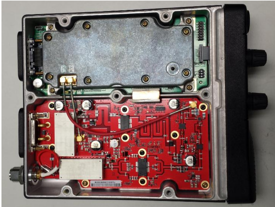
Radio with Bottom Cover Removed
