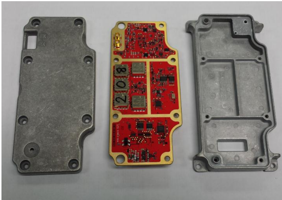
RF Board with Chassis
