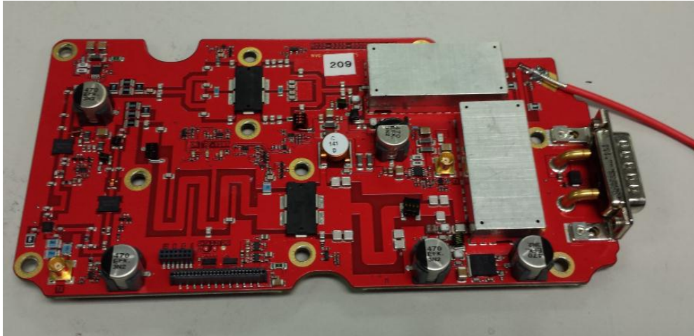
Transmitter Power Amplifier Board Top with shield
