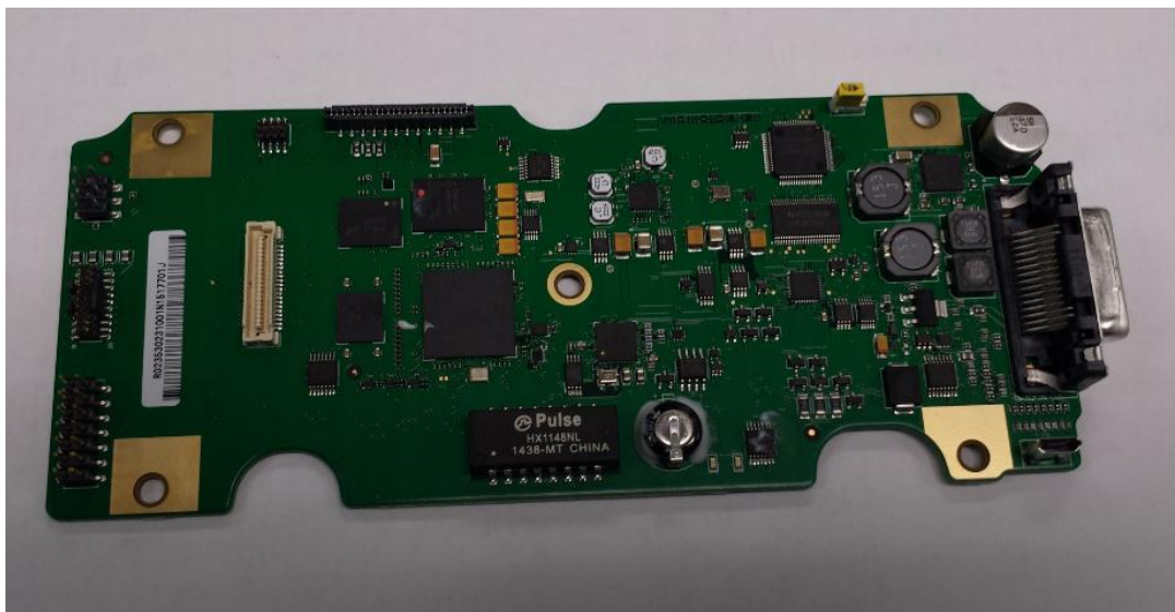
Logic Board Top
