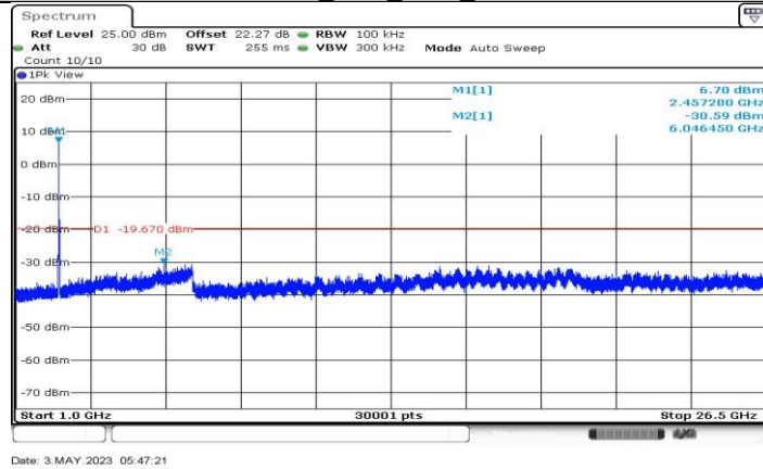
11G-CDD_Ant4_2457_1000~26500
