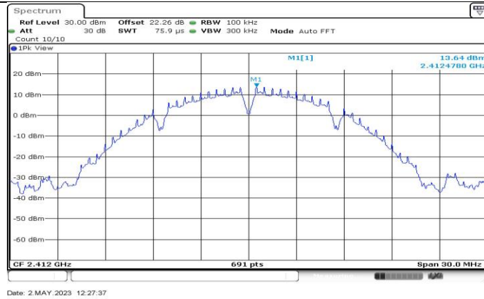
11B-CDD_Ant4_2412_0~Reference
