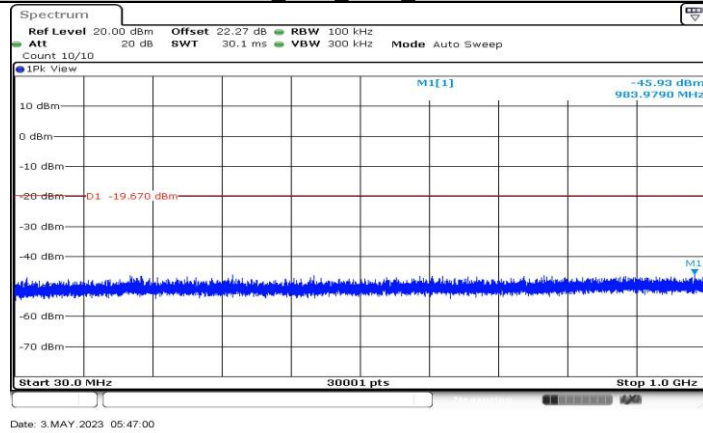
11G-CDD_Ant4_2457_30~1000
