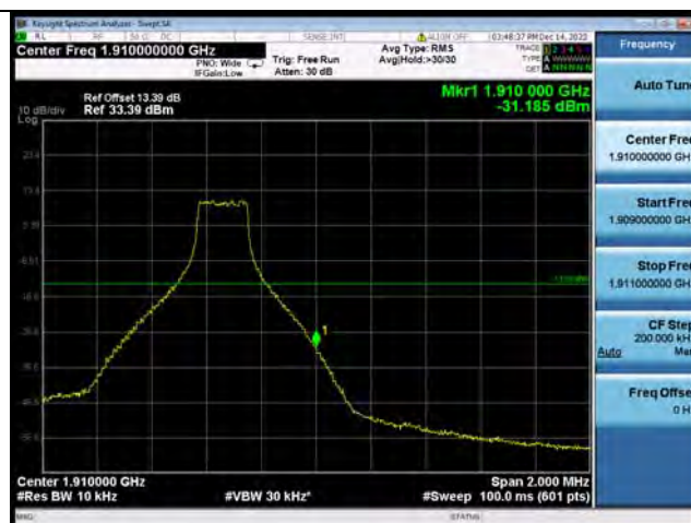
Band2-5MHz-QPSK-19175-25RB#0
