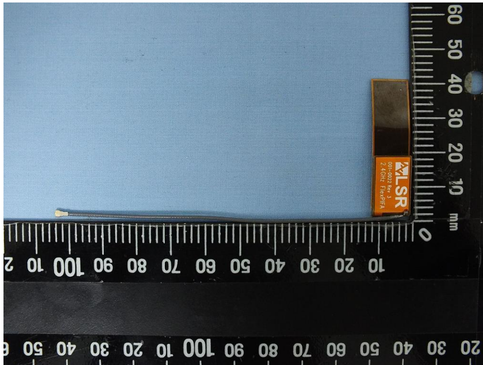
PCB Dipole antenna / model: FlexPIFA
