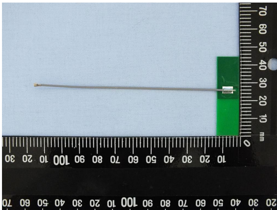
PCB Dipole antenna / model: NanoBlue
