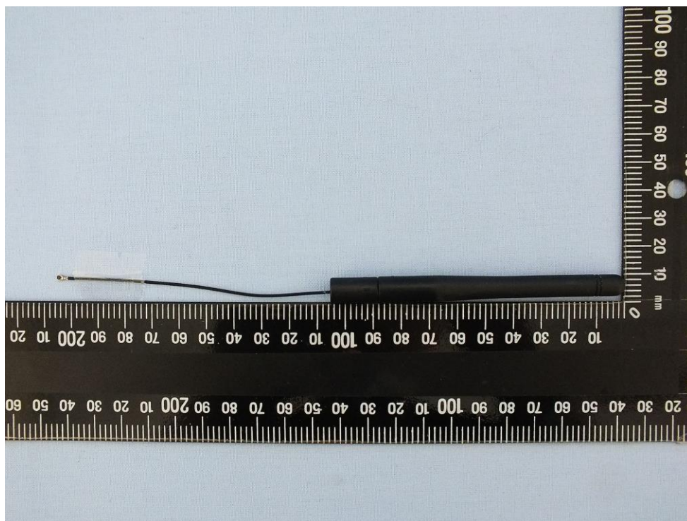
Dipole antenna / model: EDA-8709-2G4C1-B27-CY
