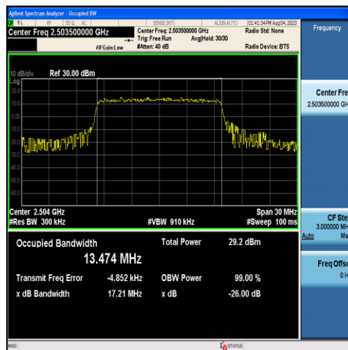
Band41-15MHz-16QAM-39725-75RB#0-13.474
