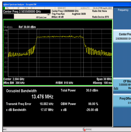
Band41-15MHz-QPSK-39725-75RB#0-13.476
