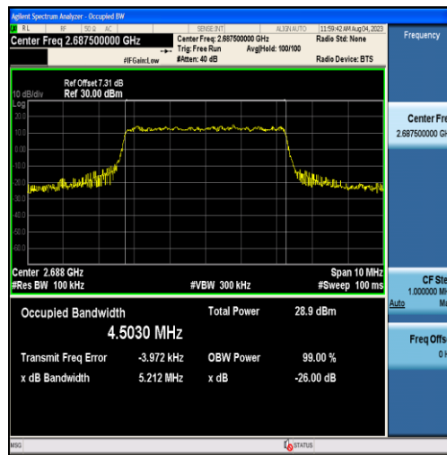
Band41-5MHz-16QAM-41565-25RB#0-4.5030
