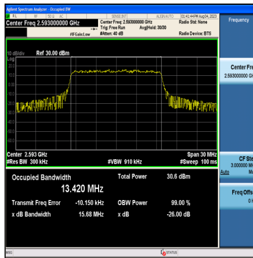
Band41-15MHz-QPSK-40620-75RB#0-13.420
