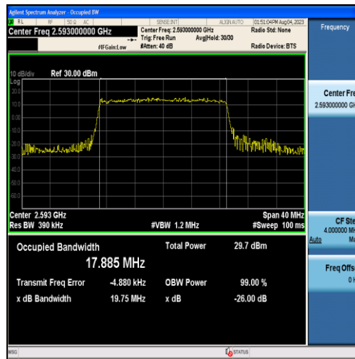
Band41-20MHz-16QAM-40620-100RB#0-17.885
