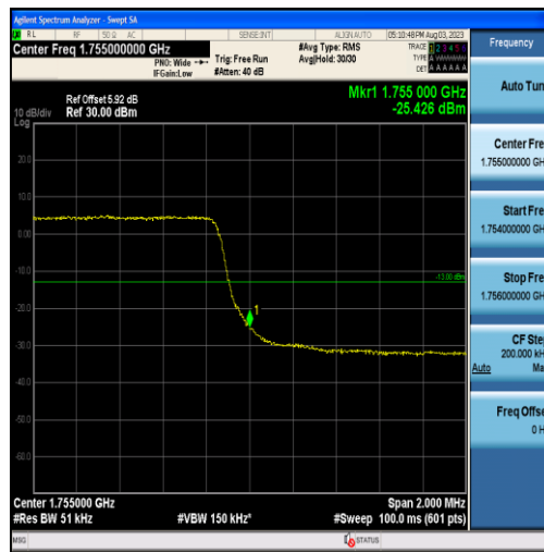
Band4-3MHz-QPSK-20385-15RB#0
