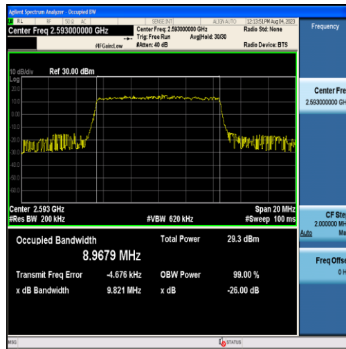
Band41-10MHz-16QAM-40620-50RB#0-8.9679
