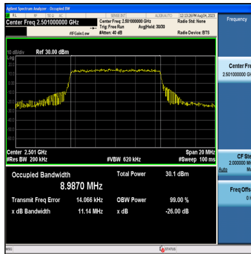
Band41-10MHz-QPSK-39700-50RB#0-8.9870
