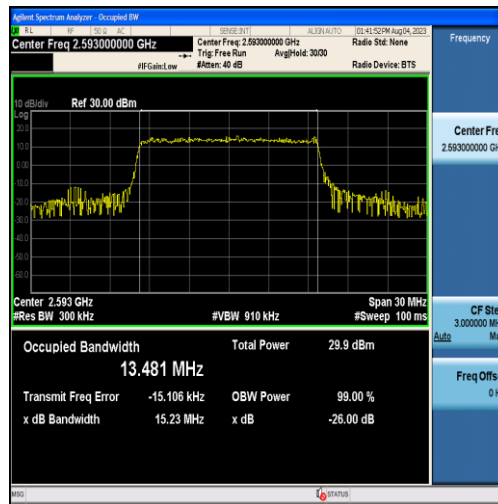
Band41-15MHz-16QAM-40620-75RB#0-13.481
