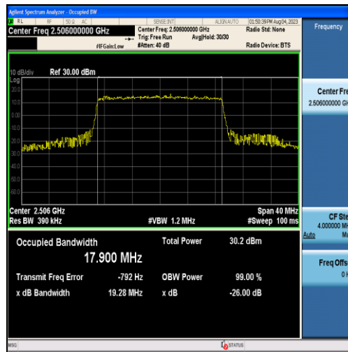
Band41-20MHz-QPSK-39750-100RB#0-17.900
