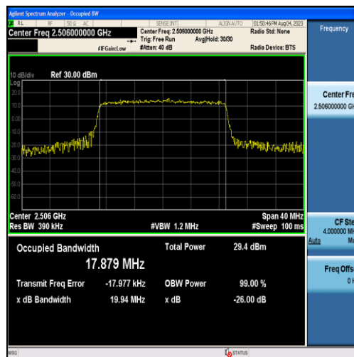
Band41-20MHz-16QAM-39750-100RB#0-17.879
