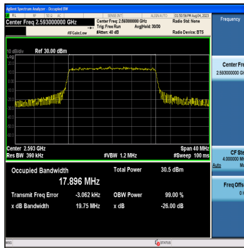
Band41-20MHz-QPSK-40620-100RB#0-17.896
