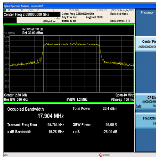
Band41-20MHz-QPSK-41490-100RB#0-17.904
