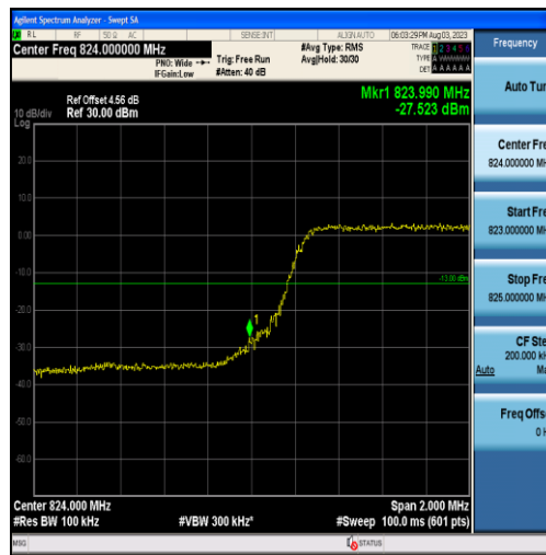
Band5-5MHz-16QAM-20425-25RB#0
