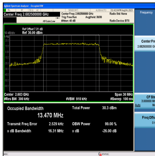
Band41-15MHz-QPSK-41515-75RB#0-13.470
