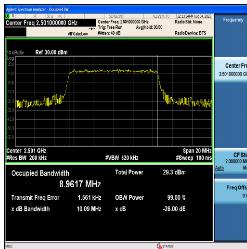
Band41-10MHz-16QAM-39700-50RB#0-8.9617
