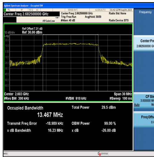
Band41-15MHz-16QAM-41515-75RB#0-13.467
