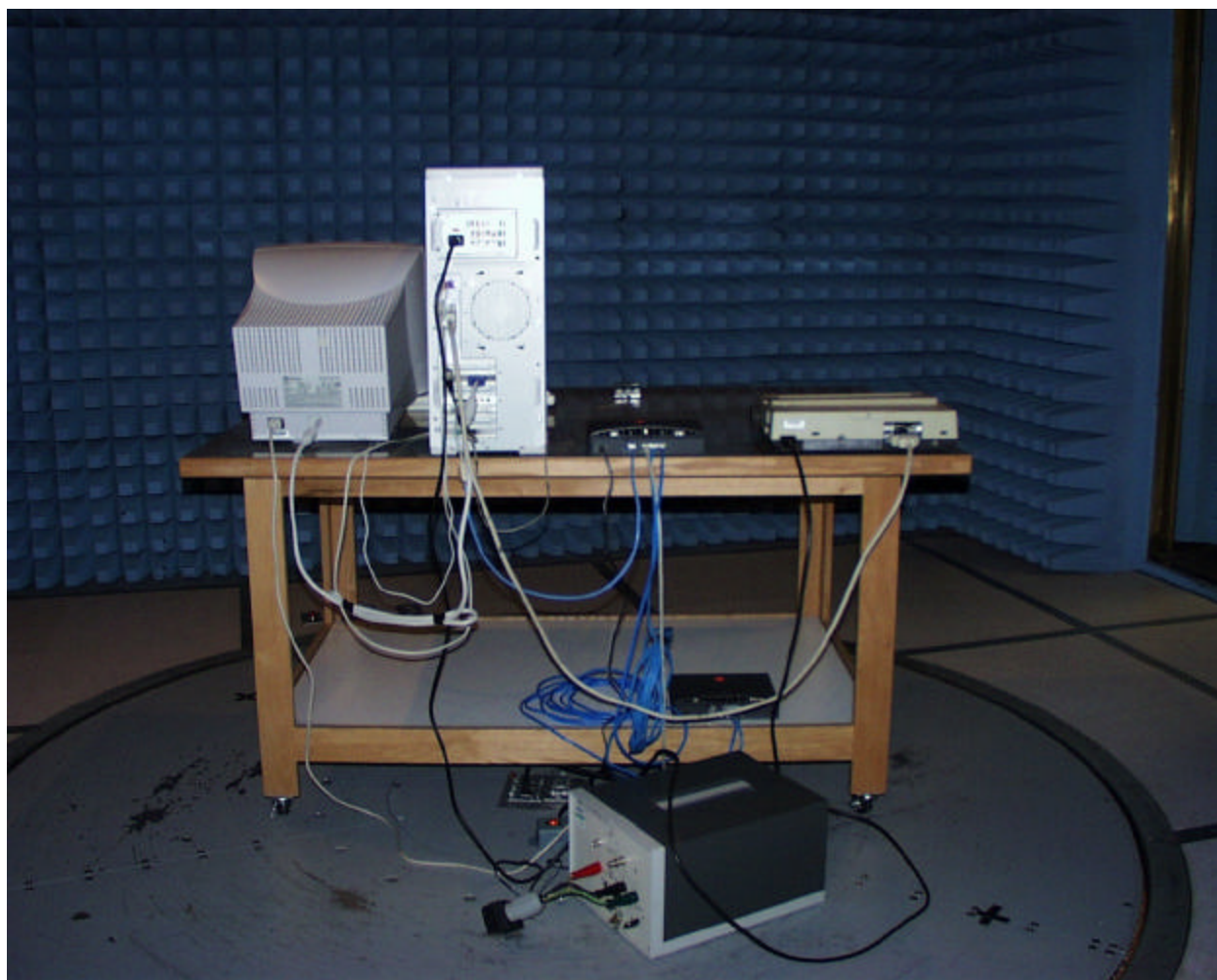
Back view worst case radiated emissions
