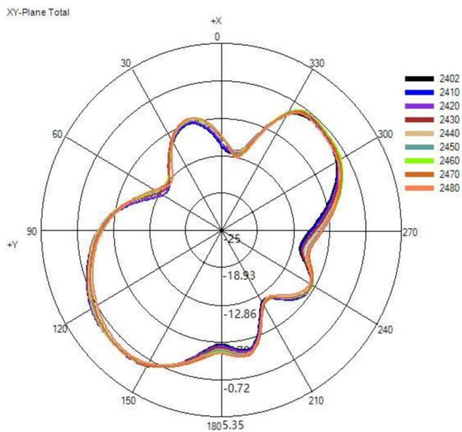
(3) X-Y (Unit: dBi):
