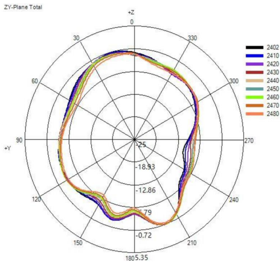
(2) Y-Z (Unit: dBi):
