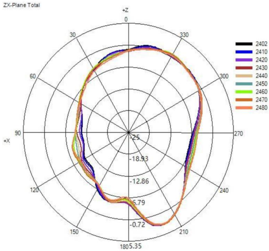
(1) X-Z (Unit : dBi):
