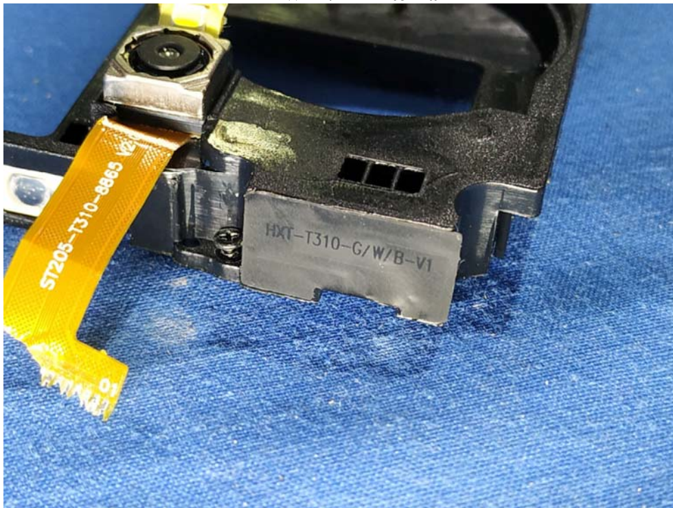
WIFI/BT Antenna
