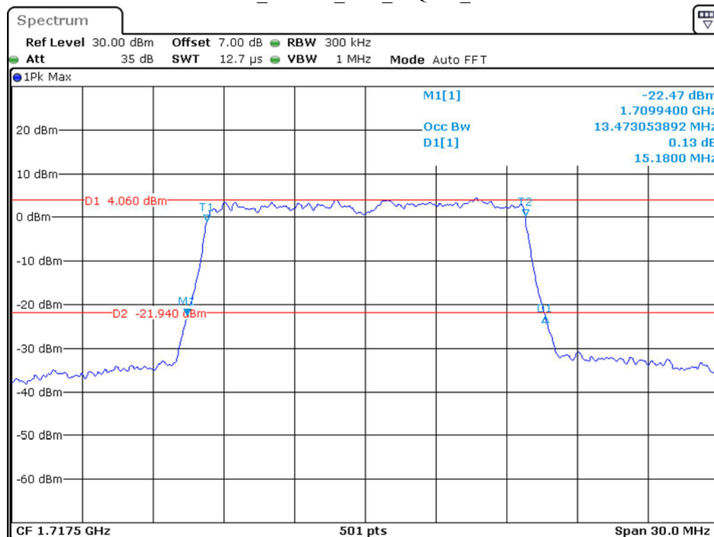
Band 66 15 MHz Low 16QAM RB75#0
