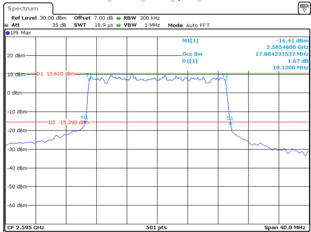
Band 41_20 MHz_Middle_QPSK_RB100#0
