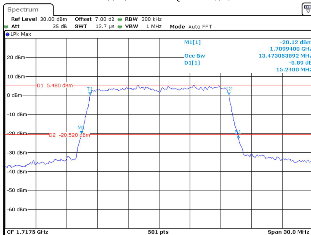
Band 66 15 MHz Low QPSK RB75#0
