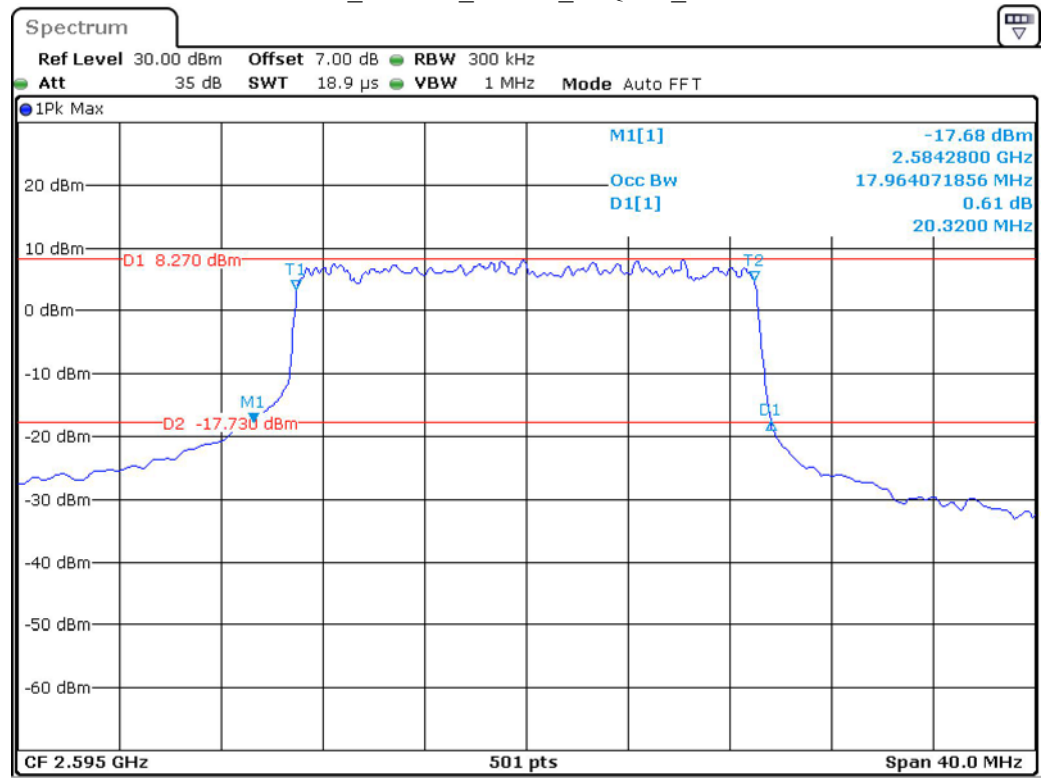
Band 41_20 MHz_Middle_16QAM_RB100#0
