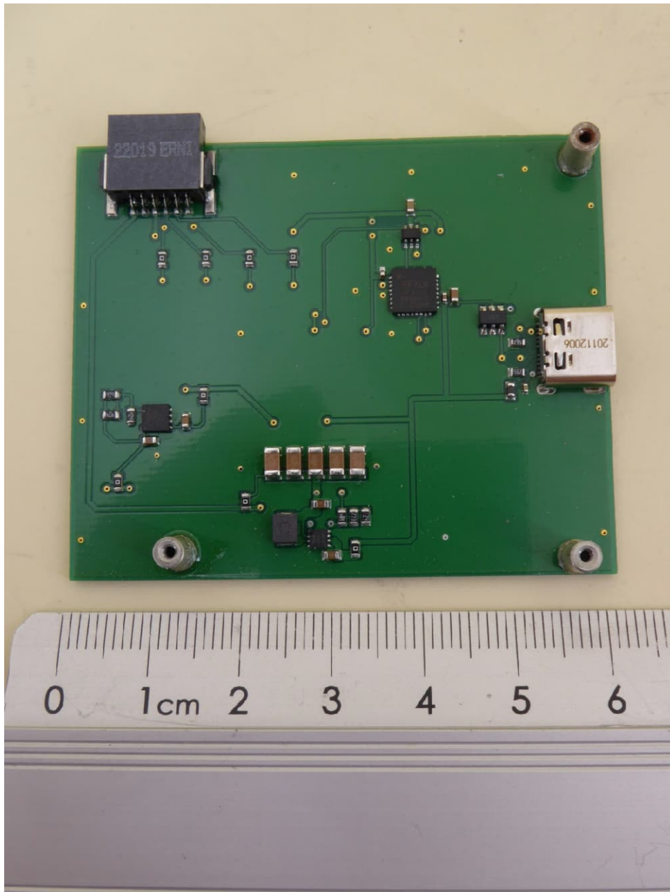
Demo board, top view
