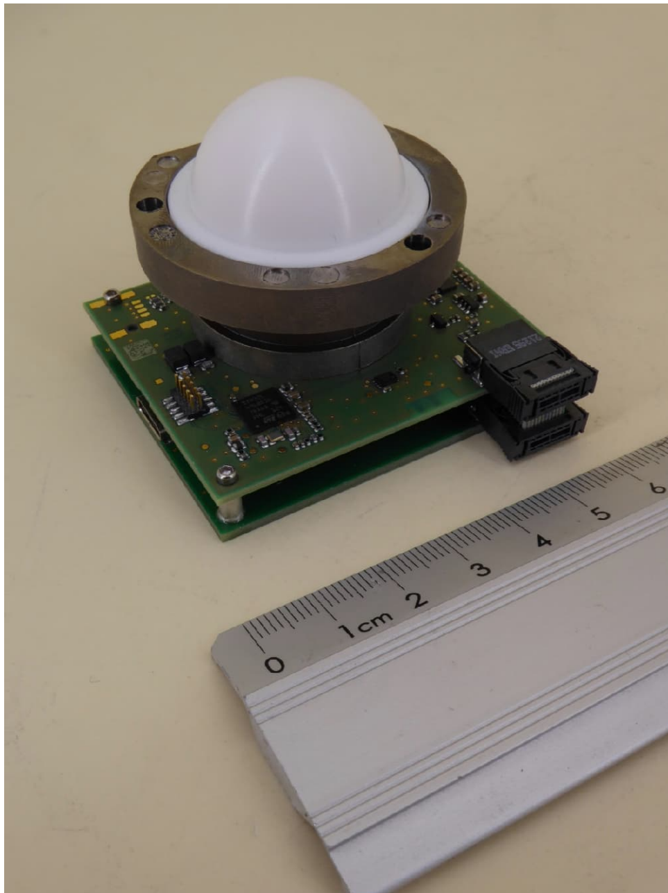
EUT mounted on demo board, 3-D-view 1
