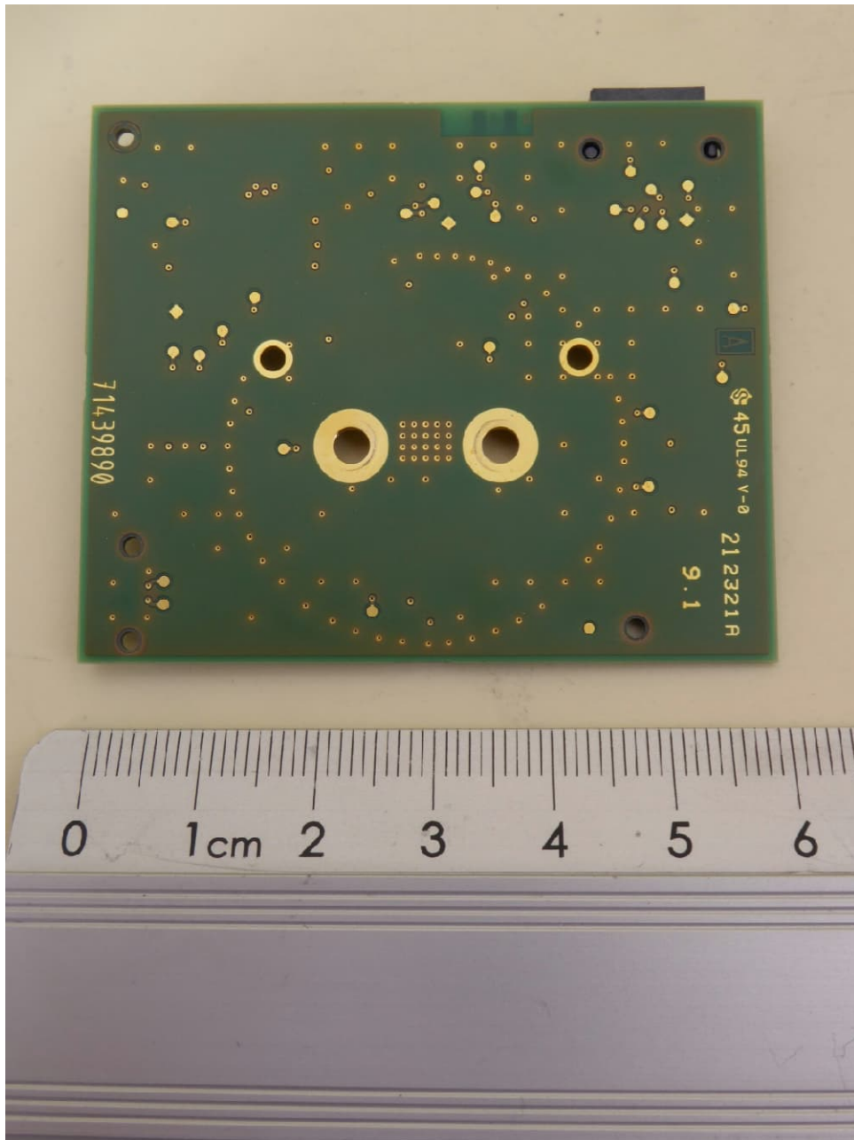
EUT, PCB, bottom view
