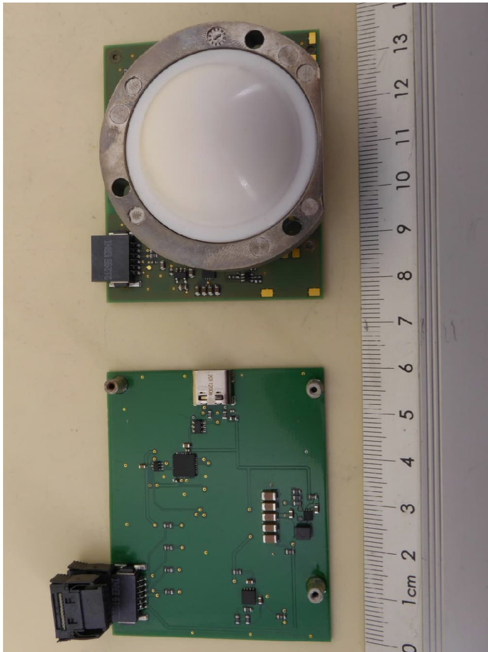
EUT removed from demo board
