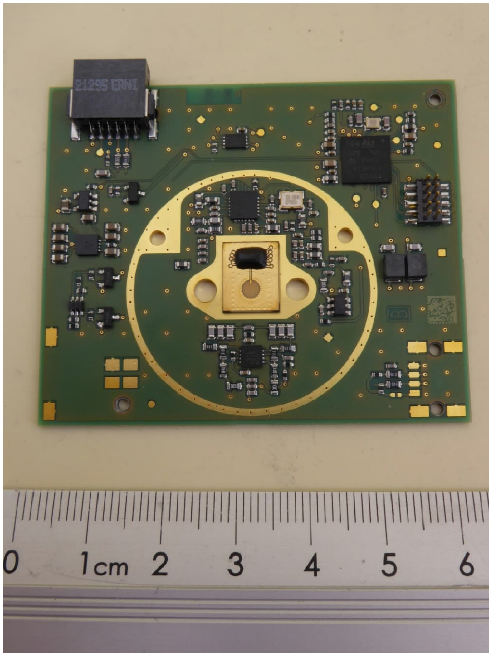
EUT, PCB, top view
