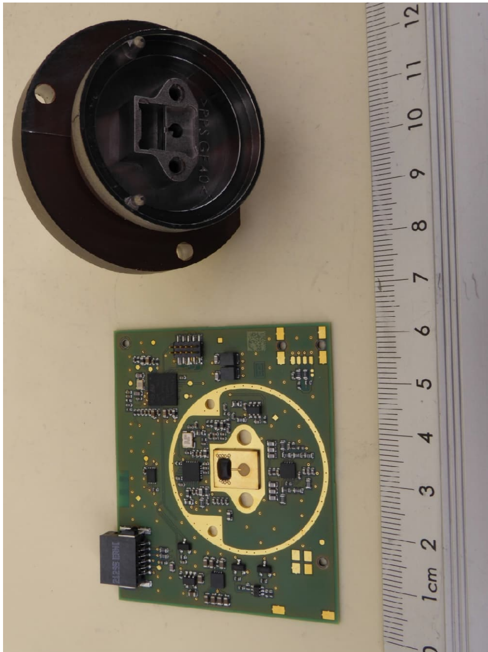
EUT, radom removed view
