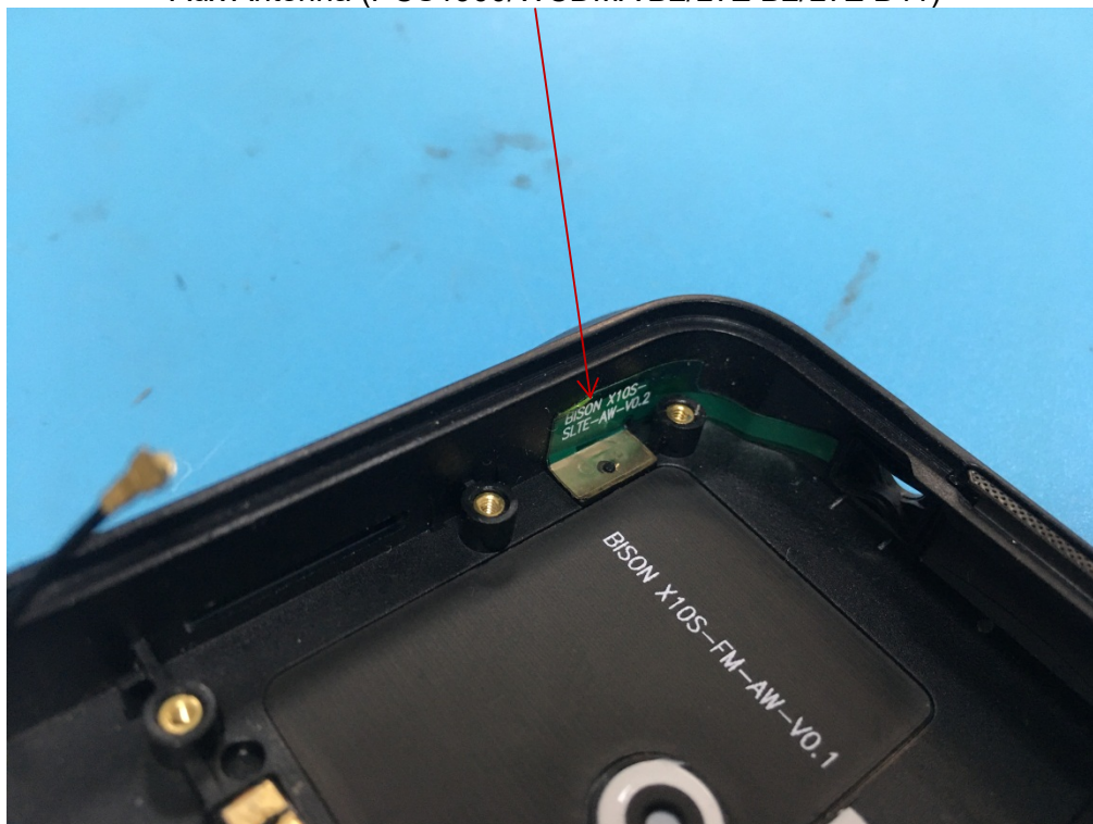
Aux Antenna (PCS1900/WCDMA B2/LTE B2/LTE B41)
