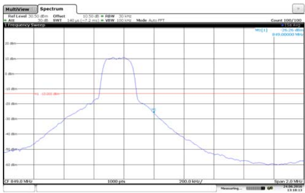
Channel High-1RB#
