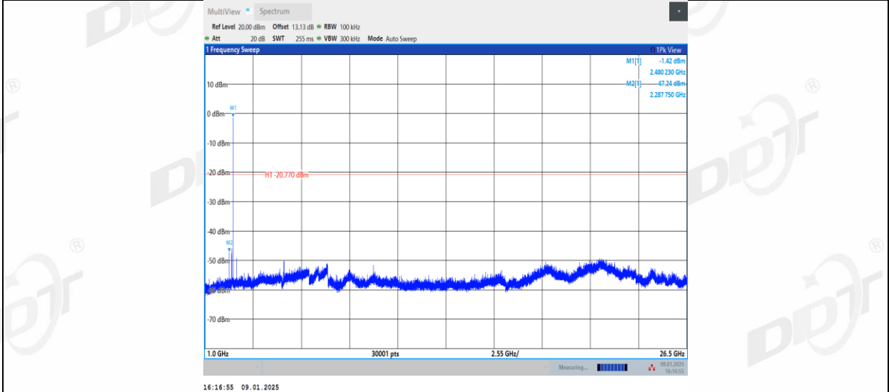
2DH5_Right side_2480_0~Reference
