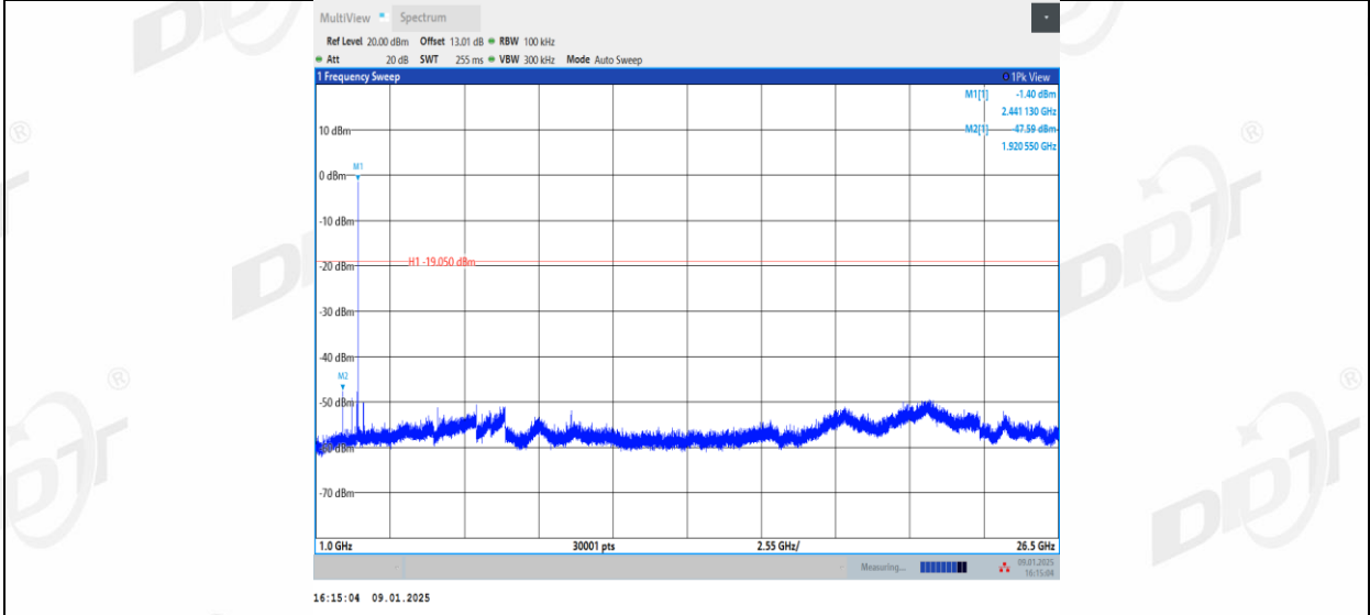
2DH5_Right side_2441_0~Reference
