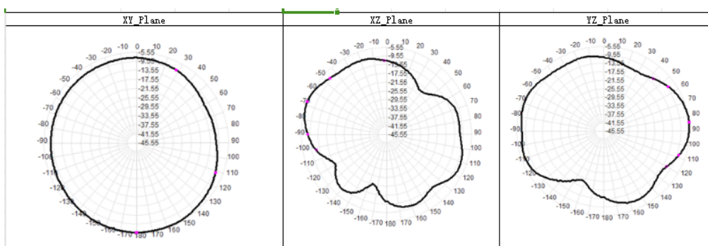
2D Radiation Pattern
