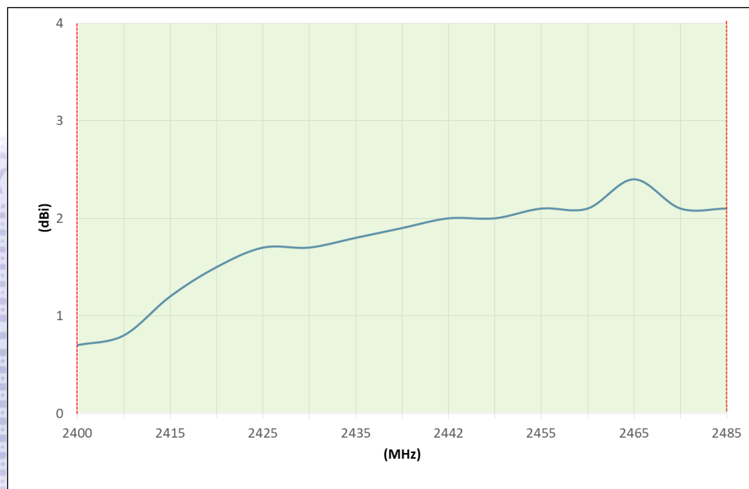
d) Peak Gain (dBi)
