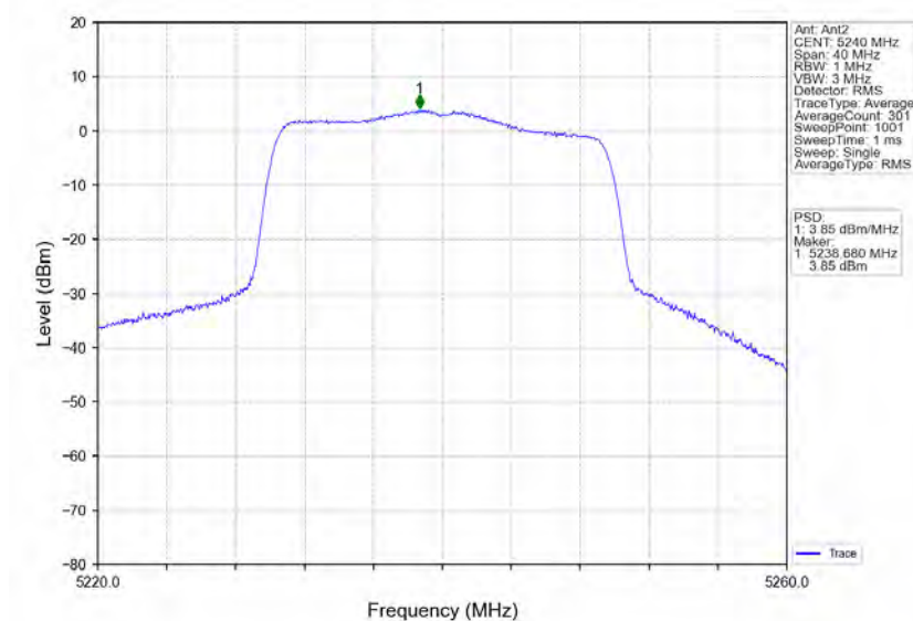
802.11ax(HEW20)_HCH_5240MHz_RU242_Left_Ant2_NTNV
