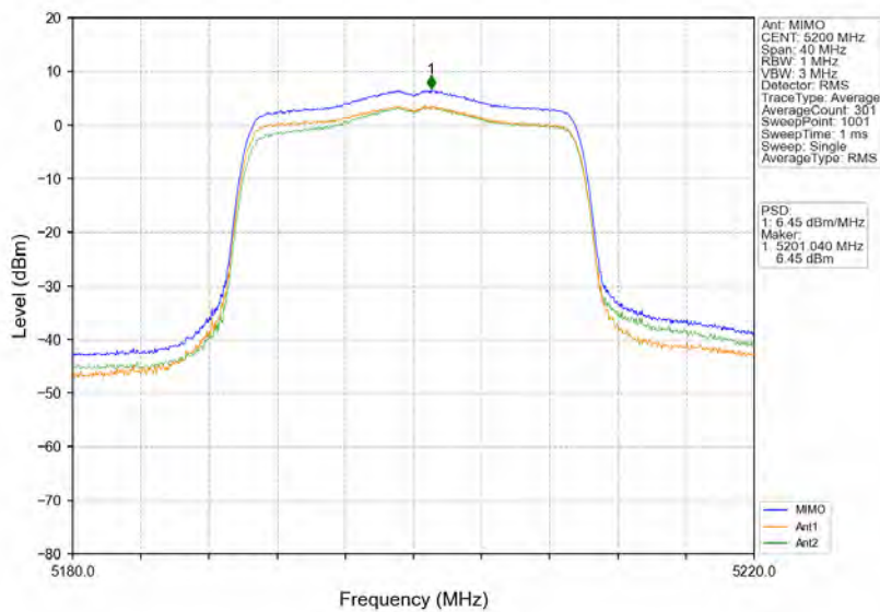
802.11ax(HEW20)_MCH_5200MHz_RU242_Left_MIMO_NTNV
