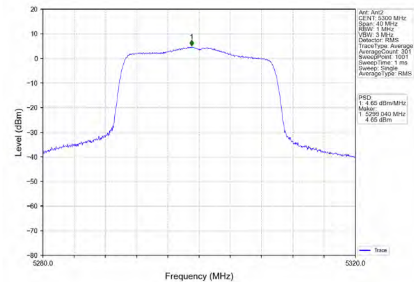
802.11ax(HEW20)_MCH_5300MHz_RU242_Left_Ant2_NTNV
