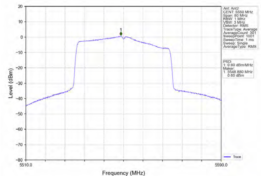
802.11ax(HEW40)_MCH_5550MHz_RU484_Left_Ant2_NTNV
