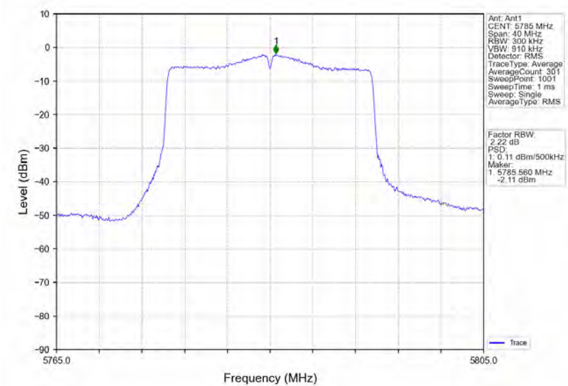
802.11ax(HEW20)_MCH_5785MHz_RU242_Left_Ant1_NTNV
