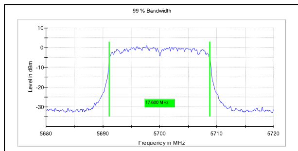
Channel Frequency:5700MHz
