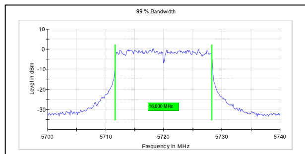
Channel Frequency:5720MHz
