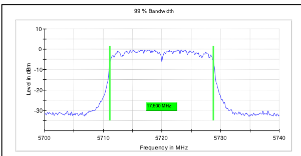
Channel Frequency:5720MHz
