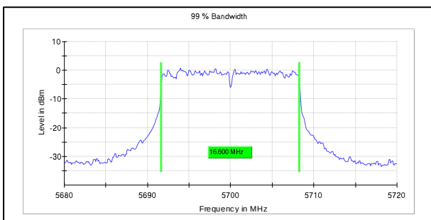
Channel Frequency:5700MHz
