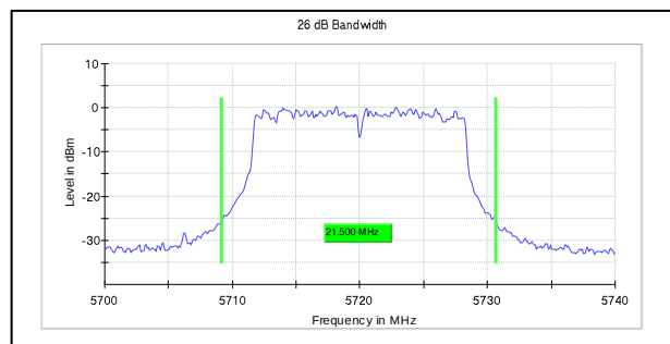
Channel Frequency:5720MHz
