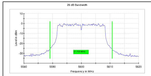
Channel Frequency:5600MHz
