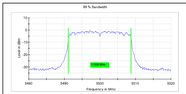
Channel Frequency:5500MHz
