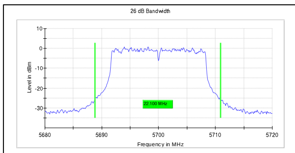
Channel Frequency:5700MHz
