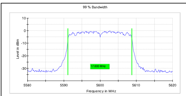
Channel Frequency:5600MHz
