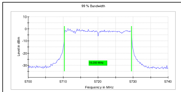
Channel Frequency:5720MHz
