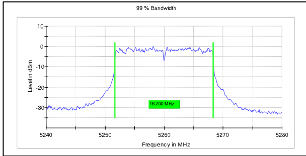
Channel Frequency:5260MHz
