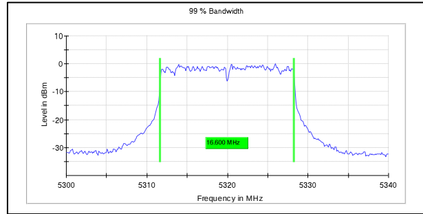
Channel Frequency:5320MHz
