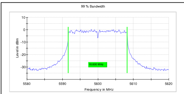
Channel Frequency:5600MHz
