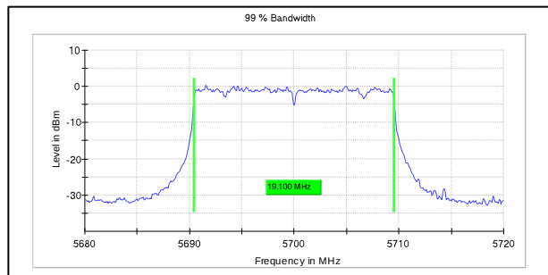
Channel Frequency:5700MHz
