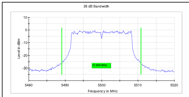
Channel Frequency:5500MHz
