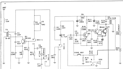
CIRCUIT DIAGRAM (RECEIVER)
