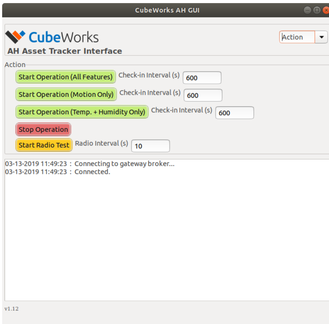
Figure 1. Main page of the GUI
