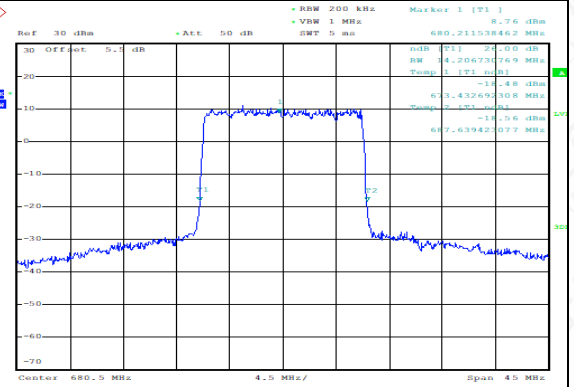
FDD71_MidRange_15MHz_680.5MHz_QPSK
