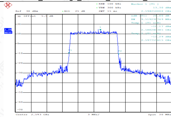
TDD41_MidRange_10MHz_2593MHz_QPSK
