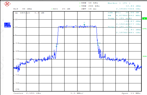
TDD38_MidRange_5MHz_2595MHz_QPSK
