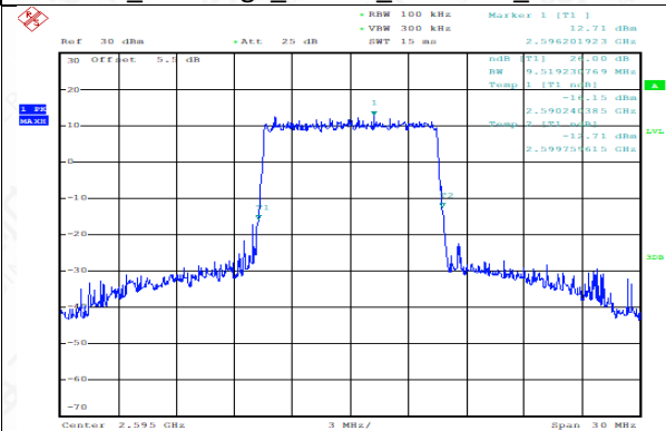
TDD38_MidRange_10MHz_2595MHz_16QAM
