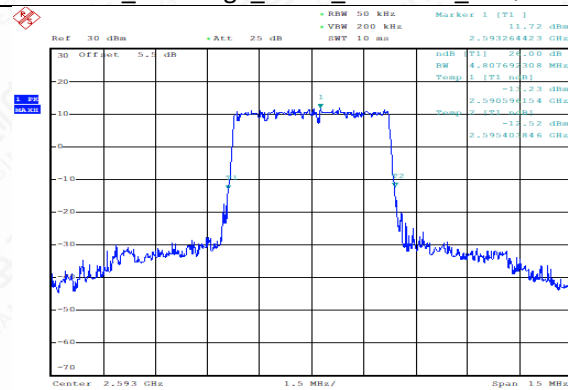
TDD41_MidRange_5MHz_2593MHz_16QAM
