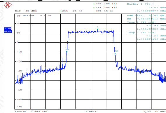
TDD38_MidRange_10MHz_2595MHz_QPSK
