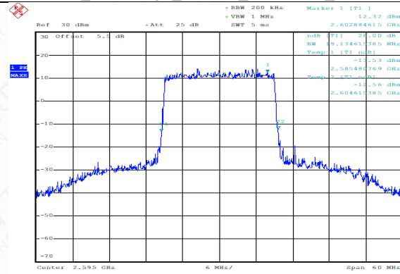
TDD38_MidRange_20MHz_2595MHz_64QAM
