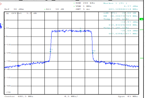
FDD71_MidRange_15MHz_680.5MHz_64QAM
