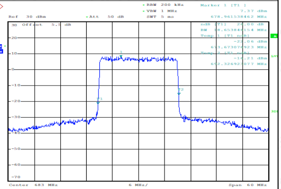
FDD71_MidRange_20MHz_683MHz_16QAM
