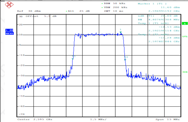
TDD38_MidRange_5MHz_2595MHz_64QAM
