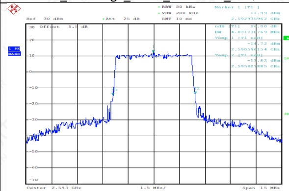
TDD41_MidRange_5MHz_2593MHz_64QAM
