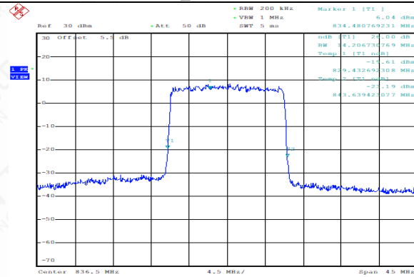
FDD26_22_MidRange_15MHz_836.5MHz_64QAM
