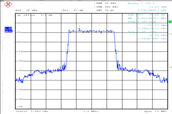
TDD41_MidRange_5MHz_2593MHz_QPSK
