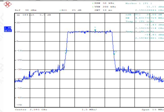
TDD38_MidRange_5MHz_2595MHz_16QAM
