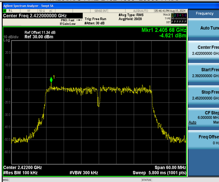
11N40SISO-Ant2-2422-0~Reference-PASS
