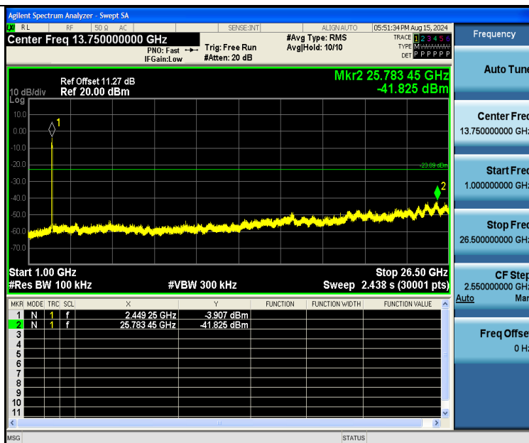
11N40SISO-Ant2-2437-1000~26500-PASS
