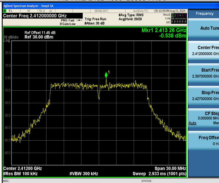
11G-Ant2-2412-0~Reference-PASS
