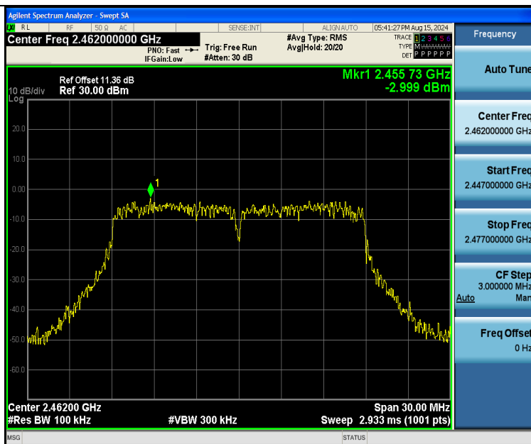
11N20SISO-Ant2-2462-0~Reference-PASS
